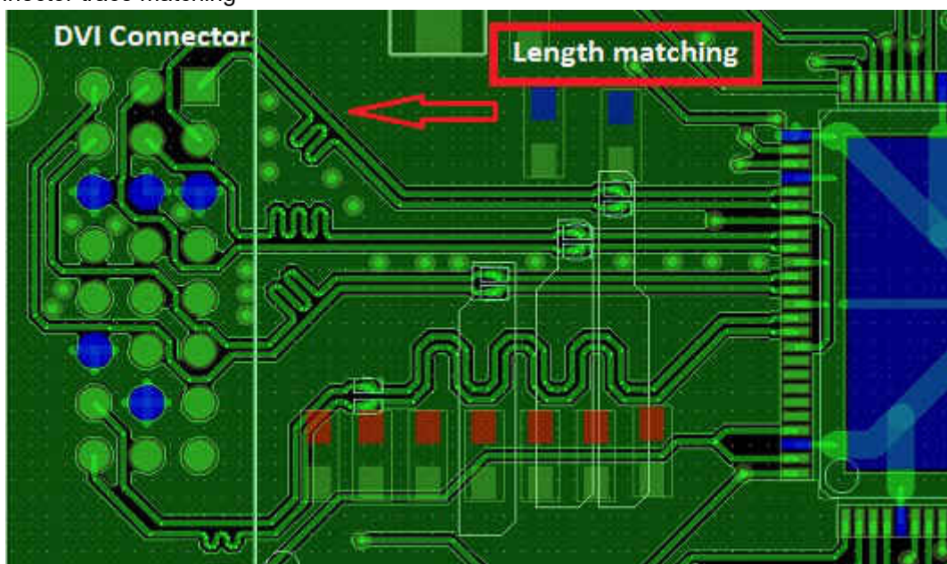
Figure 8-8. DVI Connector
