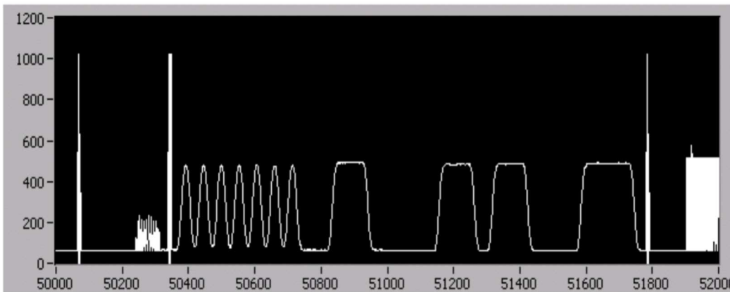
Figure 5. Line 21 Closed Caption ITU-R BT.656 Digital Output Capture in Raw Data Mode UV (chroma) data are replaced with Y (luma) data
