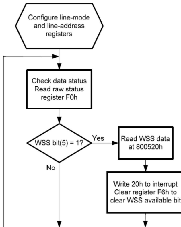
Figure 3. Example WSS/CGMS Data Retrieval
