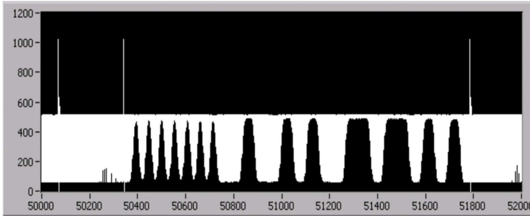
Figure 4. Line 21 Closed Caption ITU-R BT.656 Digital Output Capture with YUV Samples Present Raw Data Mode is disabled
