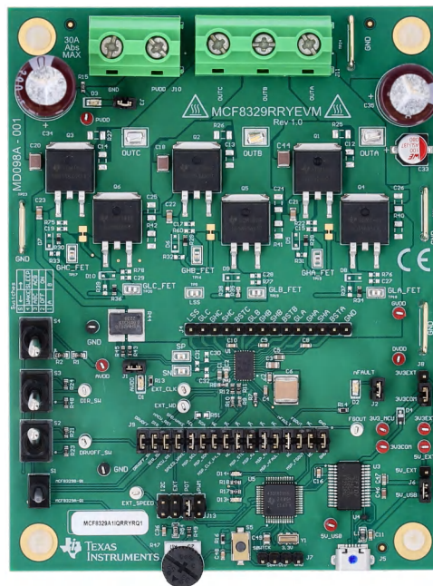
MCF8329RRYEVM (Top View)
