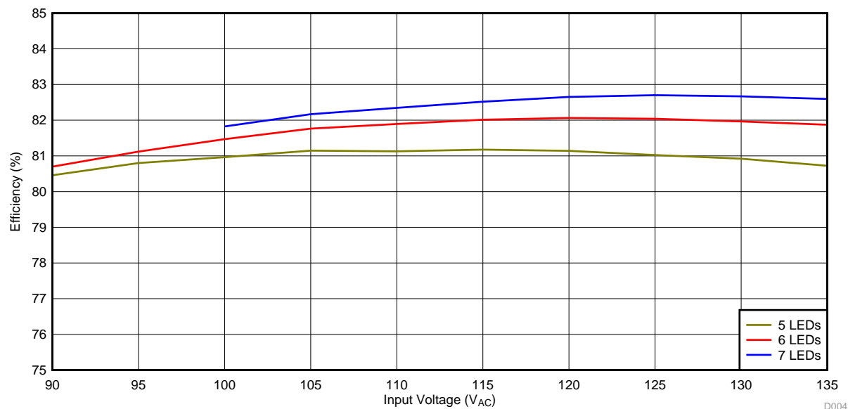
Figure 6. LM3445EVM-695 Efficiency
