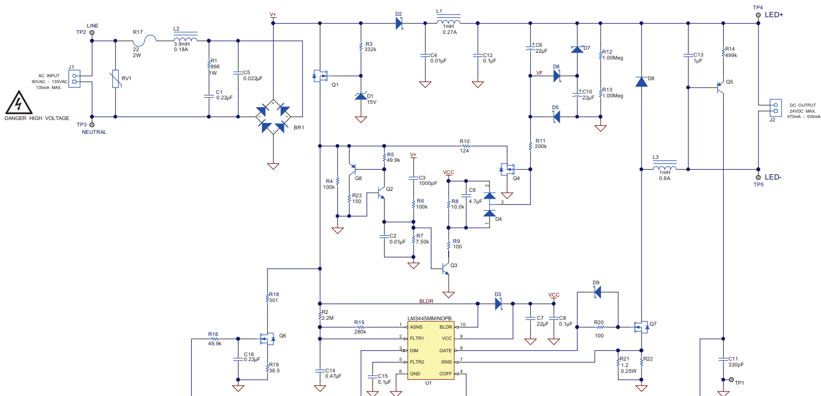
Figure 1. LM3445EVM-695 Schematic
