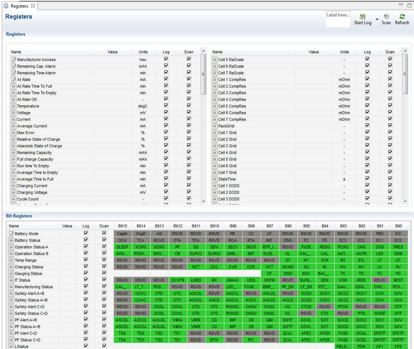
Figure 2-2. Registers Screen
