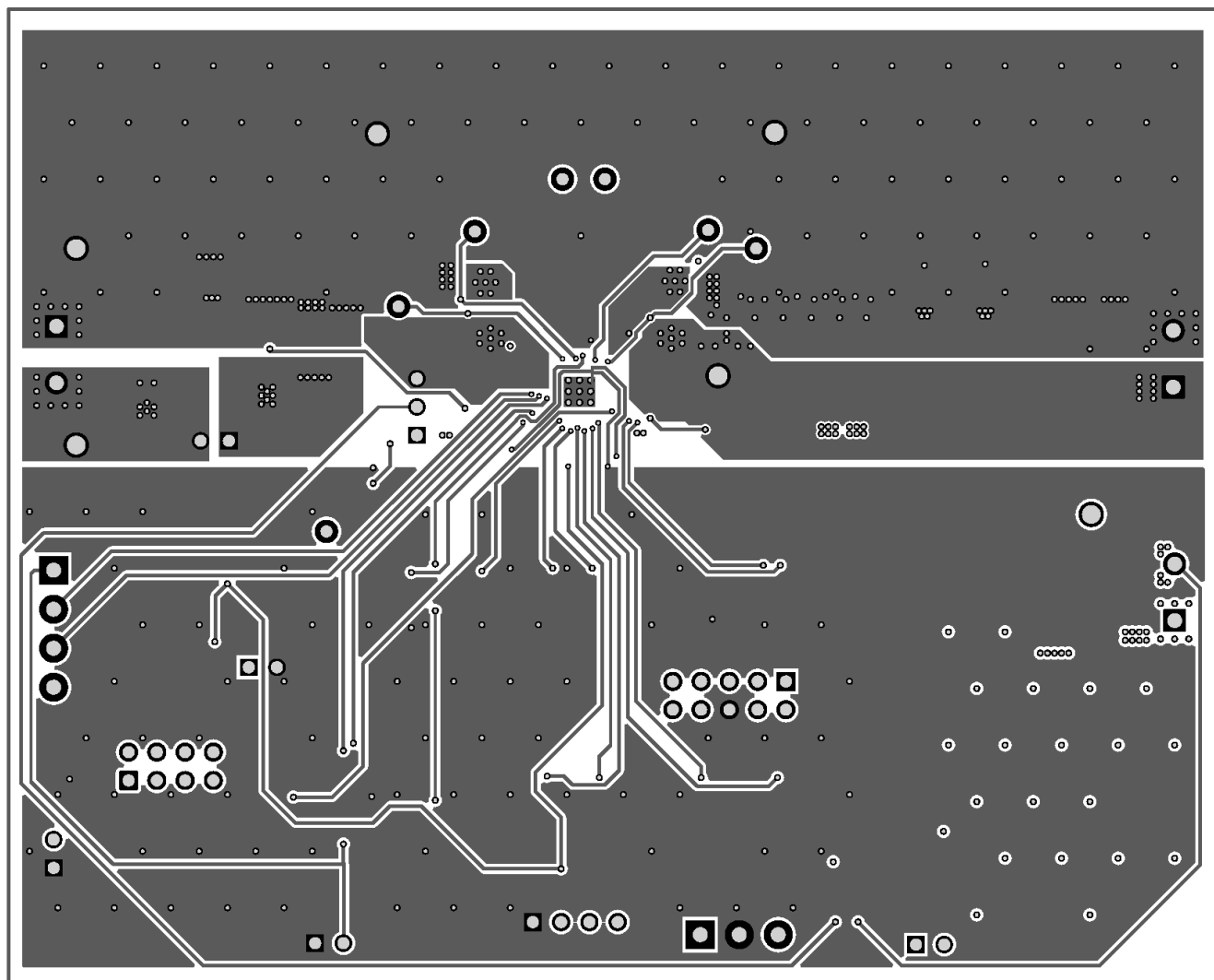
Figure 3-5. PCB Layer 3
