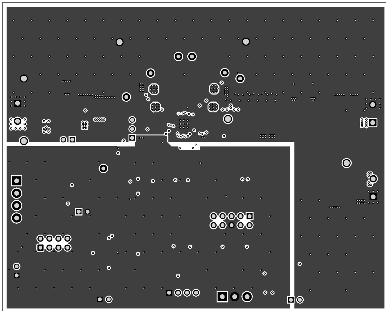
Figure 3-4. PCB Layer 2
