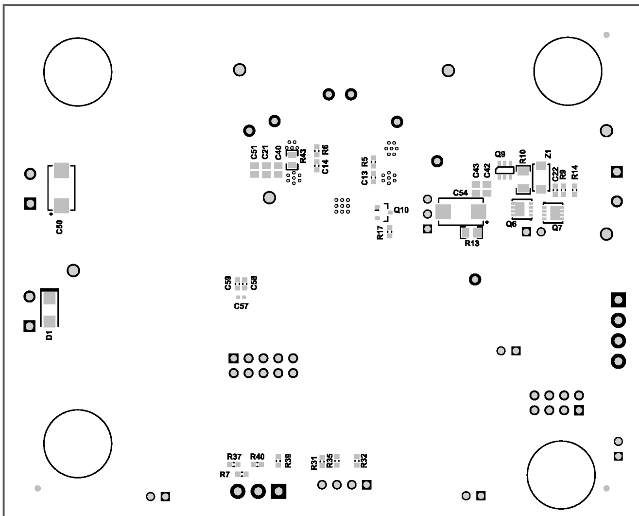
Figure 3-2. Bottom Assembly
