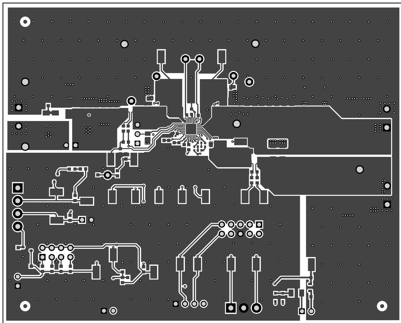
Figure 3-3. PCB Layer 1
