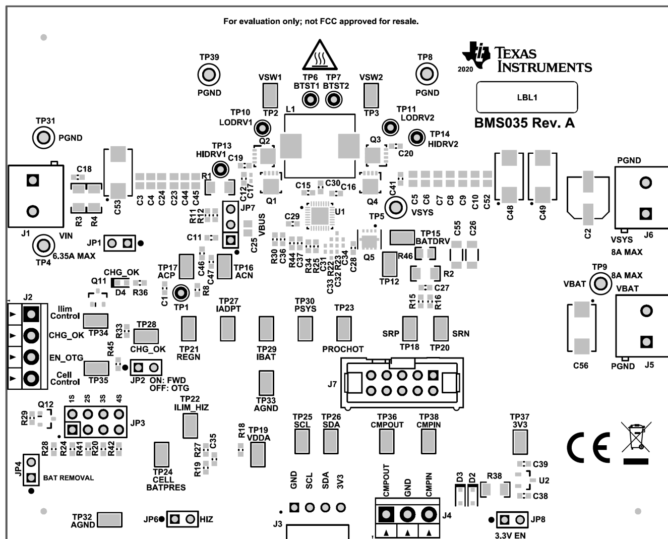
Figure 3-1. Top Assembly
