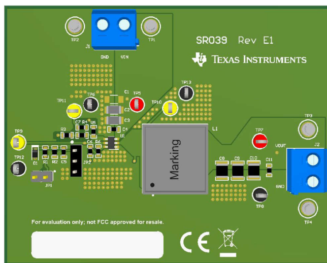
Figure 2-1. TPS542021EVM Connectors and Jumpers Placement
