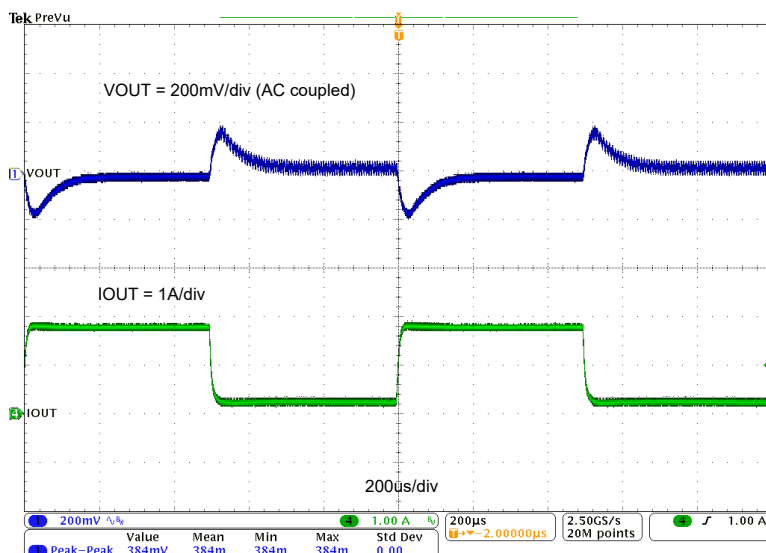
Figure 3-2. TPS542021EVM Load Transient Response, 0.2A to 1.8A Load Step
