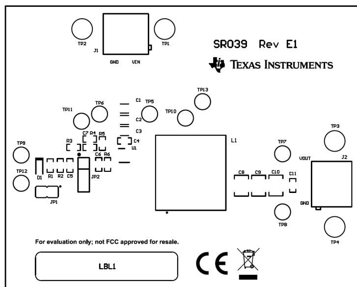
Figure 4-2. TPS542021EVM Top Assembly
