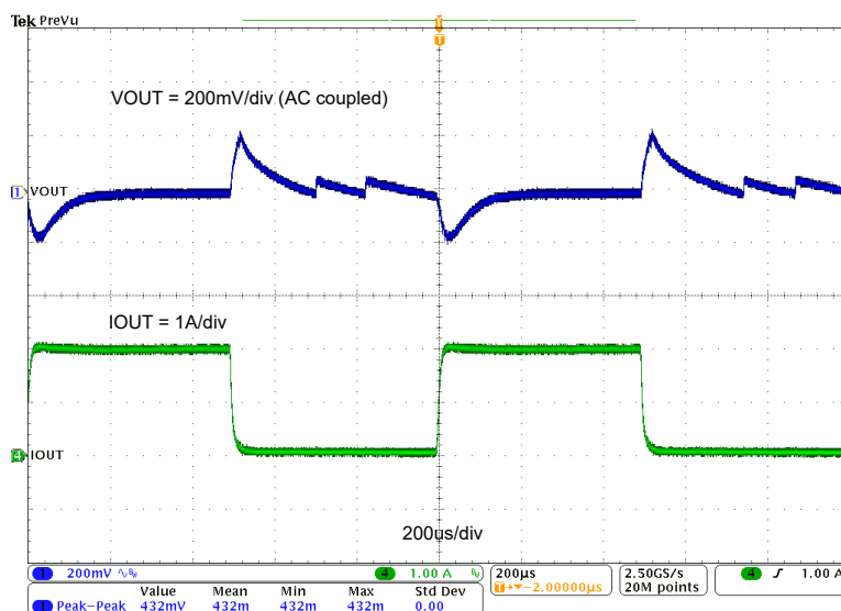
Figure 3-1. TPS542021EVM Load Transient Response, 0A to 2A Load Step
