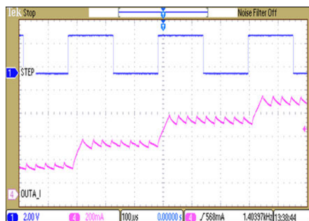
Figure 3-2. Microstepping Current vs STEP Input, Slow Decay
