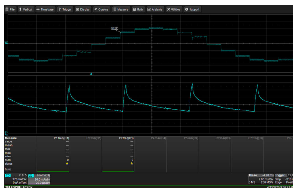
Figure 3-15. PWM at 92% Level (decreasing), PWM Frequency is 25kHz
