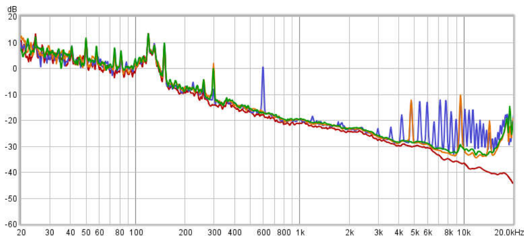
Figure 3-21. SPL Plots at Various Microstepping Levels
