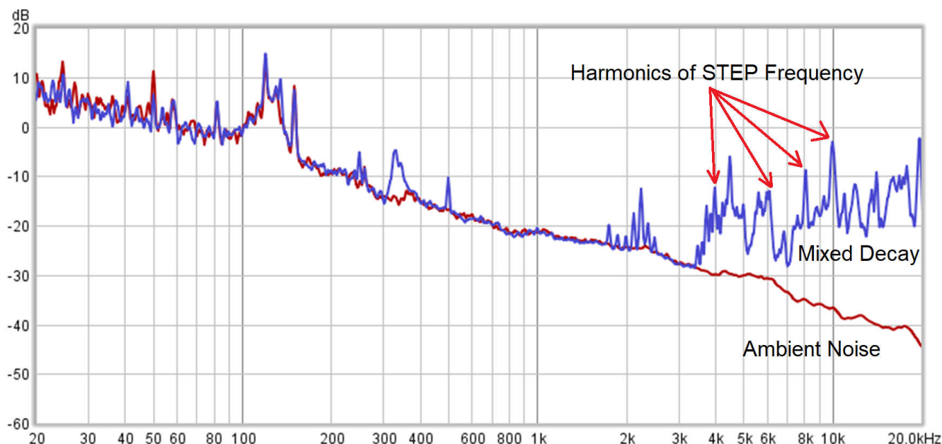
Figure 3-20. SPL Plot for 1/4 Microstepping, Mixed Decay, Step Frequency = 2000 pps (pulses per second)
