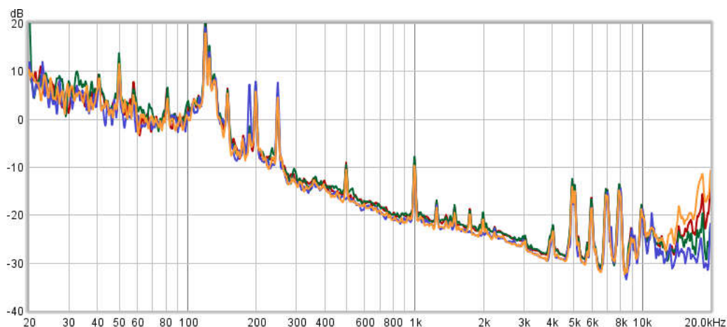
Figure 3-8. Effects of Changing Current Ripple
