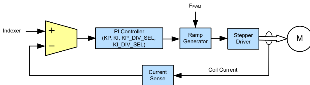
Figure 3-9. Silent Step Block Diagram
