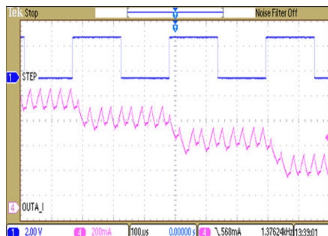
Figure 3-3. Microstepping Current vs STEP Input, Mixed Decay
