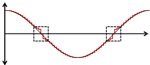
Figure 3-16. Current Distortion Due to High Blanking Time
