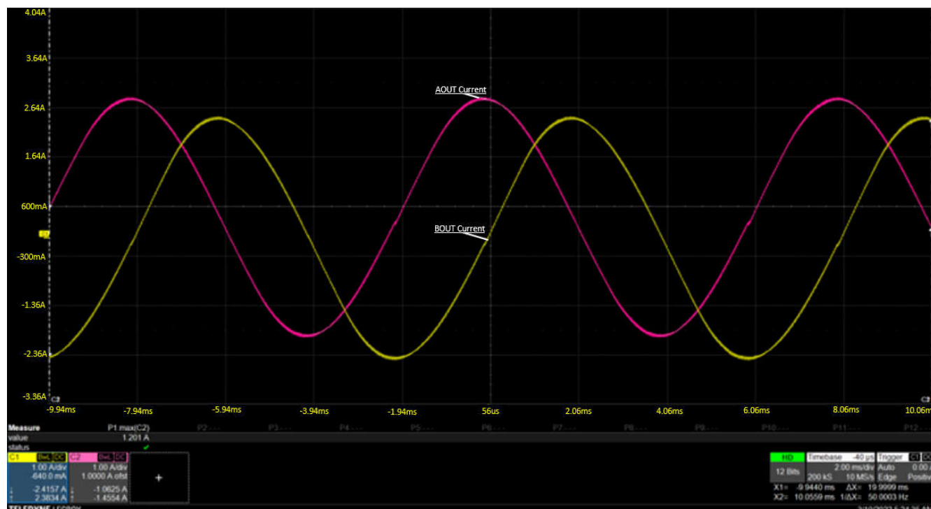
Figure 3-10. Coil Current Waveform with Silent Step Decay
