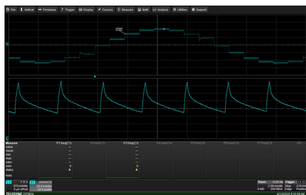
Figure 3-14. PWM at 100% Level, PWM Frequency is 35kHz
