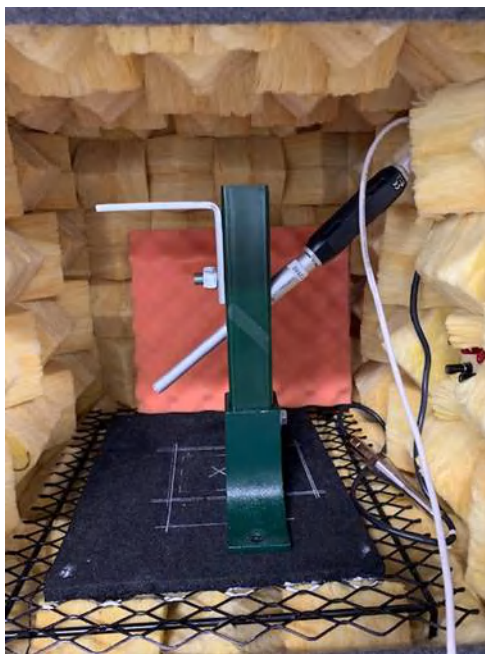
Figure 2-1. Audible Noise Measurement Setup
