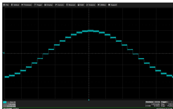
Figure 3-22. Current Waveform With 1/8 Microstepping, Smart Tune Ripple Control
