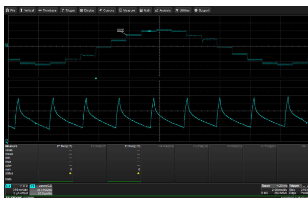
Figure 3-13. PWM at 92% Level (increasing), PWM Frequency is 44kHz
