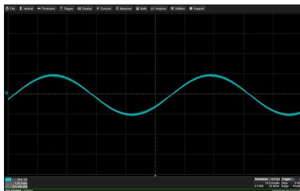
Figure 3-19. Smoothness of Zero-Cross at 1/64 Microstepping
