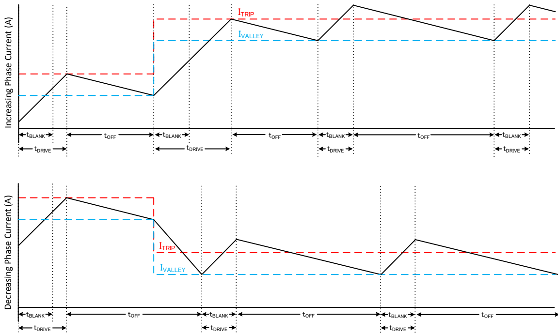
Figure 3-6. Smart tune Ripple Control Decay Mode
