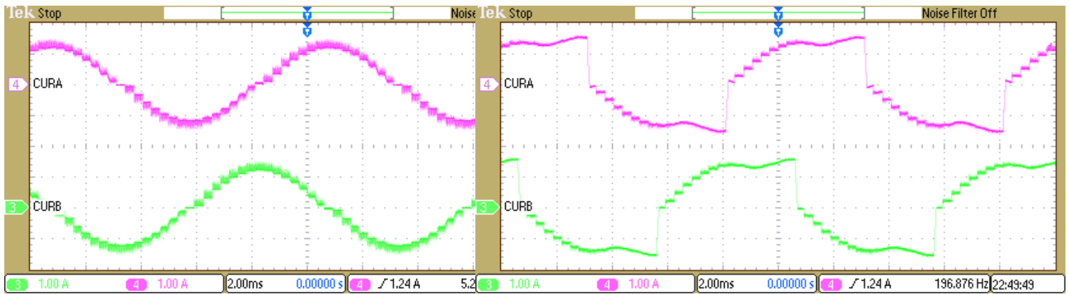
Figure 3-4. 30% Mixed Decay on Increasing and Decreasing Steps
