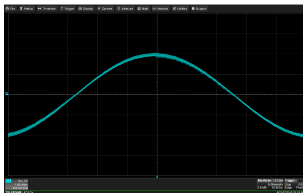
Figure 3-23. Current Waveform With 1/256 Microstepping, Smart Tune Ripple Control
