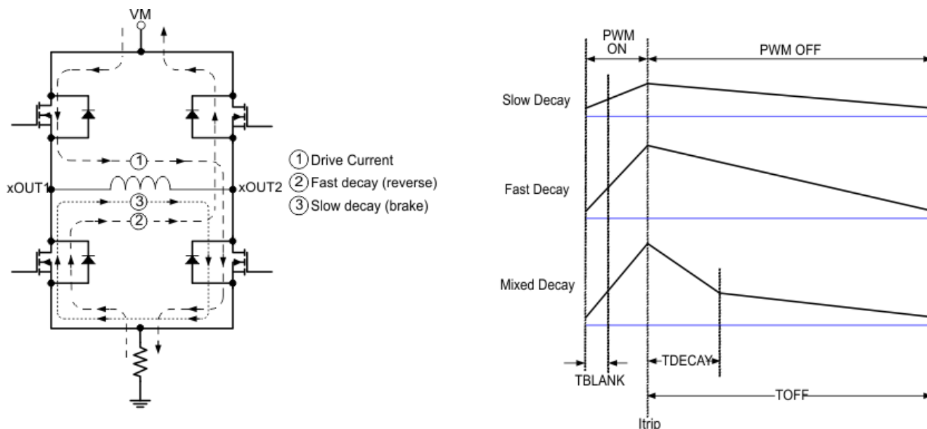
Figure 1-2. Decay Modes
