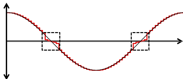
Figure 3-17. Current Distortion Due to High OFF Time
