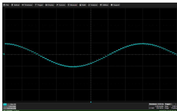
Figure 3-18. Smoothness of Zero-Cross at 1/16 Microstepping
