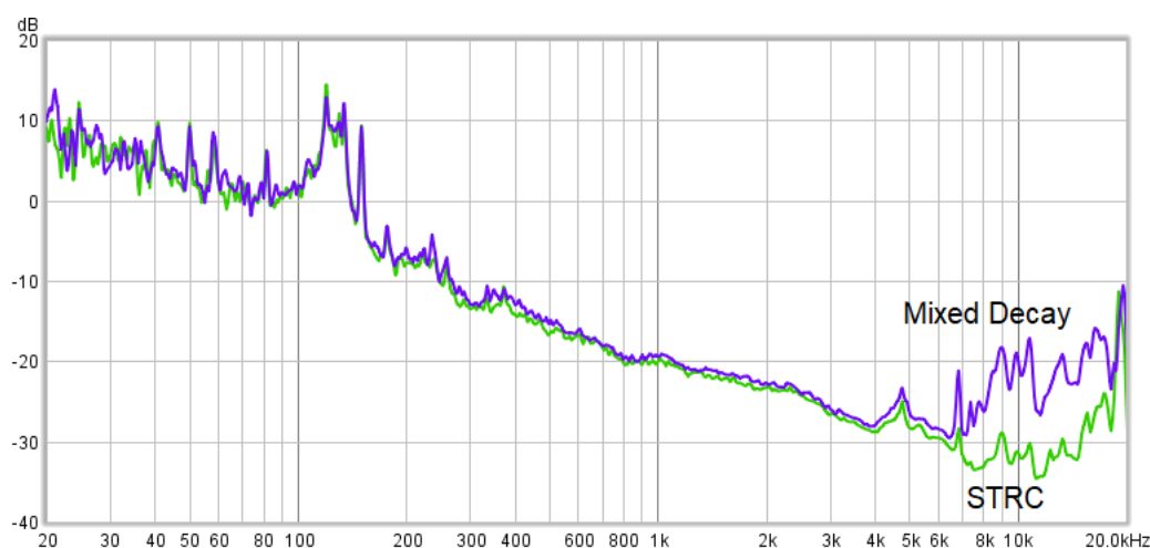
Figure 3-7. Mixed Decay vs Smart Tune Ripple Control (STRC) at 1/256 Microstepping
