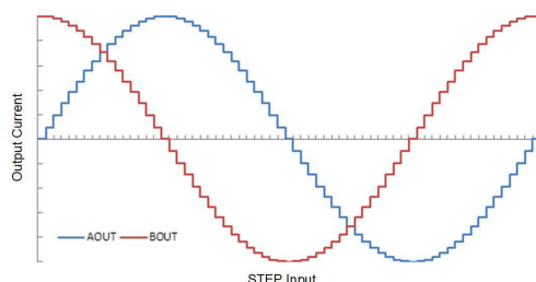
Figure 1-1. Microstepping Current Waveform
