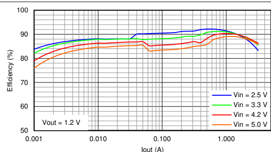
Figure 9-3. Efficiency
