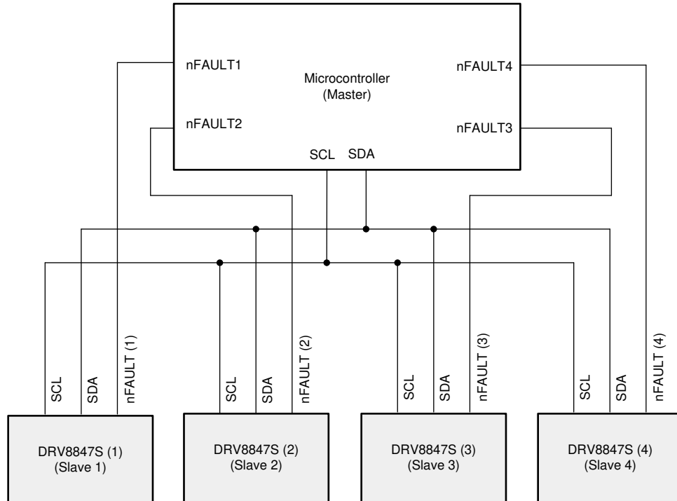
Figure 7-25. Multi-Slave Operation of DRV8847S
