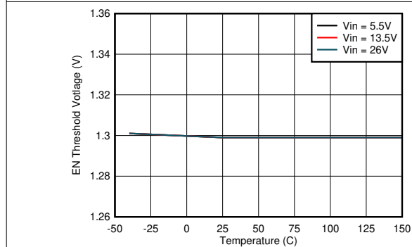
Figure 8-3. Precision Device Enable Threshold
