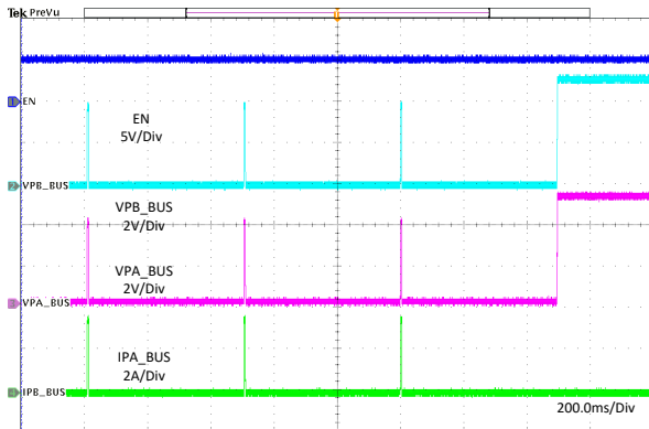
Figure 11-25. 1-Ω Load Recovery
