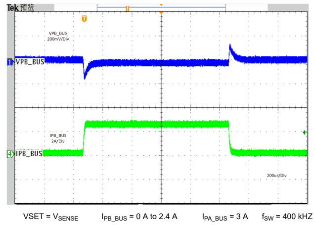
Figure 11-8. Load Transient Without Cable Compensation
