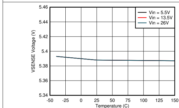
Figure 8-5. V_{SENSE} Voltage vs Junction Temperature
