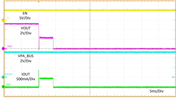
Figure 11-28. OUT short to 5.1-Ω Load
