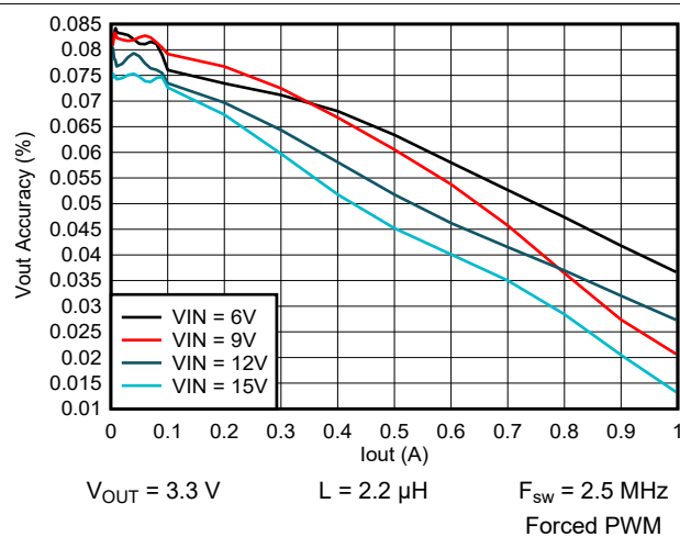
Figure 9-19. Output Voltage vs Output Current
