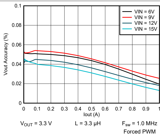
Figure 9-25. Output Voltage vs Output Current
