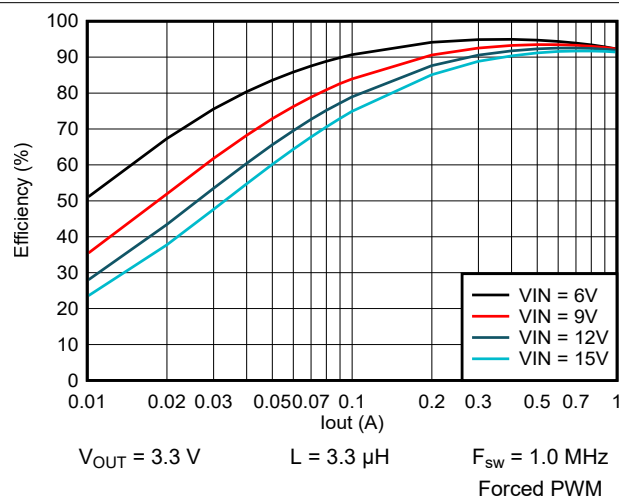
Figure 9-21. Efficiency vs Output Current
