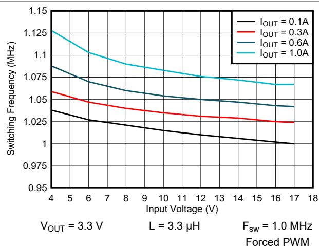
Figure 9-23. Switching Frequency vs Input Voltage
