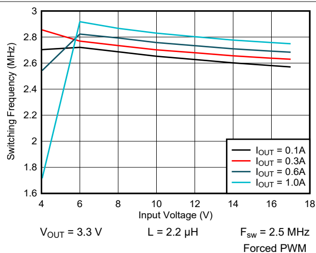
Figure 9-17. Switching Frequency vs Input Voltage
