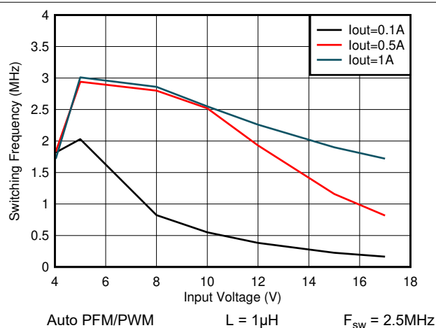
Figure 7-29. Switching Frequency vs Input Voltage V_{\text{OUT}} = 3.3\text{V}
