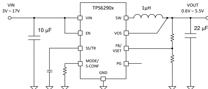
Simplified Schematic
