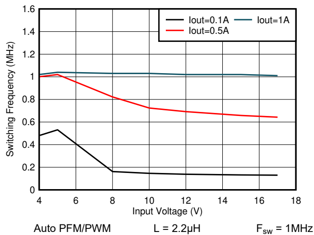
Figure 7-27. Switching Frequency vs Input Voltage V_{\text{OUT}} = 3.3\text{V}
