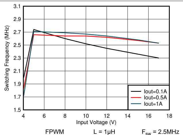
Figure 7-30. Switching Frequency vs Input Voltage V_{\text{OUT}} = 3.3\text{V}
