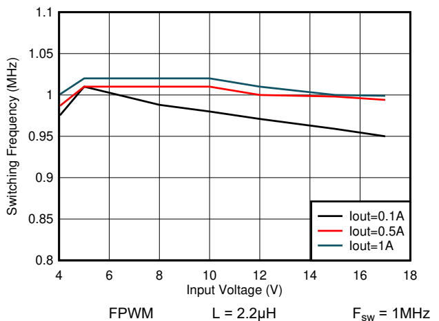
Figure 7-28. Switching Frequency vs Input Voltage V_{\text{OUT}} = 3.3\text{V}
