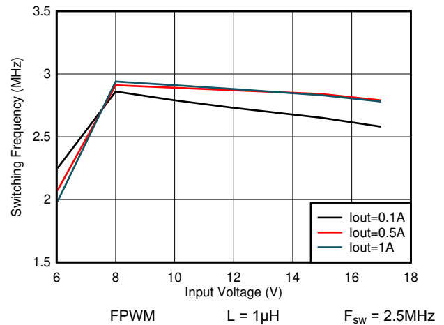
Figure 7-26. Switching Frequency vs Input Voltage V_{\text{OUT}} = 5\text{V}
