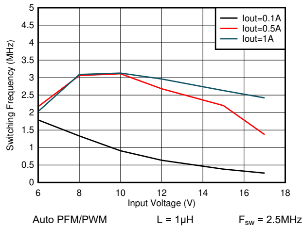
Figure 7-25. Switching Frequency vs Input Voltage V_{\text{OUT}} = 5\text{V}
