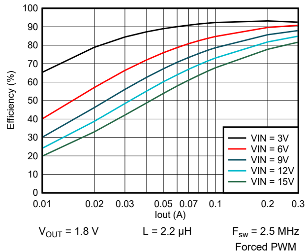
Figure 9-27. Efficiency vs Output Current
