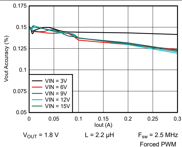
Figure 9-31. Output Voltage vs Output Current
