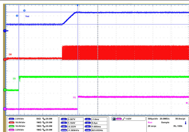
Figure 9-62. Start-Up Timing
