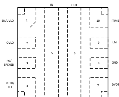
Figure 6-1. TPS25946xx RPW Package 10-Pin QFN Top View
