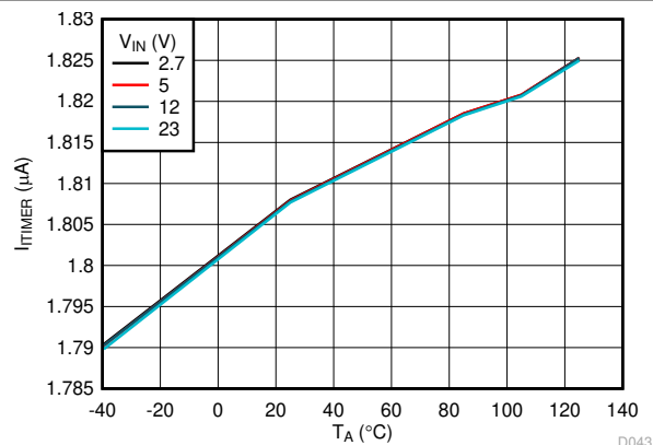
Figure 7-18. ITIMER Discharge Current vs Temperature
