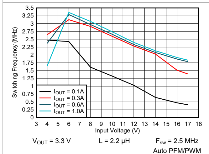
Figure 9-16. Switching Frequency vs Input Voltage
