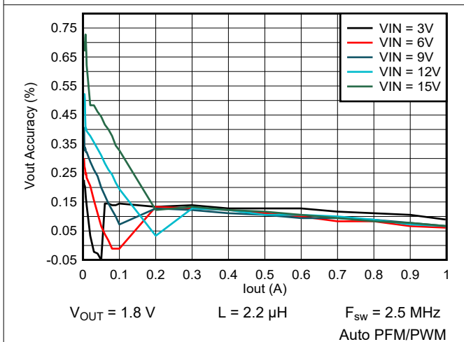
Figure 9-30. Output Voltage vs Output Current
