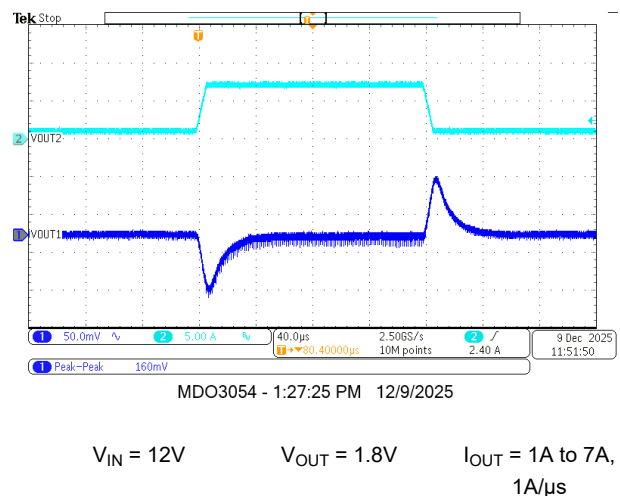
Figure 8-25. VOUT1 Load Transient
