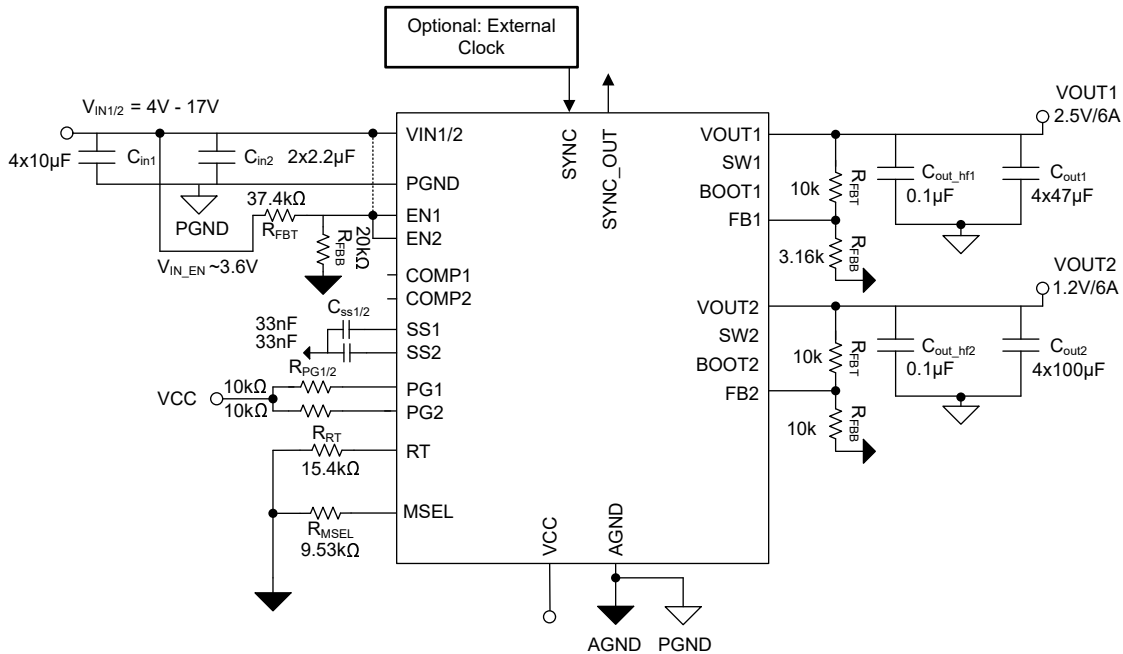
Figure 8-1. Two Output Application Schematic
