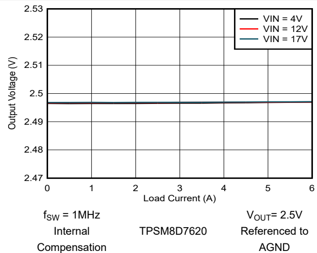
Figure 8-7. Load Regulation
