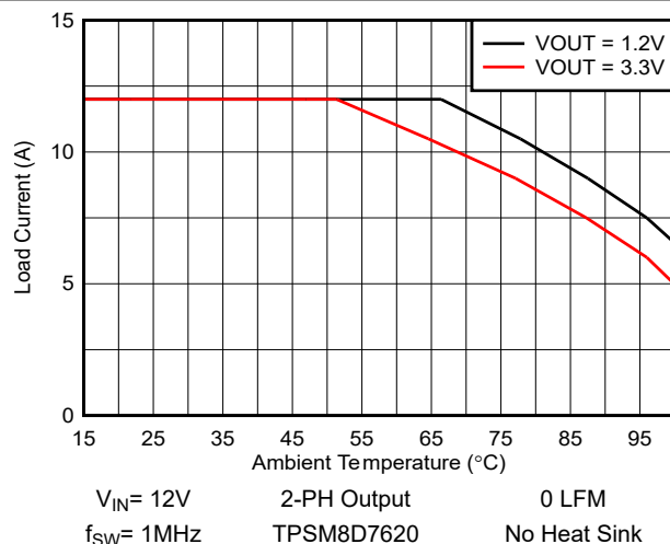
Figure 6-4. Maximum Output Current vs Ambient Temperature
