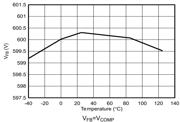
Figure 6-2. V_{FB} vs Temperature
