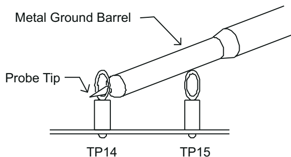
Figure 4-1. Tip and Barrel Measurement for Vout Ripple
