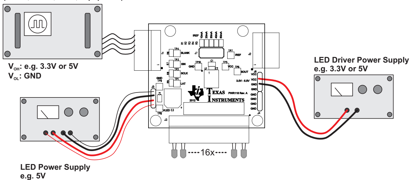
Figure 2. TLC5929 EVM Recommended Test Set-Up
