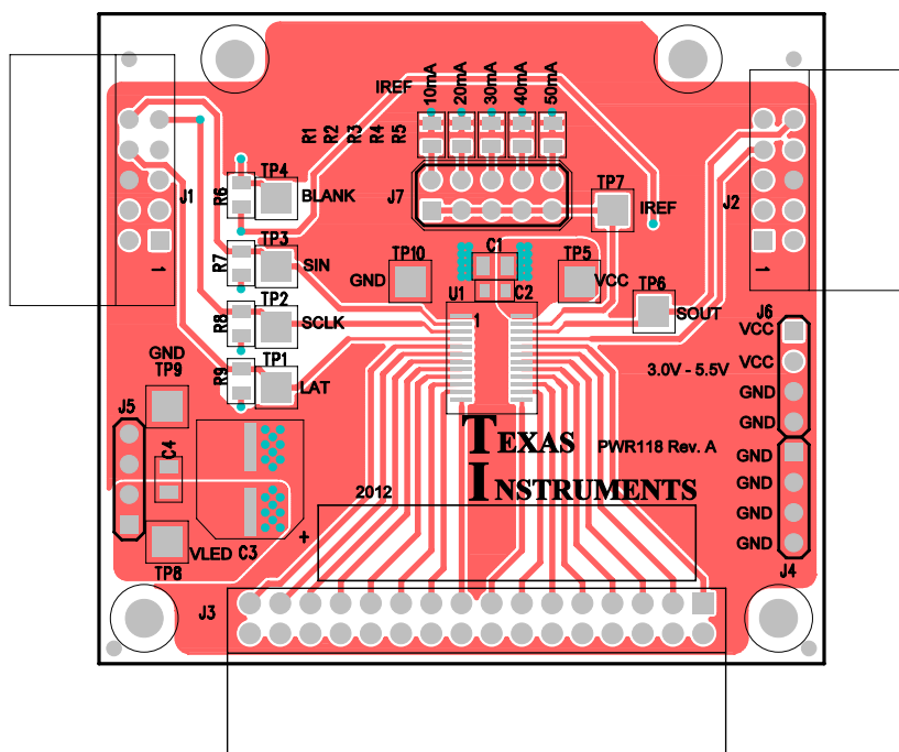
Figure 3. TLC5929 EVM Component Placement (Viewed From Top)
