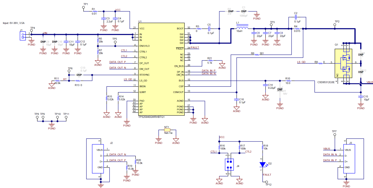
Figure 8. TPS25840Q1EVM-079 Schematic
