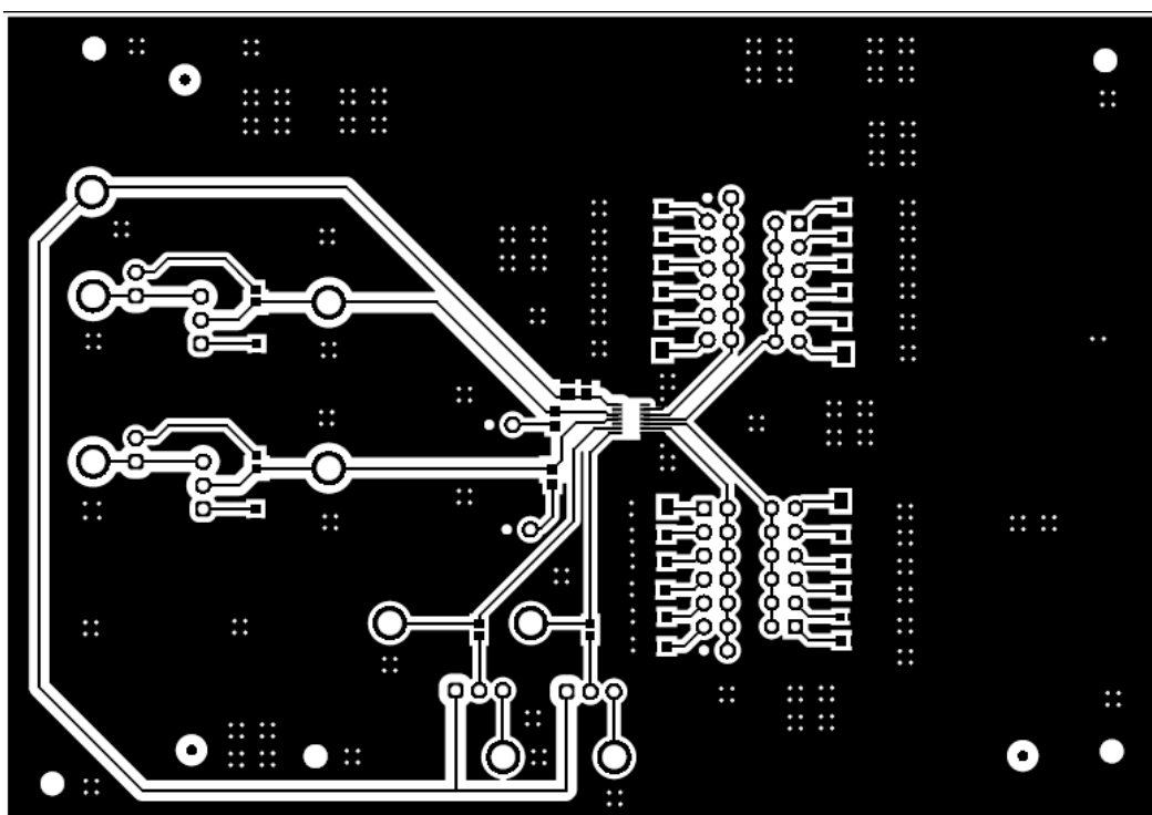
Figure 2-5. Top Layer
