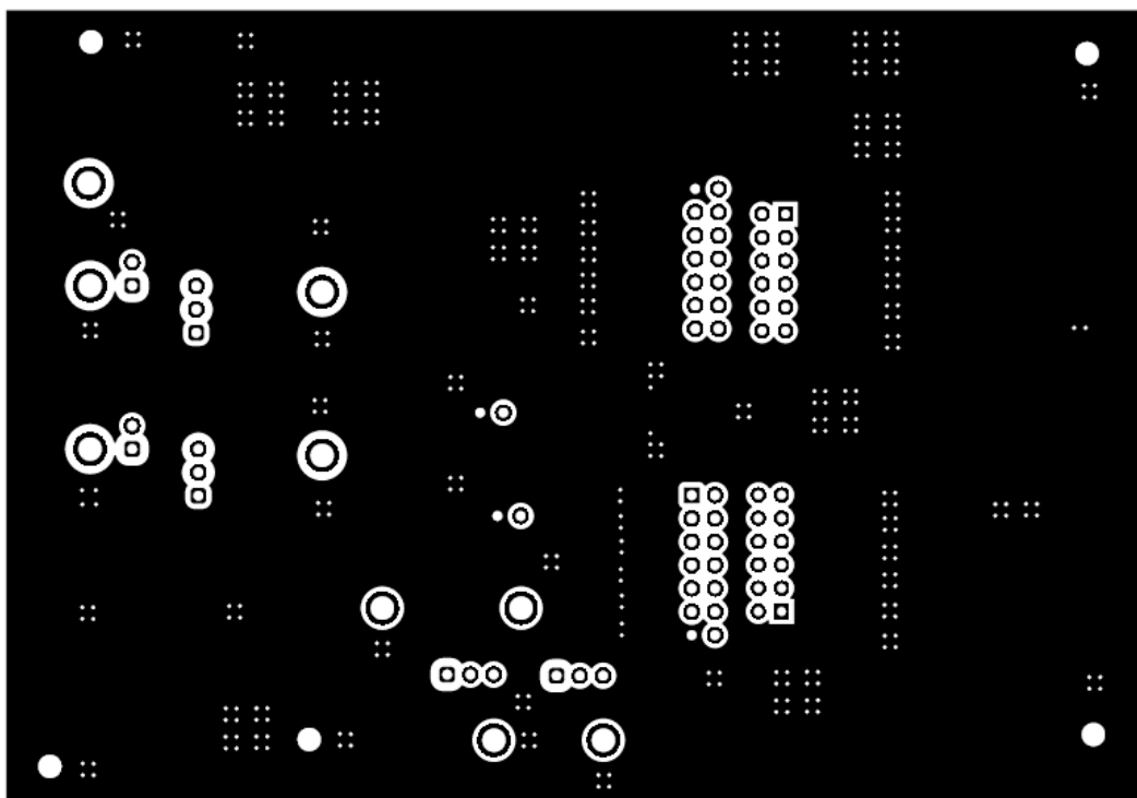
Figure 2-6. Bottom Layer
