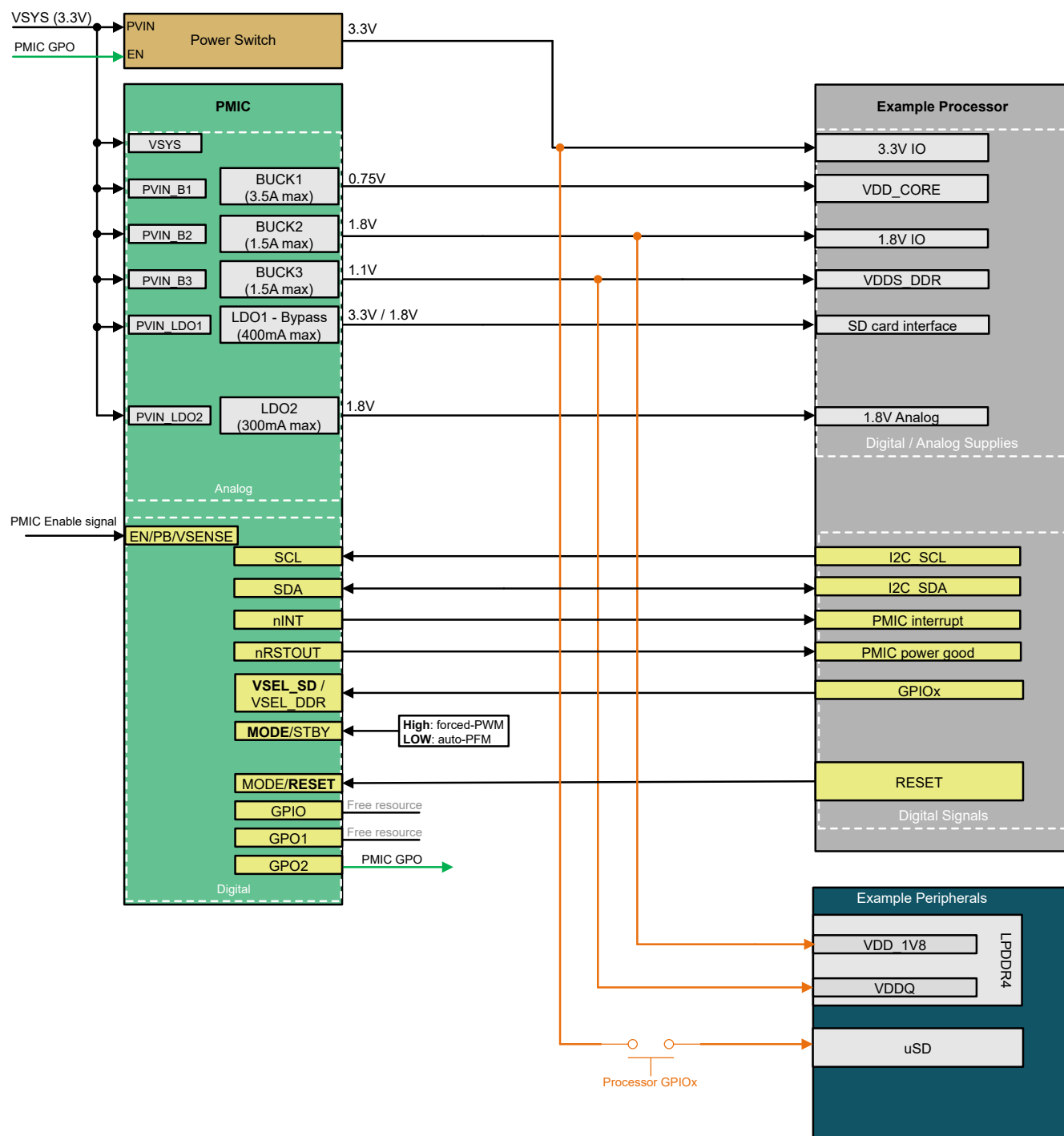
Figure 2-2. TPS6521501-Q1 Example Block Diagram
