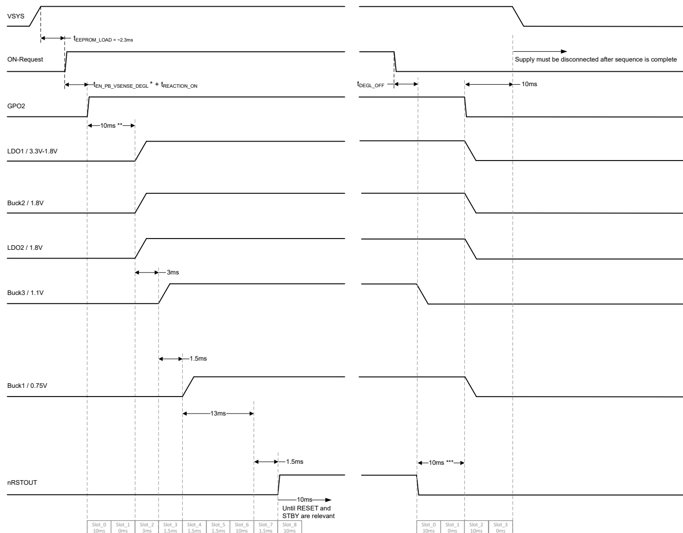
Figure 2-1. TPS6521501-Q1 Power Sequence
