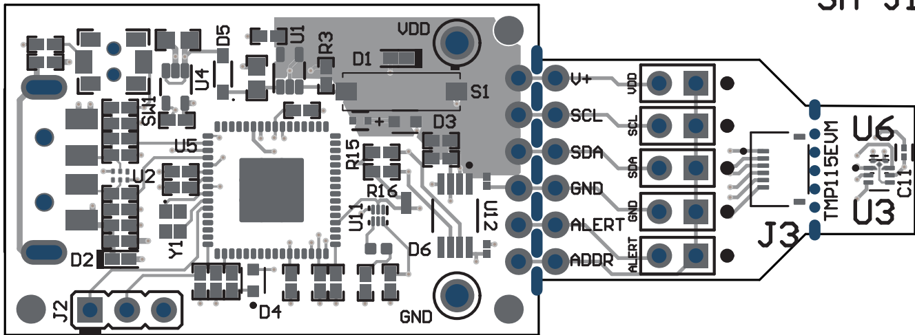
Figure 4-2. Top View
