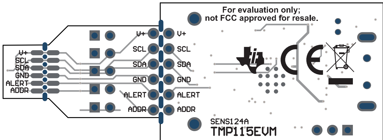
Figure 4-3. Bottom View
