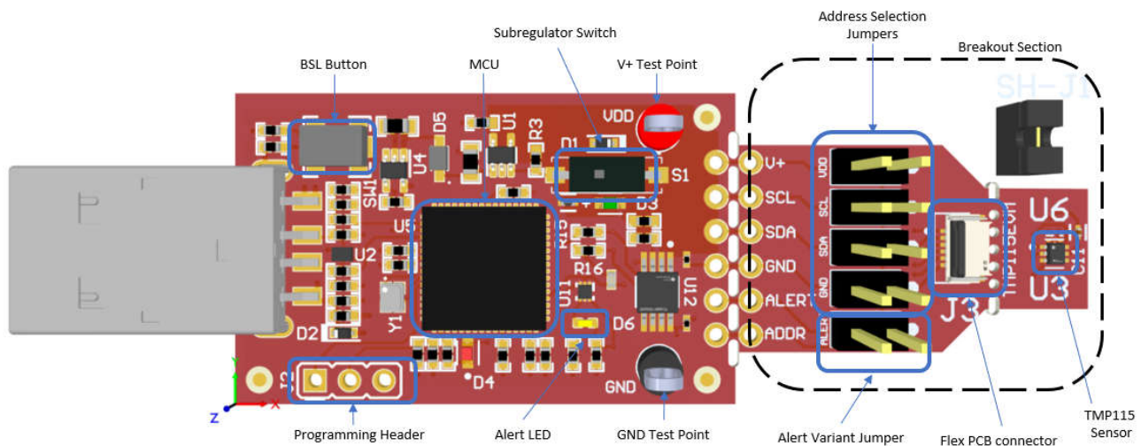
Figure 2-1. TMP115EVM Board Sections
