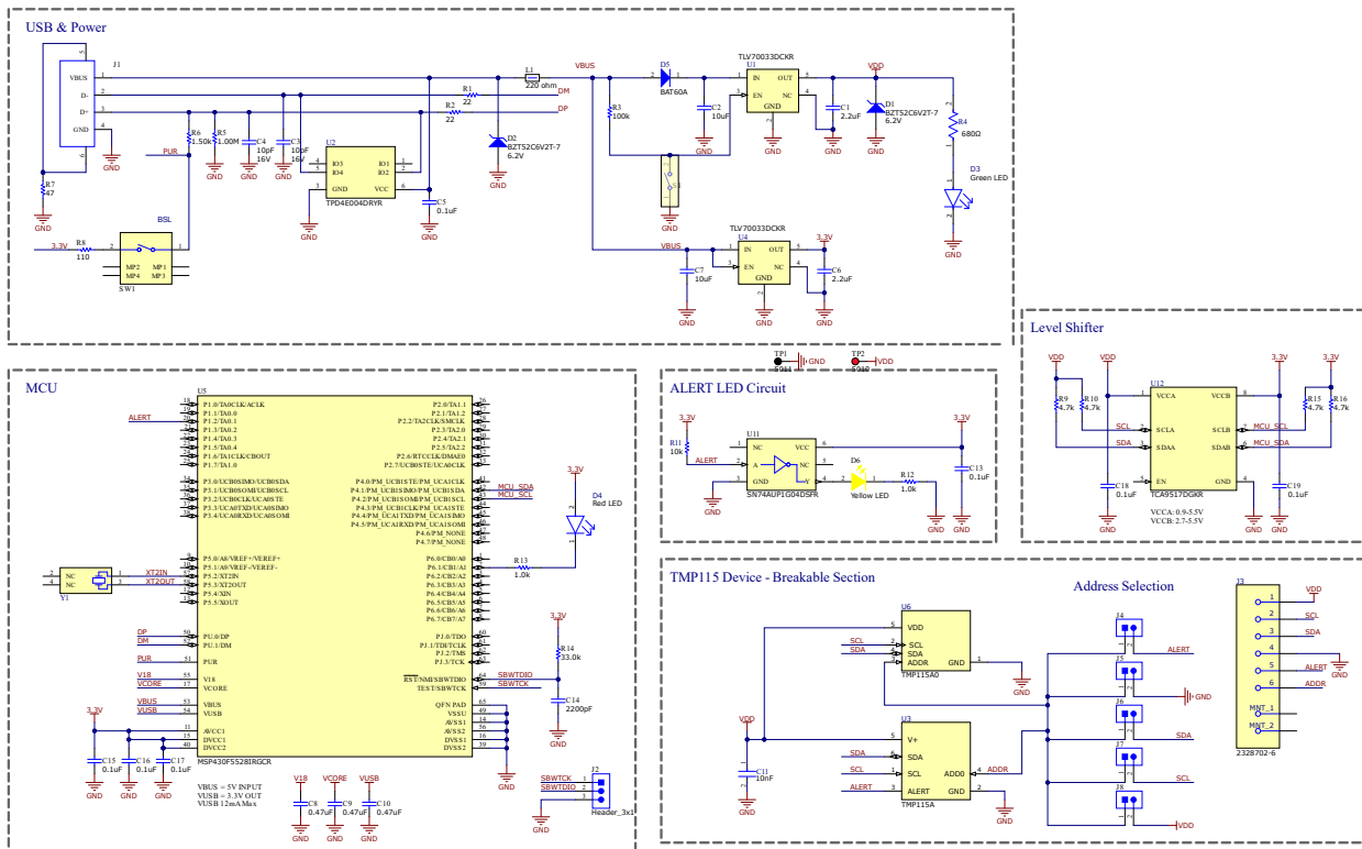
Figure 4-1. Schematic
