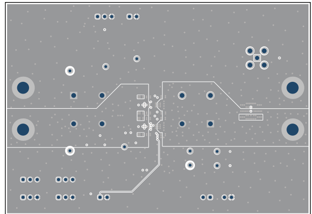
Figure 5-5. Internal Layer 2
