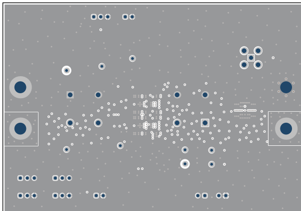
Figure 5-4. Internal Layer 1
