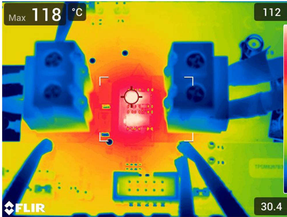
Figure 4-1. Thermal Performance (TPSM8287B30-2X-EVM, V_{IN} = 5V , V_{OUT} = 0.6V , I_{OUT} = 60A )
