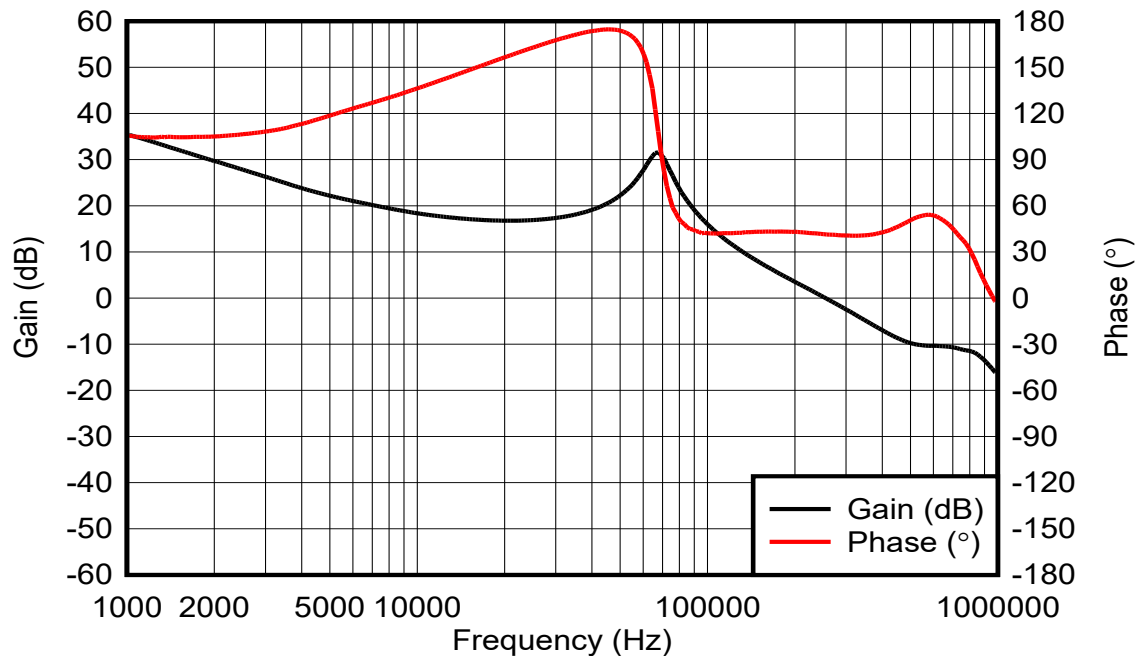
Figure 4-2. Loop Response Measurement (TPSM8287B30-2X-EVM, V_{IN} = 5V , V_{OUT} = 0.6V , I_{OUT} = 60A )
