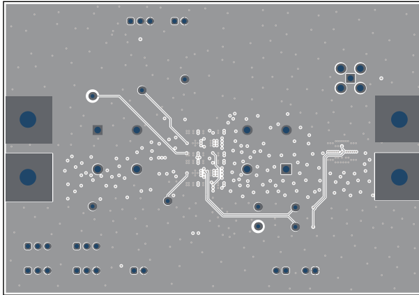
Figure 5-10. Bottom Layer
