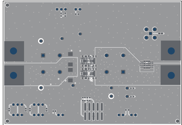
Figure 5-3. Top Layer
