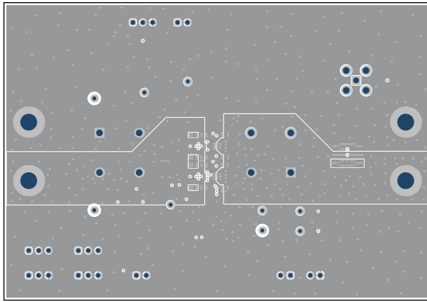
Figure 5-8. Internal Layer 5
