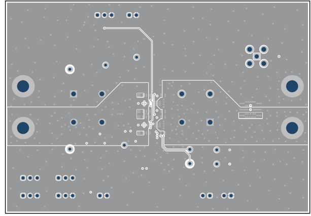
Figure 5-9. Internal Layer 6
