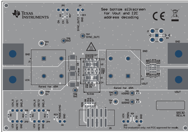
Figure 5-2. Top Assembly
