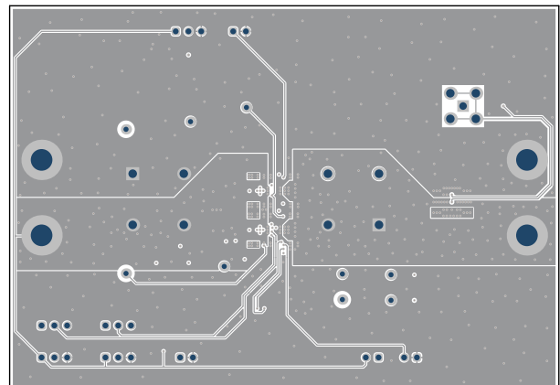
Figure 5-7. Internal Layer 4
