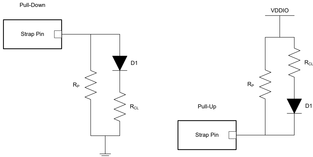
Figure 2-6. DP83826A LED Strap Circuit
