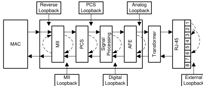
Figure 8-8. Loopback Test Modes
