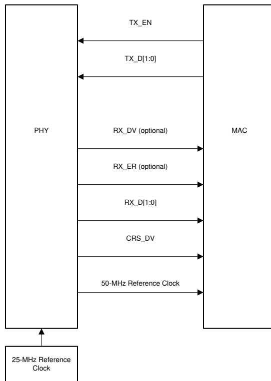
Figure 8-7. RMII Leader Signaling
