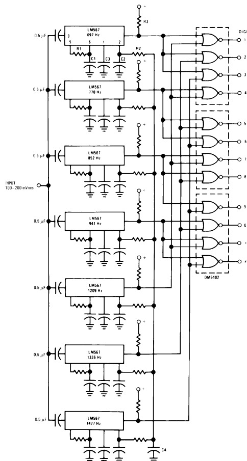
Figure 10-1. Touch-Tone Decoder
