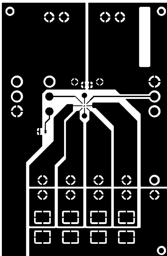
Figure 4. LP5524 Evaluation Board Layer 1 (Top).
