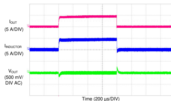
Figure 8-30. TPS7H4010-SEP Load Transients
