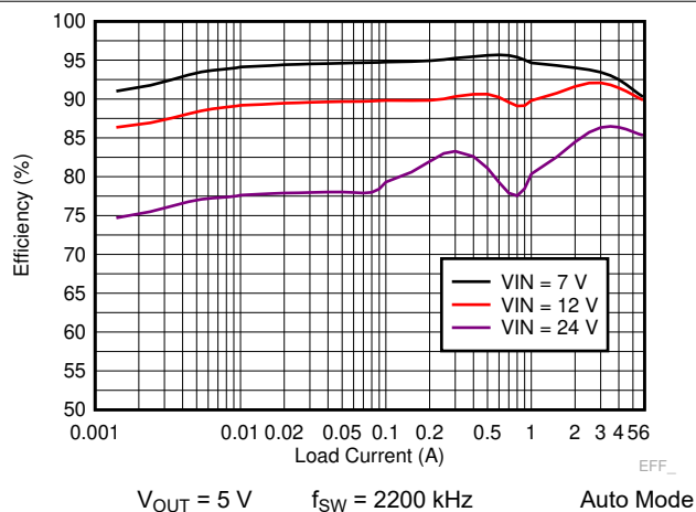
Figure 8-7. TPS7H4010-SEP Efficiency
