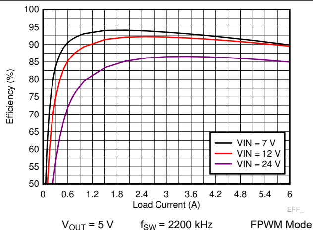
Figure 8-8. TPS7H4010-SEP Efficiency
