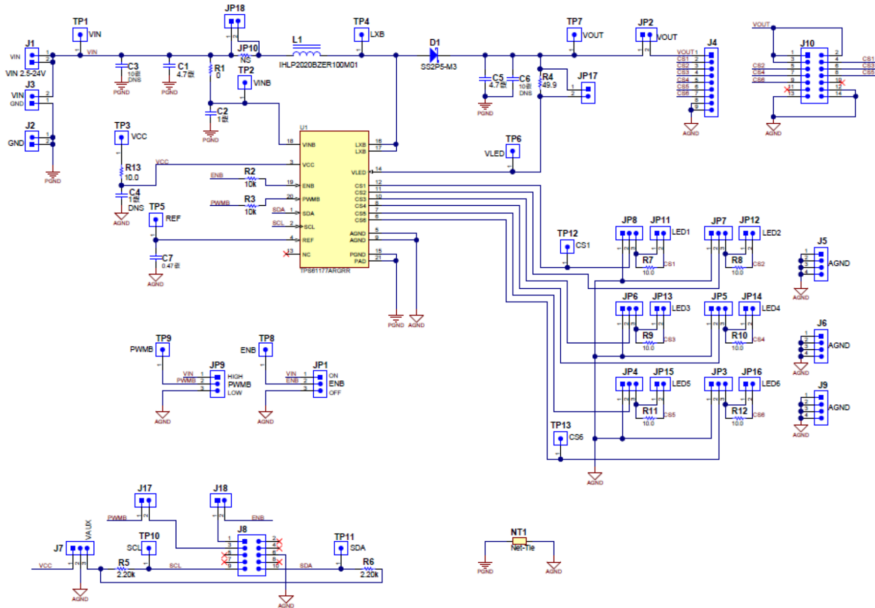
Figure 10. TPS61177AEVM Schematic
