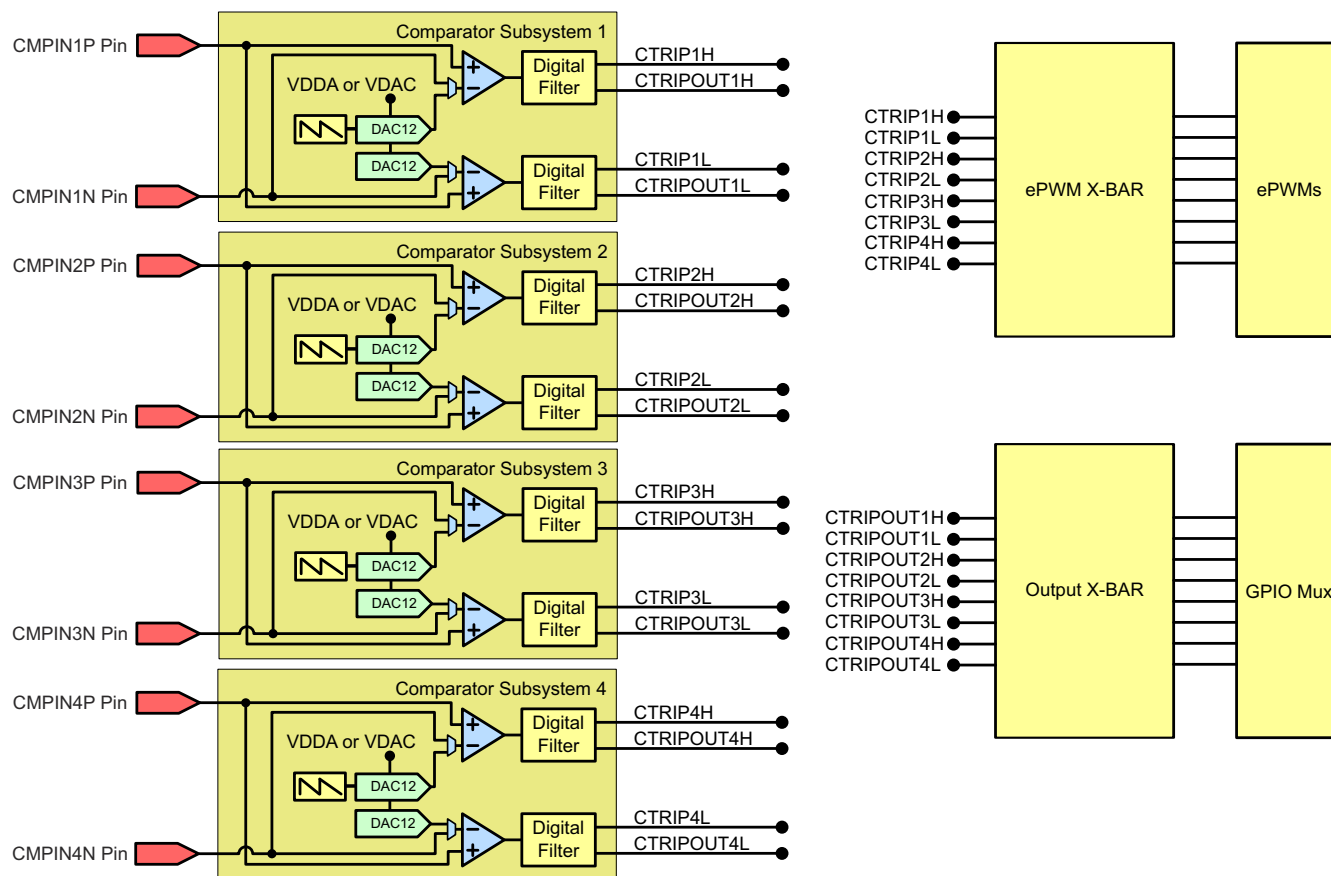
Figure 6-38. CMPSS Connectivity (100-Pin PZP)
