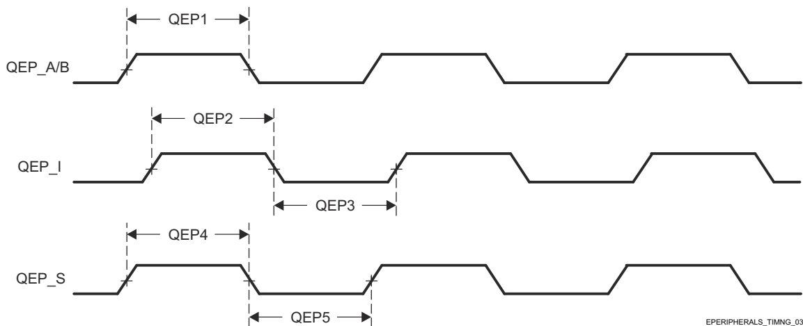
Figure 6-41. EQEP Timing Requirements
