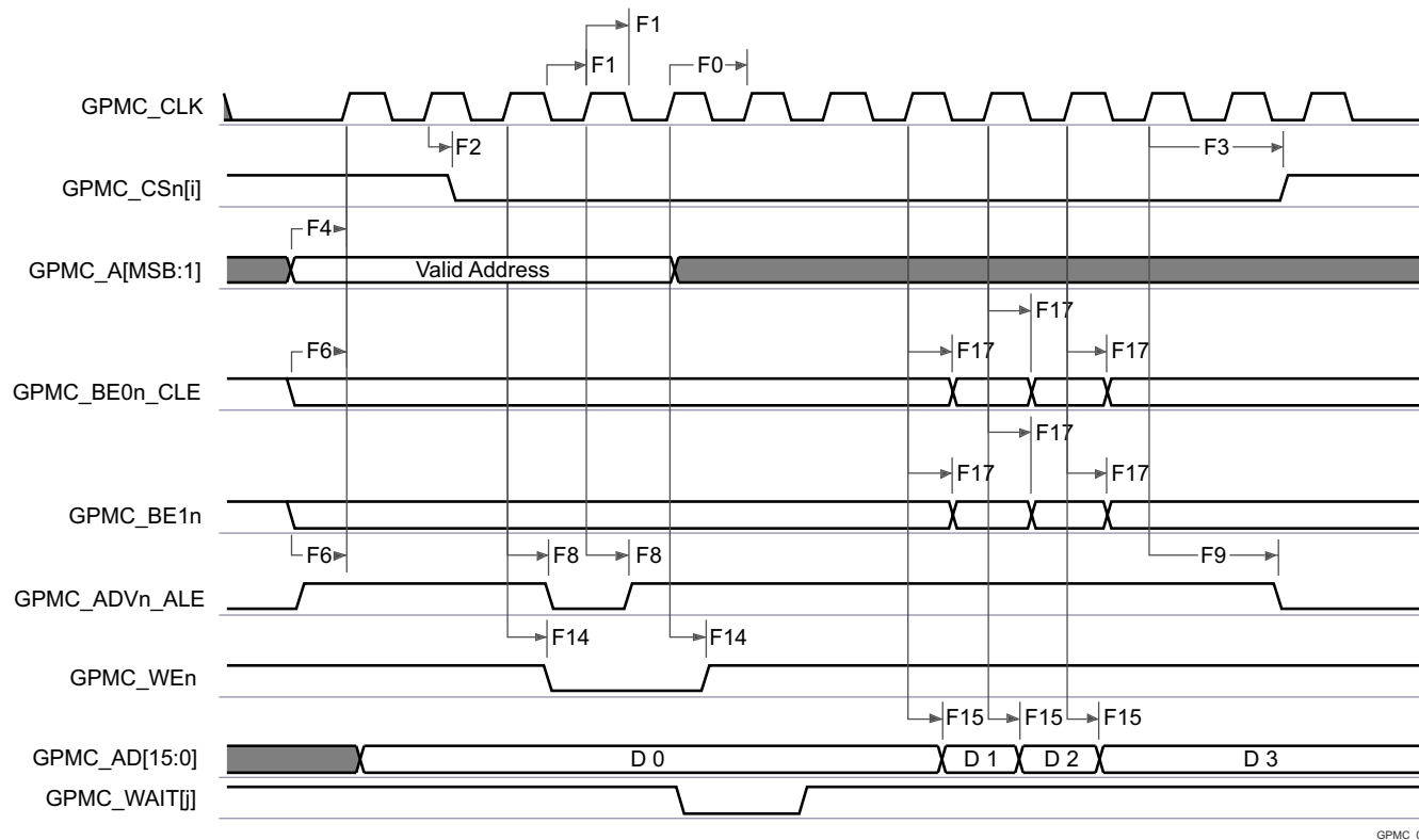
Figure 6-43. GPMC and NOR Flash — Synchronous Burst Read — 4x16-bit (GPMCFCLKDIVIDER = 0)
