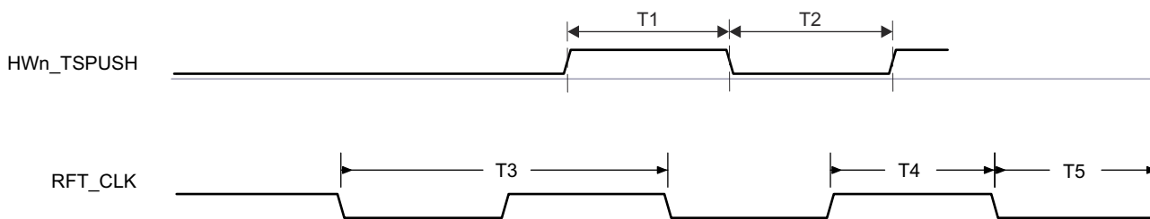
Figure 6-30. CPTS Timing Requirements
