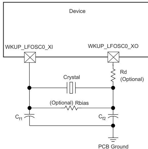
Figure 6-19. WKUP_LFOSC0 Crystal Implementation
