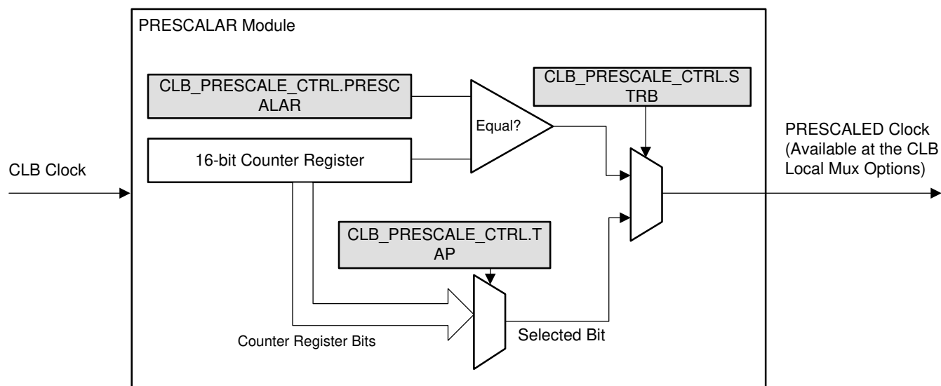
Figure 9-4. CLB Clock Prescaler
