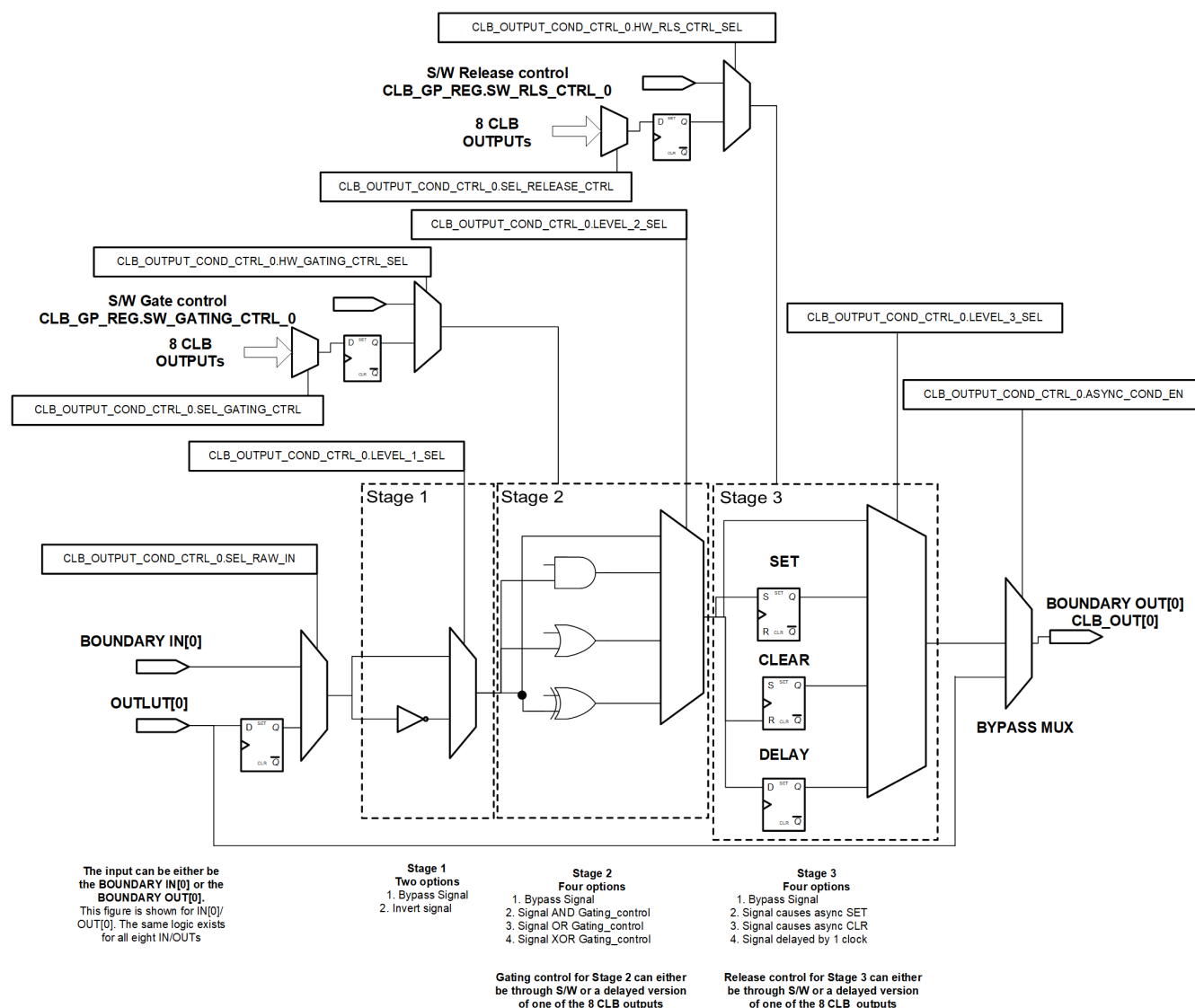
Figure 9-18. AOC Block
