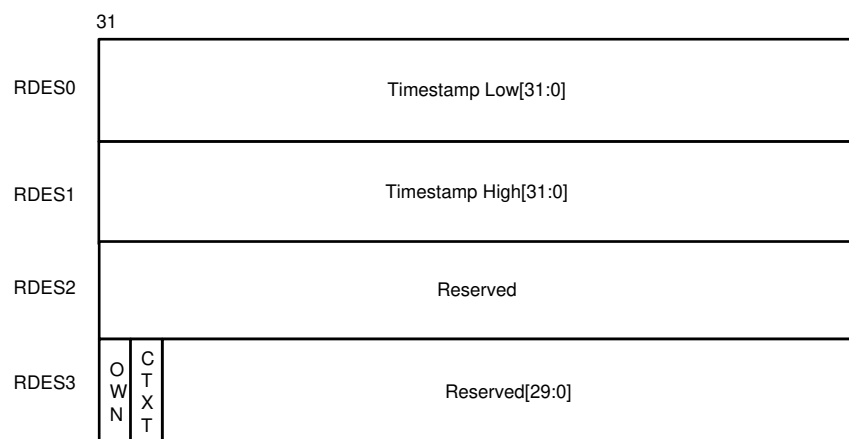
Figure 43-26. Receive Context Descriptor Format
