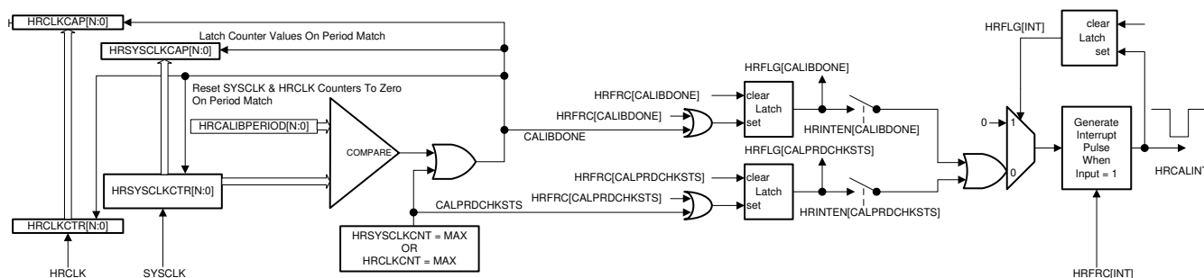
Figure 25-2. HRCAP Calibration
