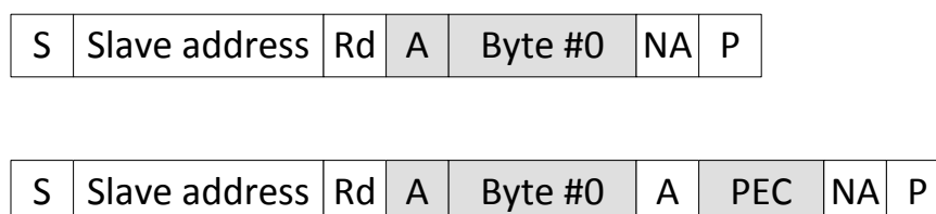
Figure 35-17. Receive Byte Message With and Without PEC
