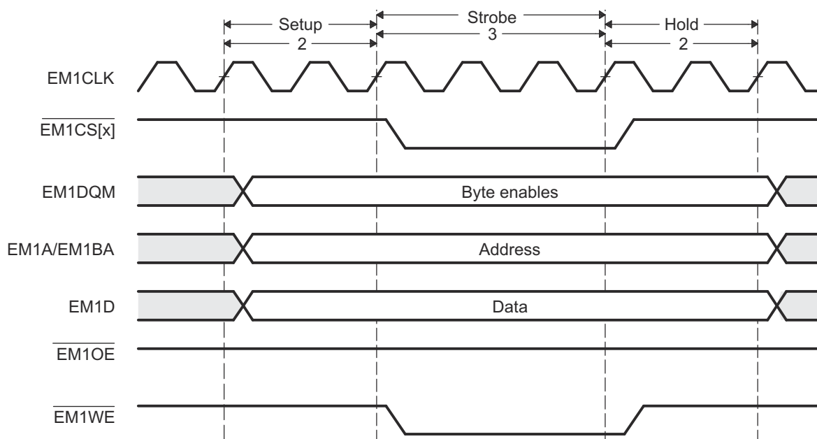
Figure 12-14. Timing Waveform of an Asynchronous Write Cycle in Select Strobe Mode
