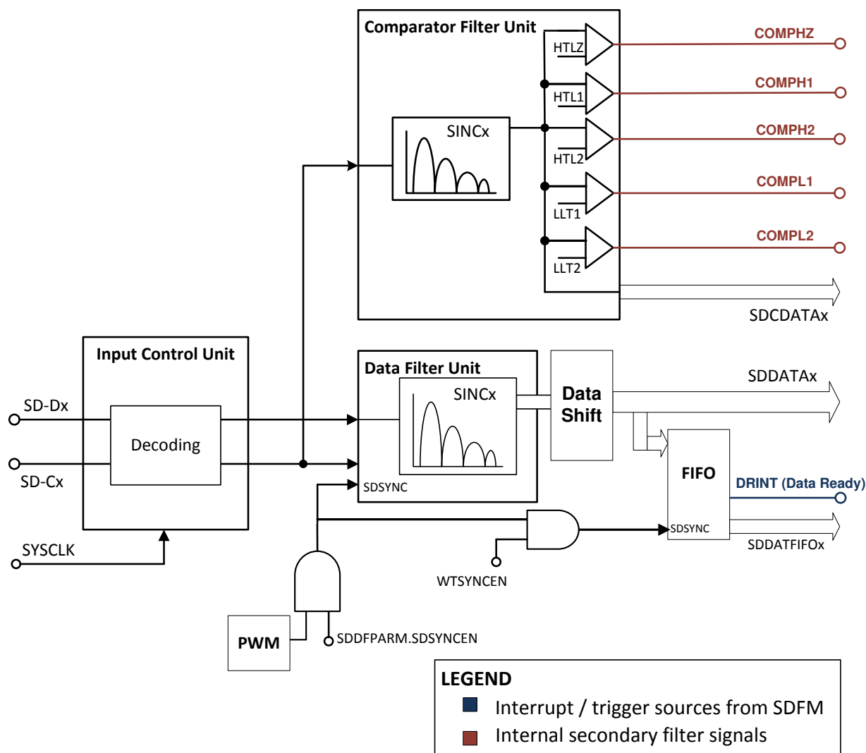
Figure 28-3. Block Diagram of One Filter Module
