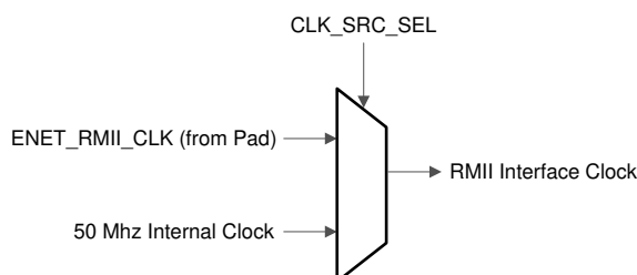
Figure 43-5. RMII Clocking
