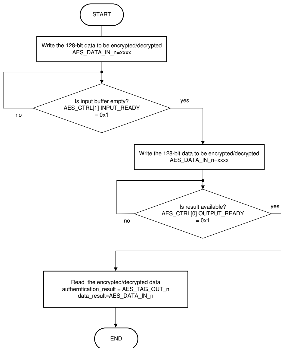
Figure 42-12. AES Polling Mode
