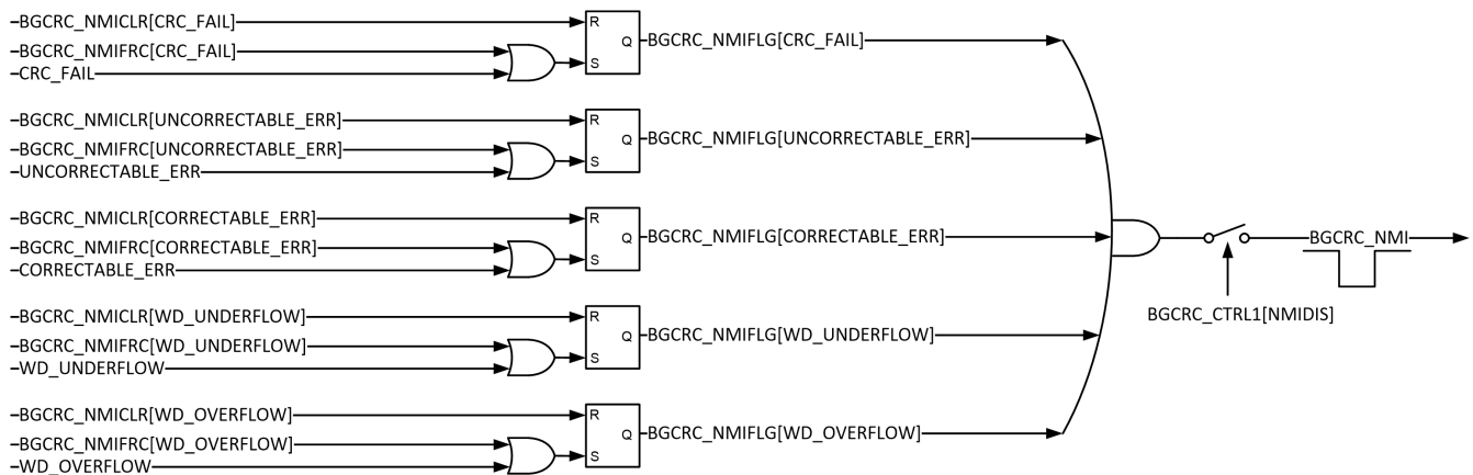
Figure 7-3. BGCRC NMI
