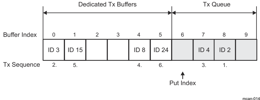
Figure 45-18. Mixed Dedicated Tx Buffers /Tx Queue (example)
