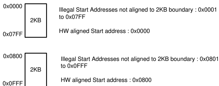
Figure 41-12. Unaligned Start Address
