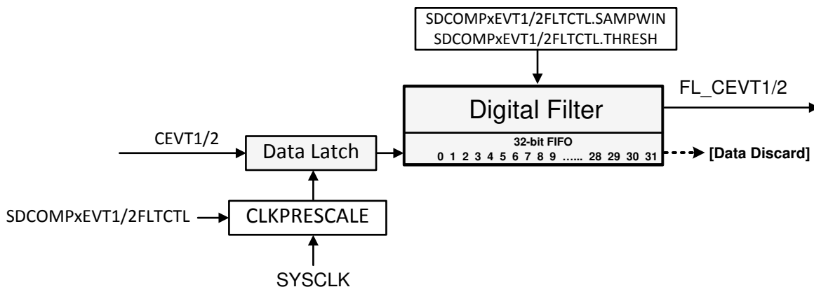
Figure 28-12. Digital Filter
