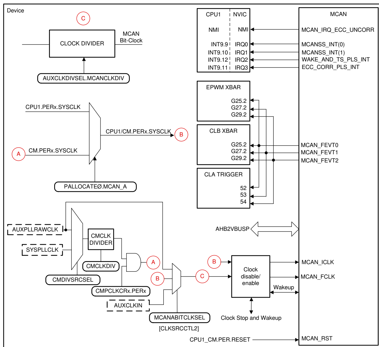
Figure 45-3. MCAN Integration
