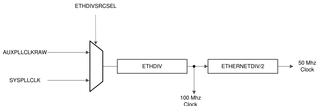
Figure 43-4. Ethernet Clocking
