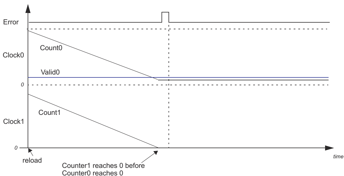
Figure 10-5. Clock1 Faster Than Clock0 - Results in an Error and Stops Counting
