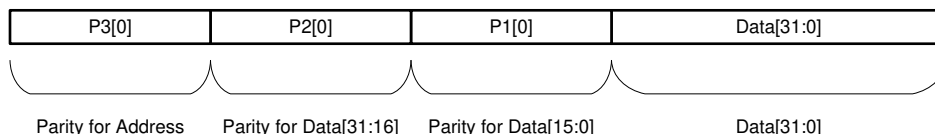
Figure 41-9. Content of Each Memory Location for Parity Memories
