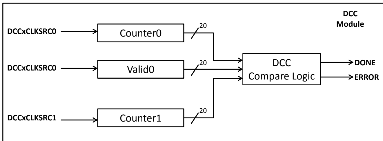
Figure 10-2. DCC Operation
