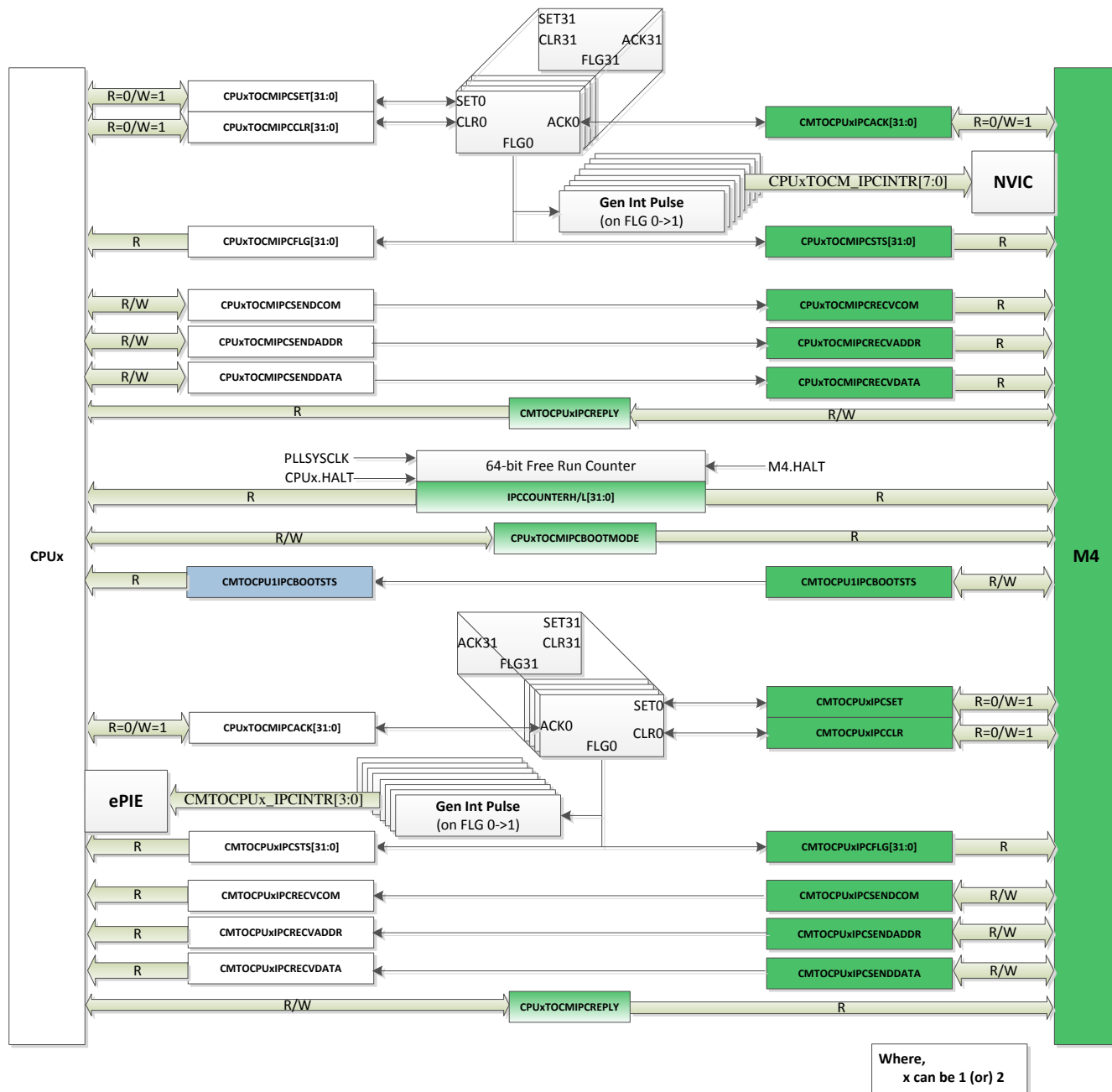
Figure 16-2. CPuX_to_CM IPC Module
