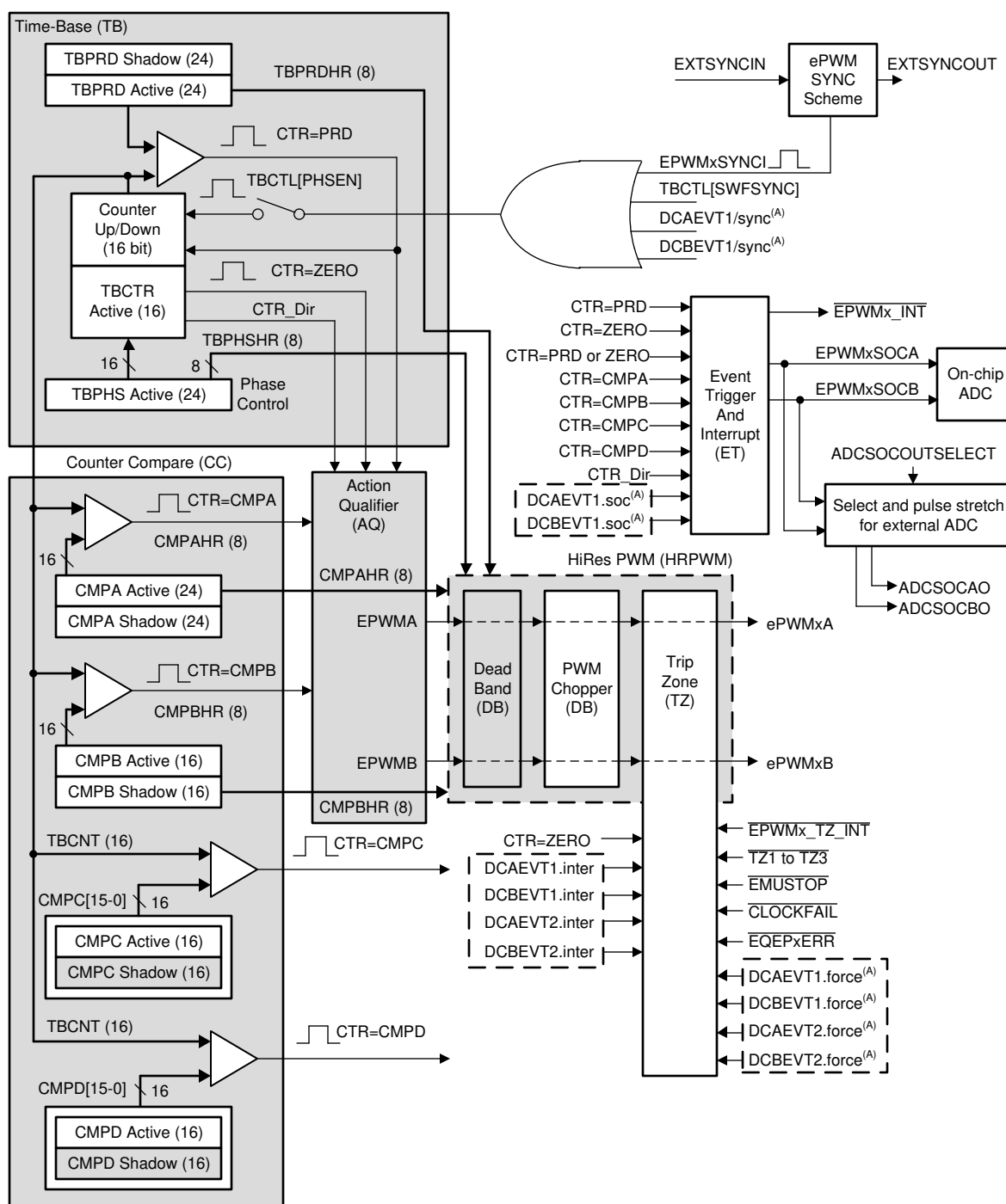
Figure 26-3. ePWM Modules and Critical Internal Signal Interconnects
