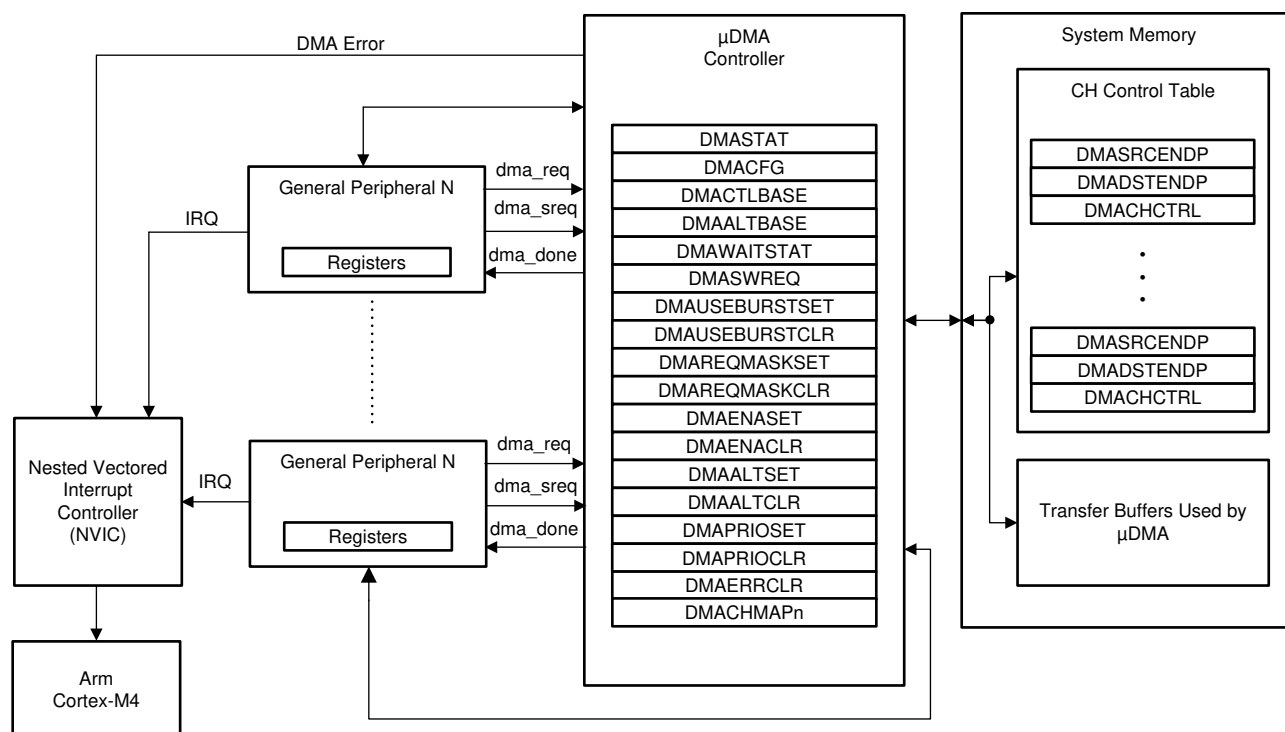
Figure 49-1. \mu DMA Block Diagram
