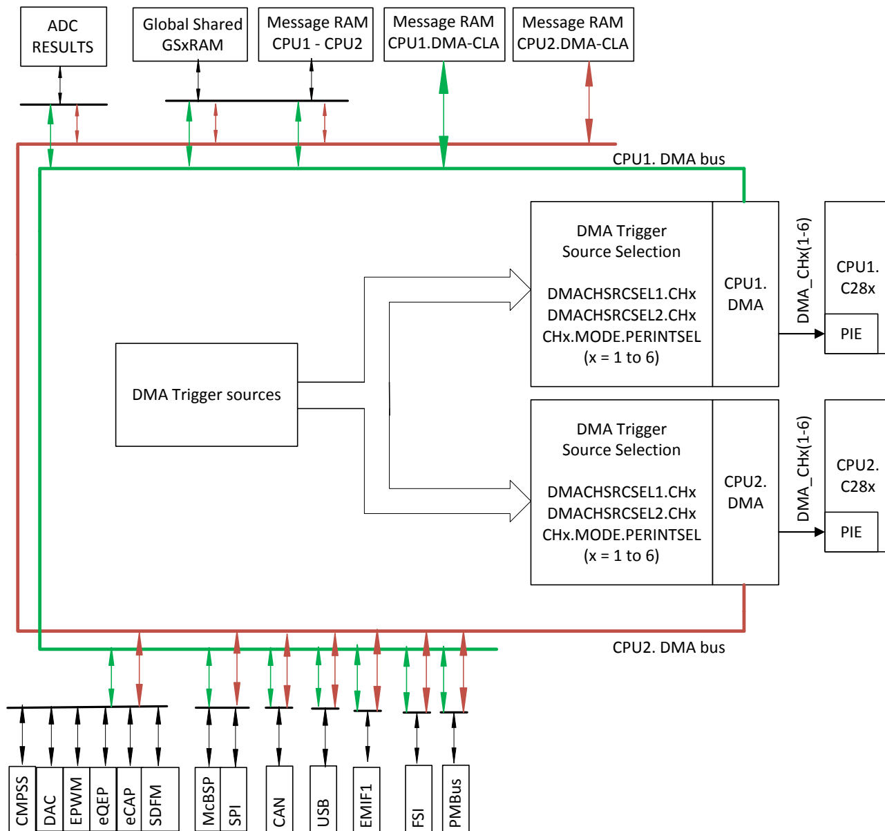
Figure 11-1. DMA Block Diagram
