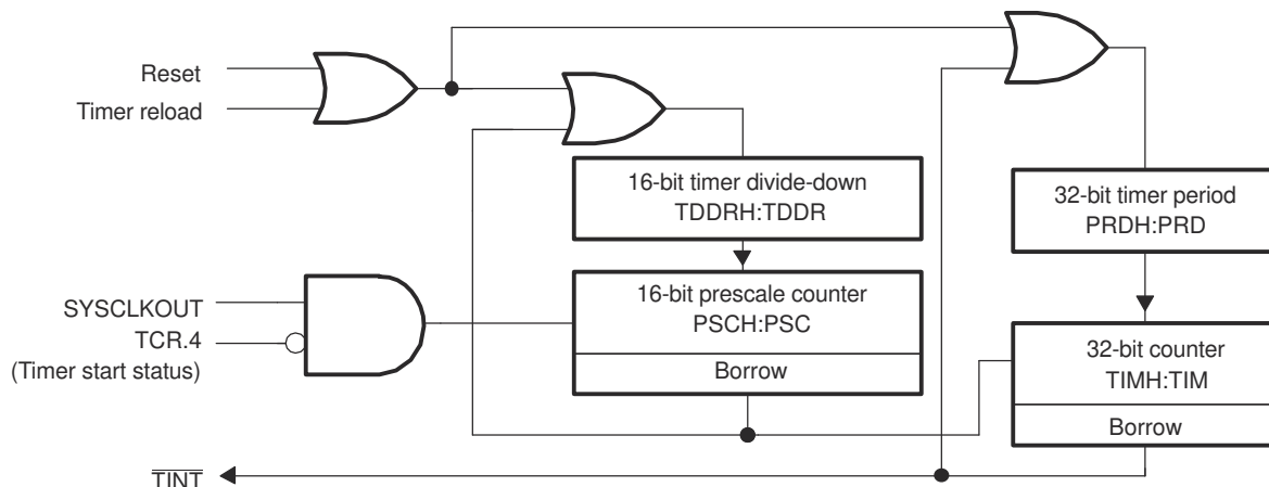
Figure 3-13. CPU-Timers
