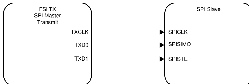
Figure 32-14. FSITX as SPI Master, Transmit Only
