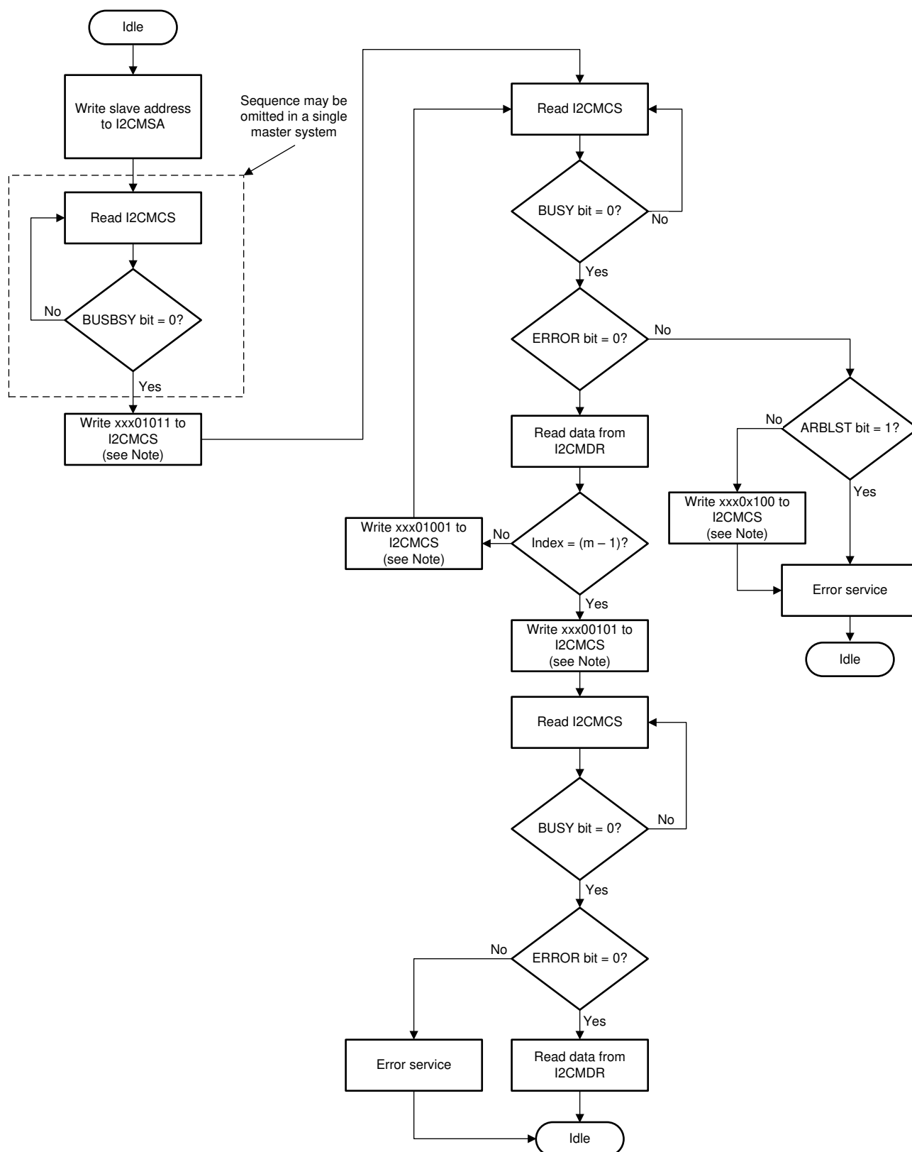
Figure 46-11. Master Receive of Multiple Data Bytes
