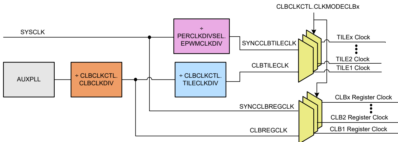
Figure 9-3. CLB Clocking
