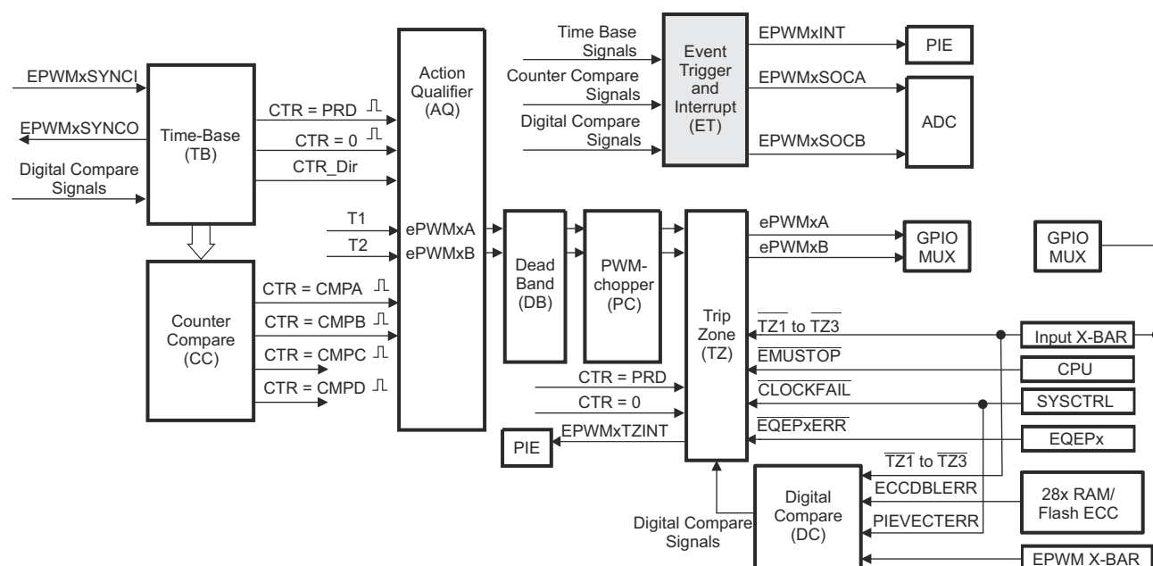
Figure 26-45. Event-Trigger Submodule
