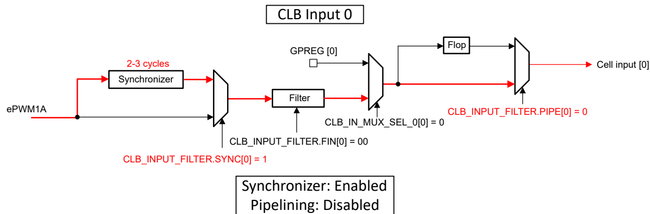
Figure 9-7. CLB Input Synchronization Example
