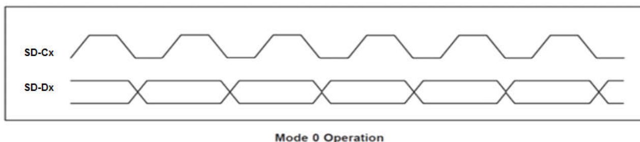
Figure 28-5. Different Modulator Modes Supported
