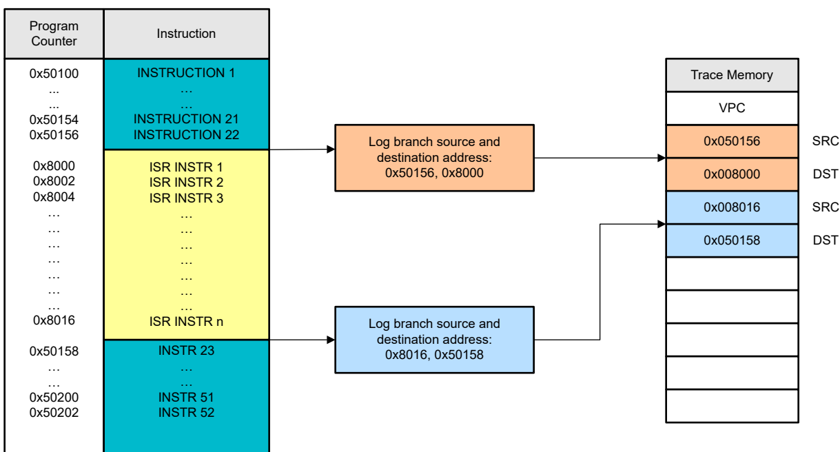
Figure 14-5. PC Trace Operation
