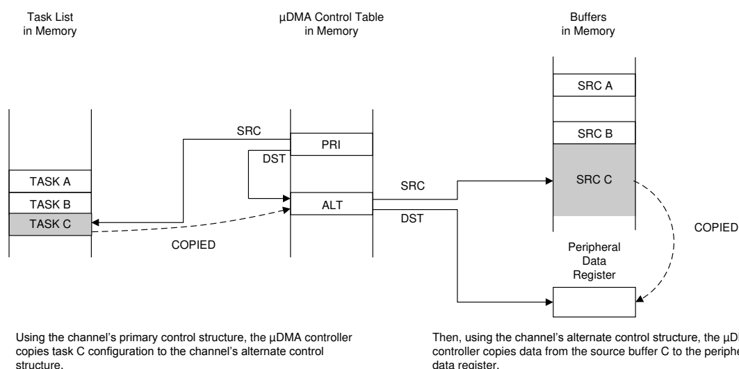
Figure 49-6. Peripheral Scatter-Gather, \mu DMA Copy Sequence
