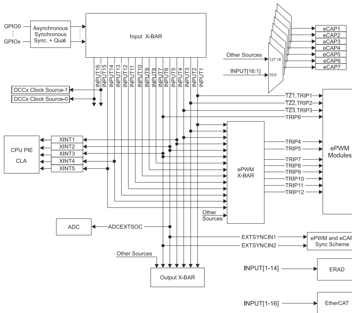
Figure 17-1. Input X-BAR
