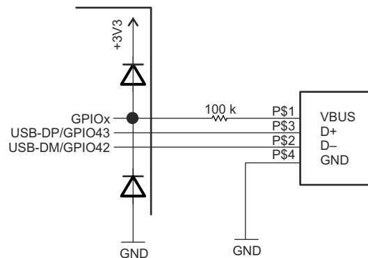
Figure 38-2. USB Scheme
