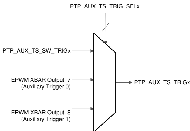
Figure 43-7. Trigger Sources for Auxiliary Timestamping
