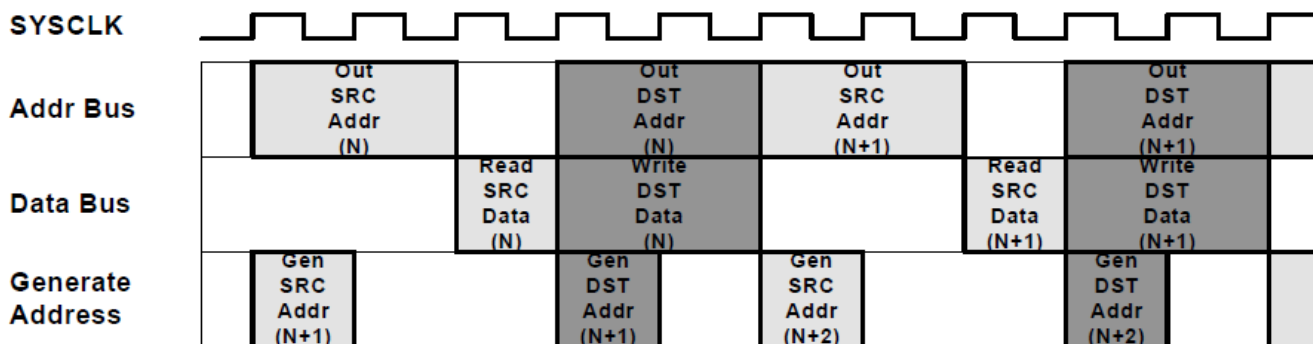
Figure 11-6. 3-stage Pipeline with One Read Stall
