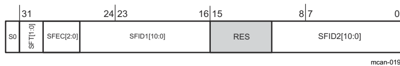
Figure 45-23. Standard Message ID Filter Element Structure
