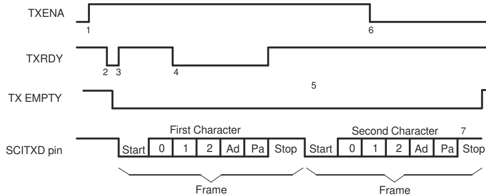
Figure 36-9. SCI TX Signals in Communications Mode
