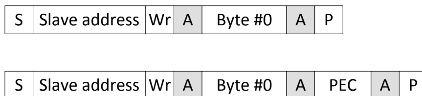
Figure 35-3. Send Byte Message With and Without PEC
