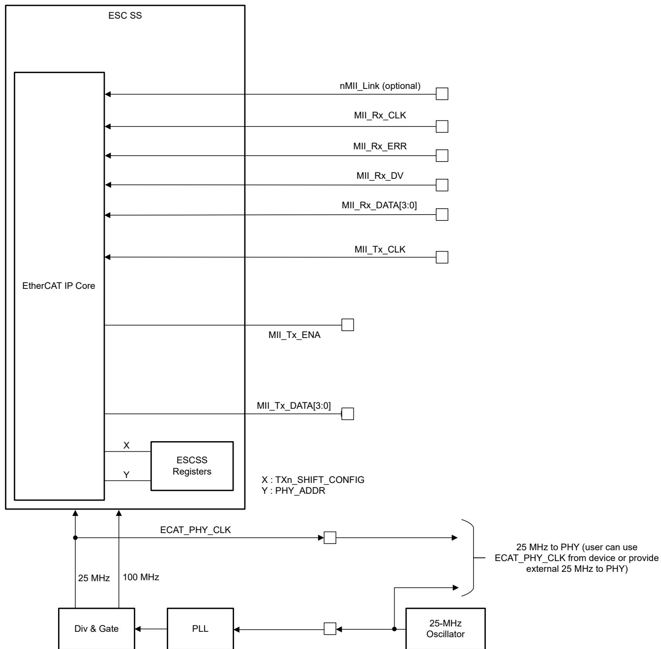
Figure 31-4. ESC PHY Interface Diagram
