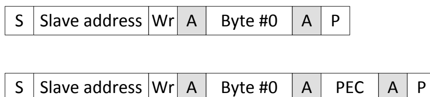
Figure 35-16. Send Byte Message With and Without PEC
