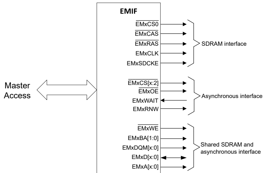
Figure 12-2. EMIF Functional Block Diagram
