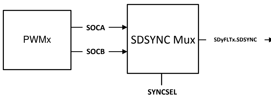
Figure 28-10. SDSYNC Event
