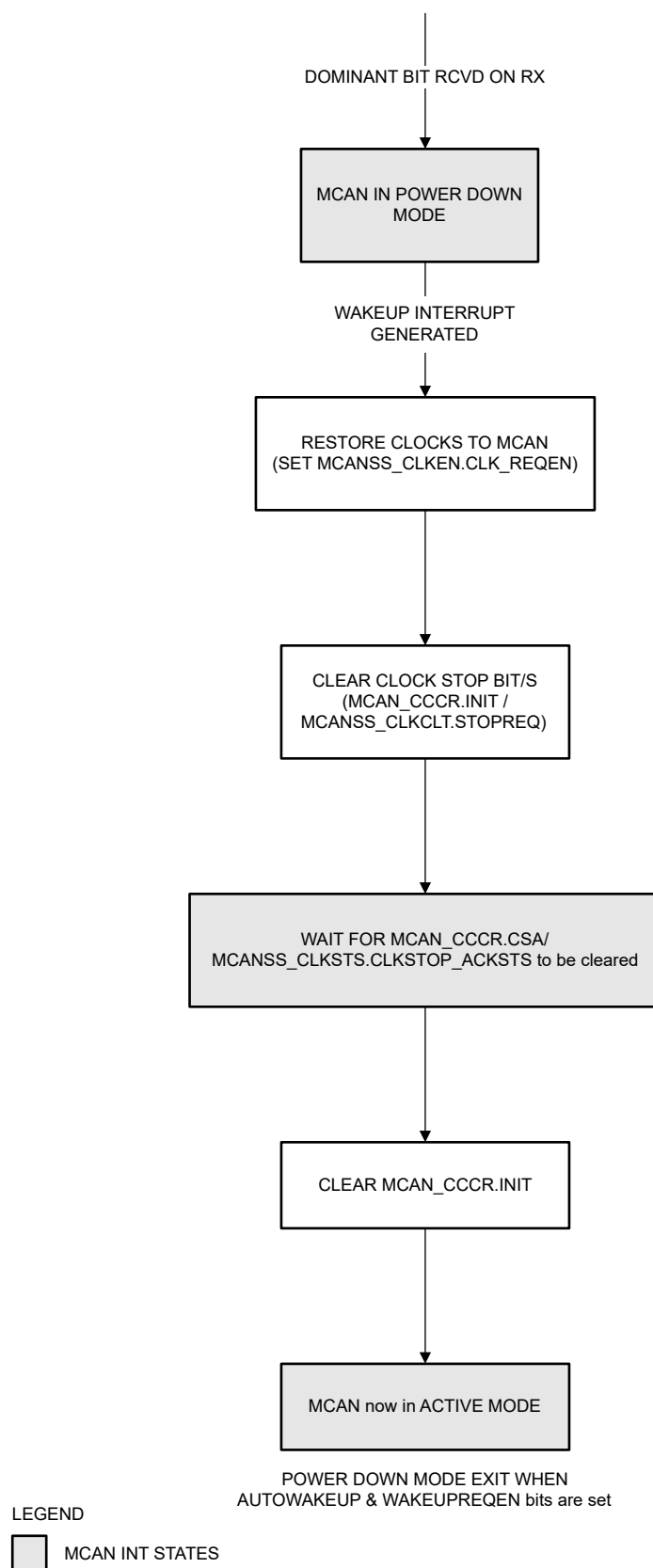
Figure 45-9. Auto Wakeup Enabled Exit from Power Down
