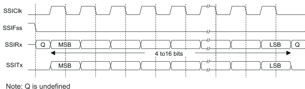
Figure 47-6. Freescale SPI Frame Format with SPO =0 and SPH=1
