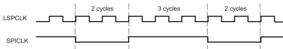
Figure 37-8. SPI: SPICLK-LSPCLK Characteristic when (BRR + 1) is Odd, BRR > 3 , and CLKPOLARITY = 1
