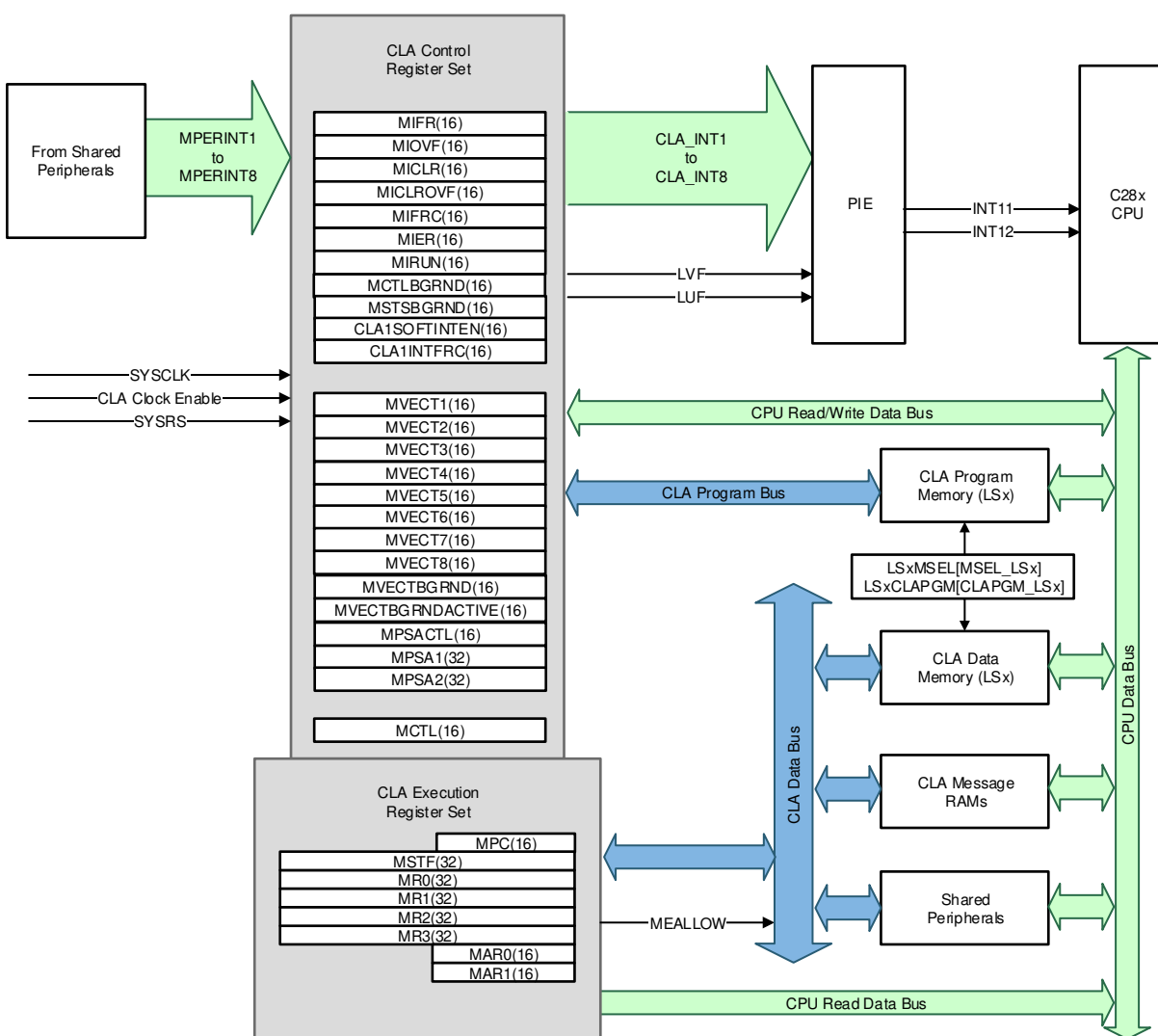
Figure 8-1. CLA Block Diagram
