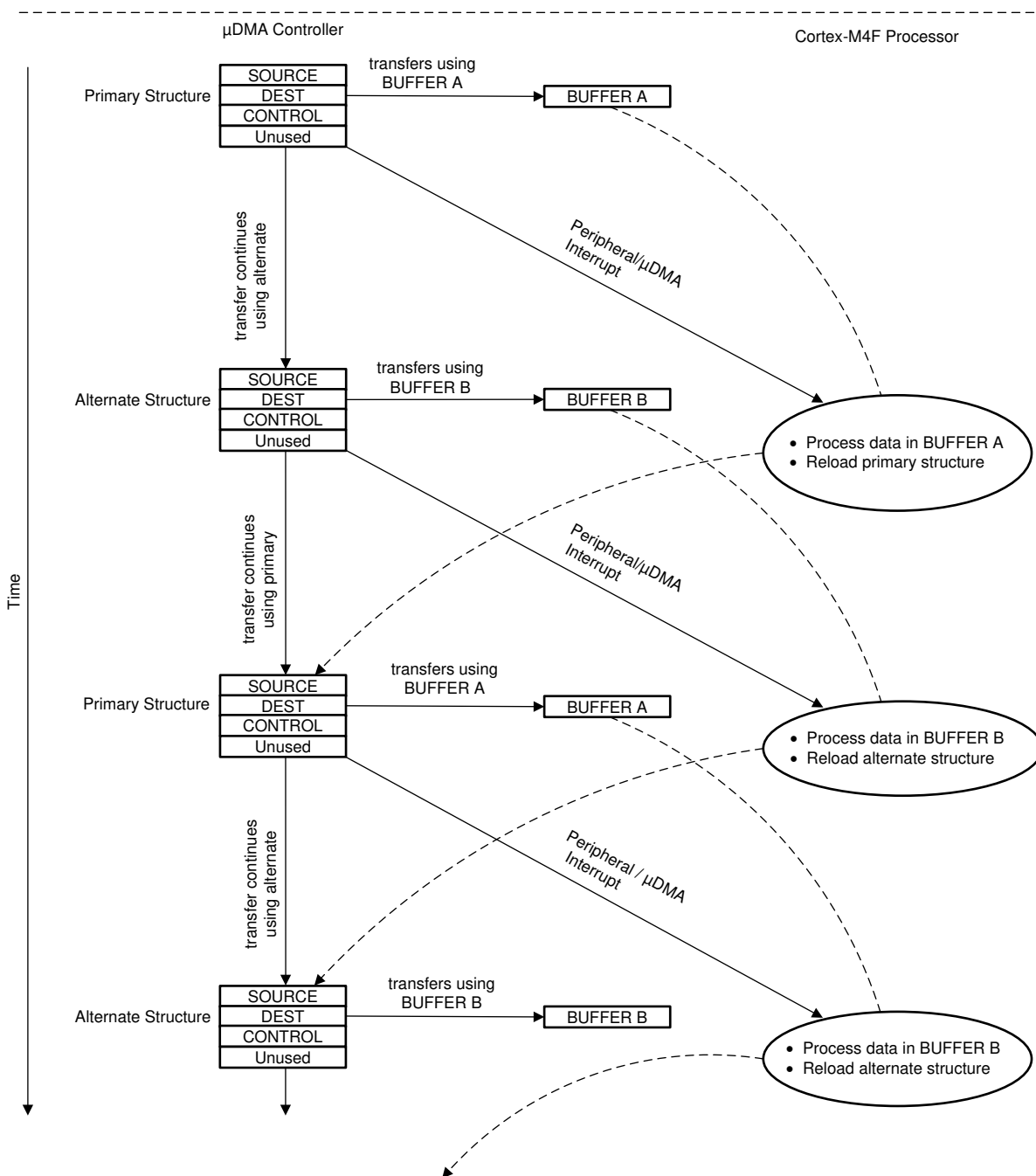
Figure 49-2. Example of Ping-Pong \mu DMA Transaction
