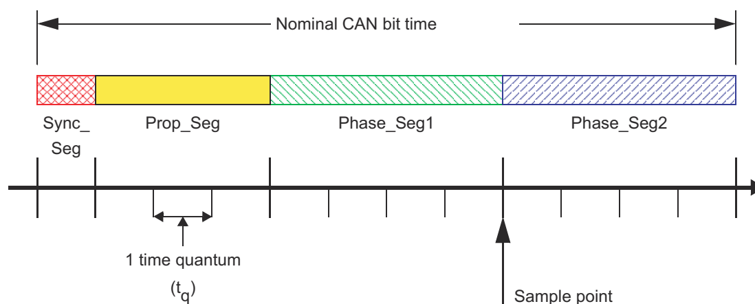
Figure 30-14. Bit Timing
