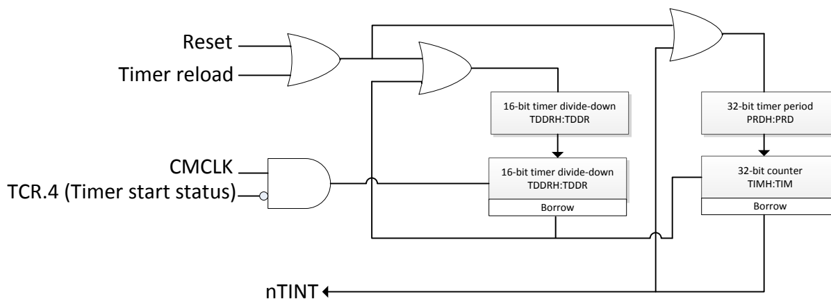
Figure 41-3. CM CPU-Timers
