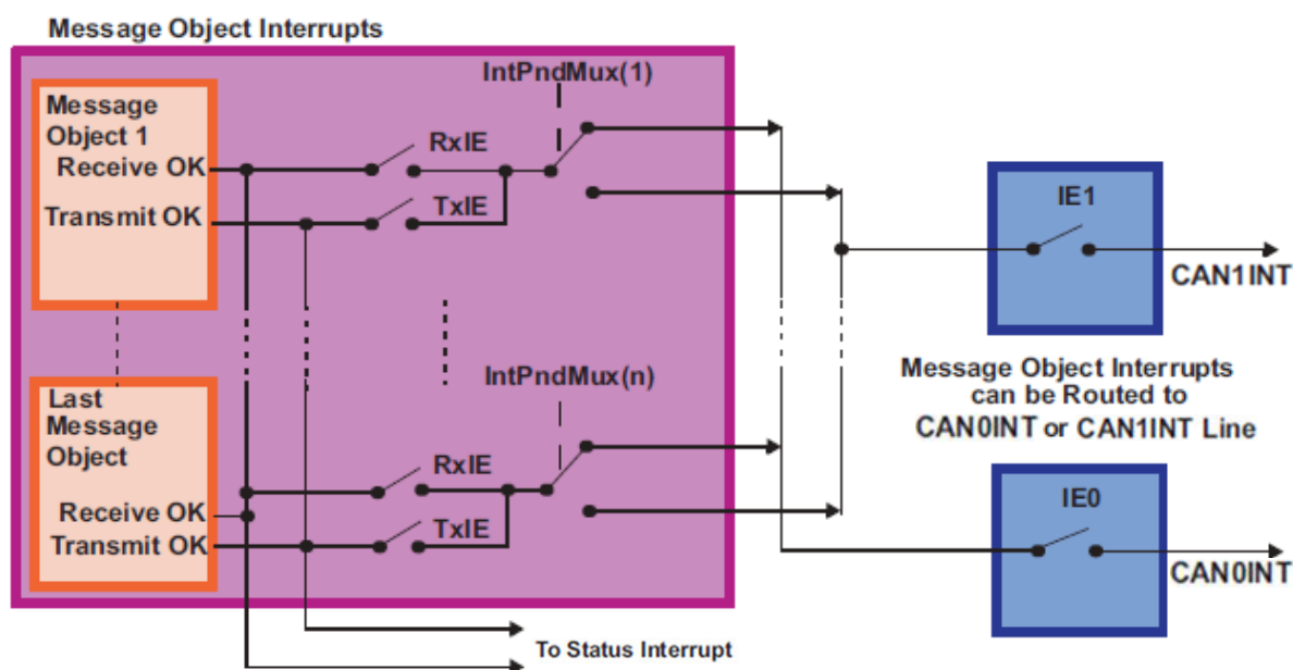
Figure 30-9. CAN Interrupt Topology 2
