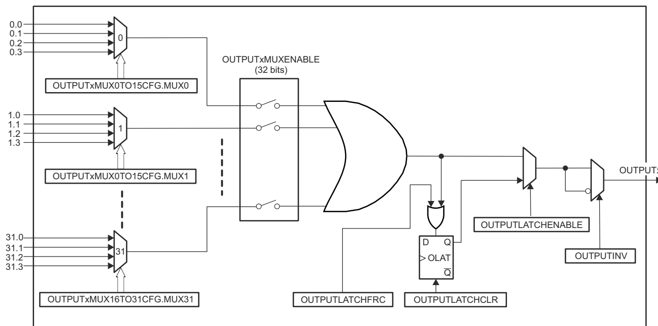
Figure 17-5. GPIO Output X-BAR Architecture
