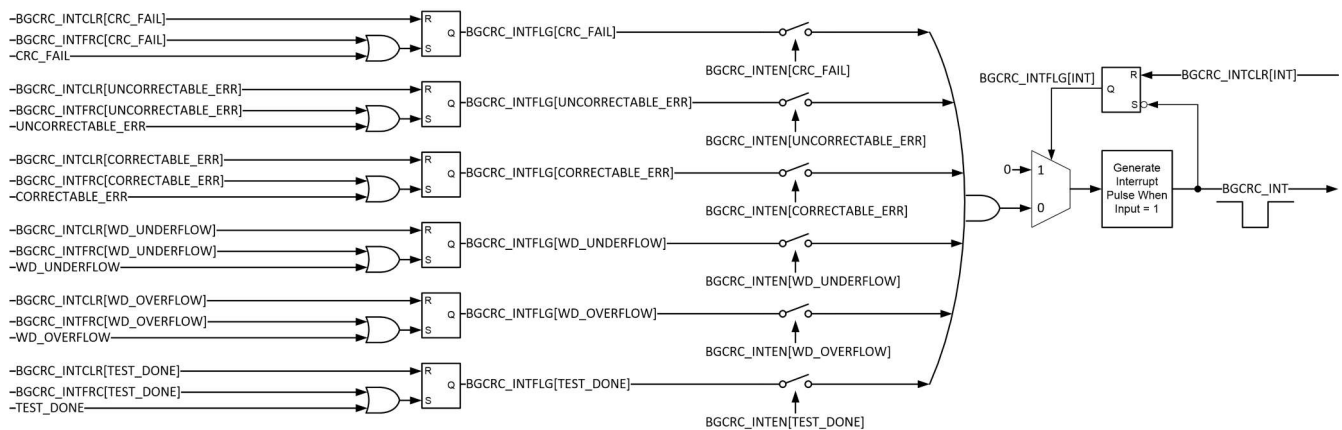
Figure 7-4. BGCRC Interrupt
