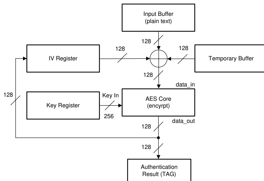
Figure 42-11. AES - CBC-MAC Authentication Mode
