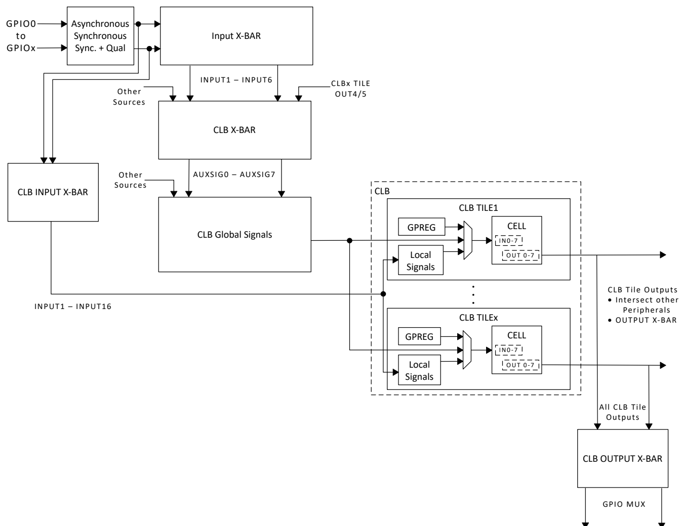
Figure 9-5. GPIO to CLB Tile Connections
