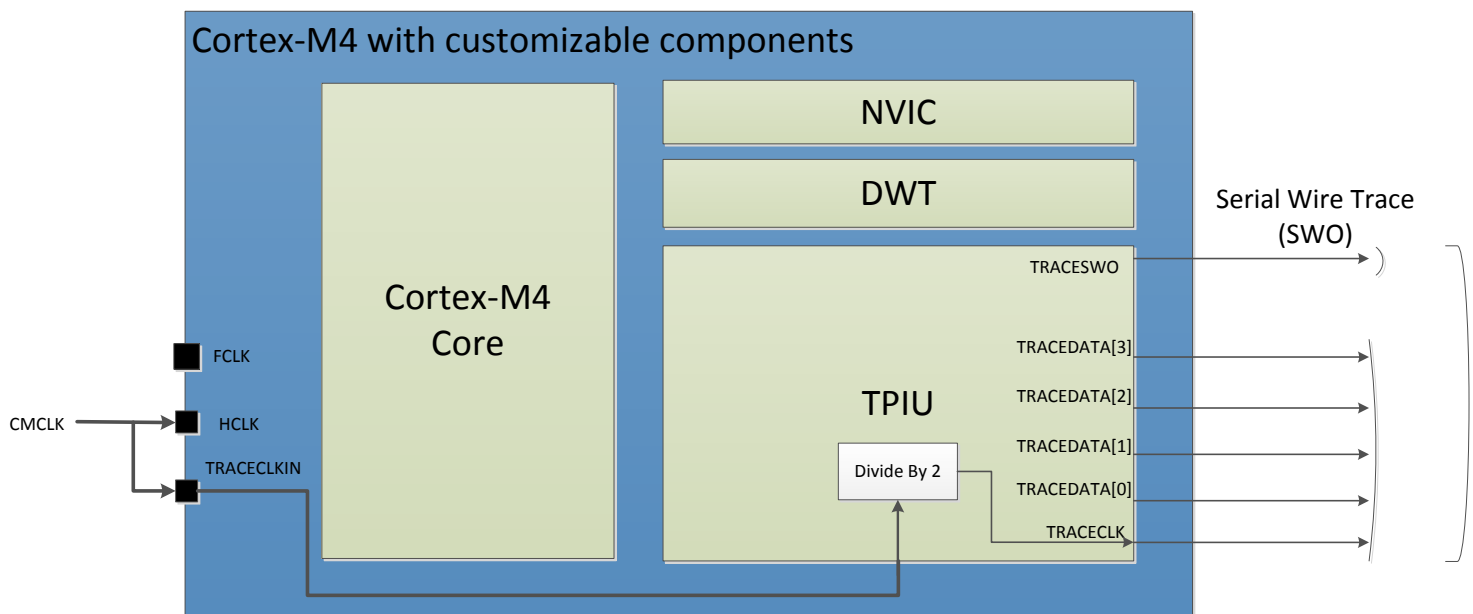
Figure 41-16. Debug Trace
