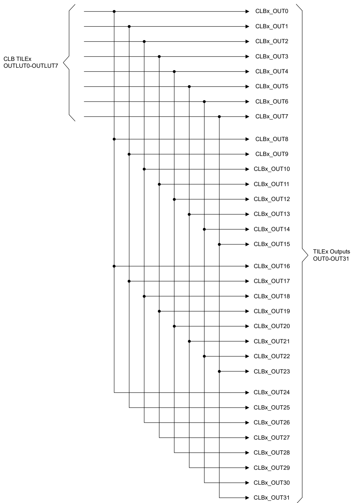
Figure 9-9. CLB Outputs
