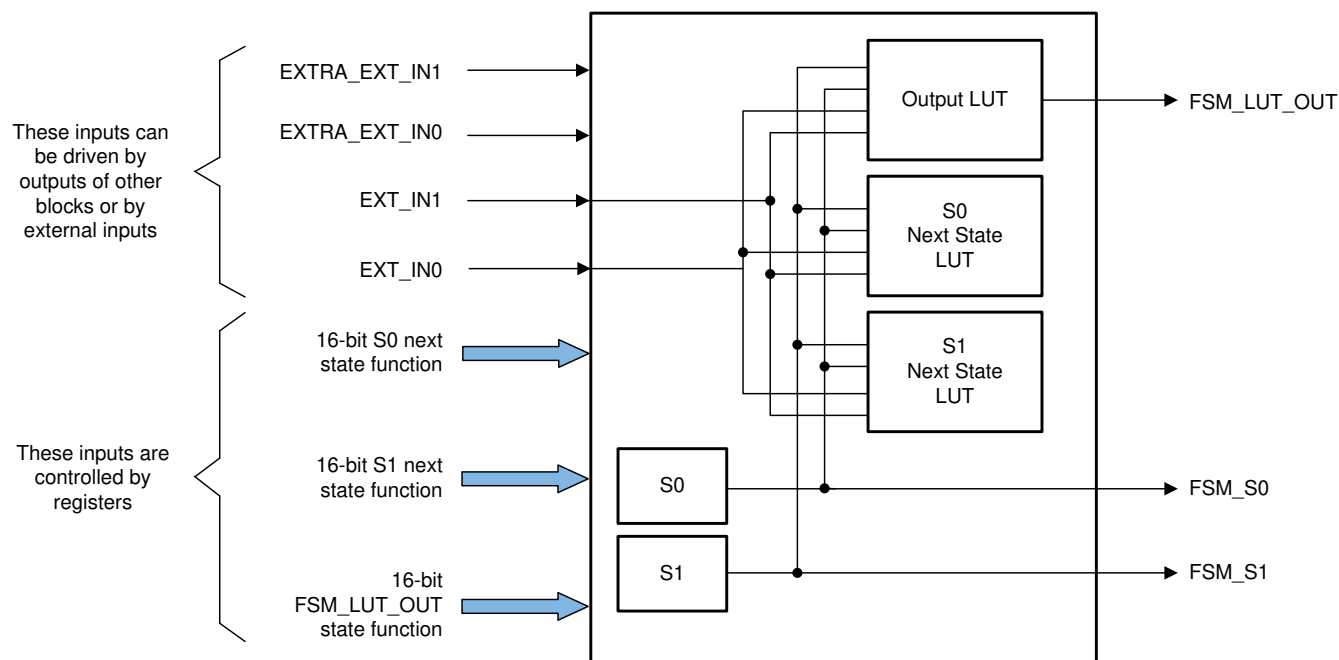
Figure 9-14. FSM Block
