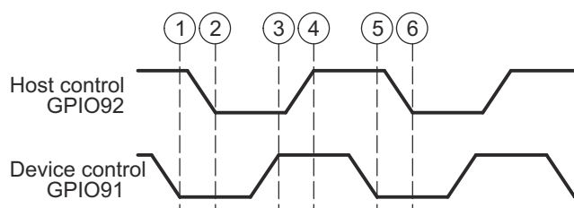
Figure 5-15. Parallel GPIO Bootloader Handshake Protocol
