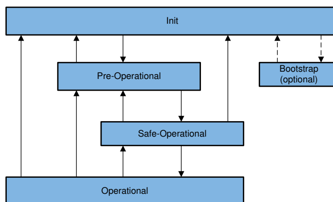
Figure 31-6. EtherCAT State Machine
