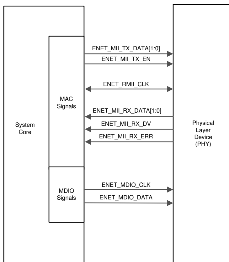
Figure 43-2. RMII Mode Signals
