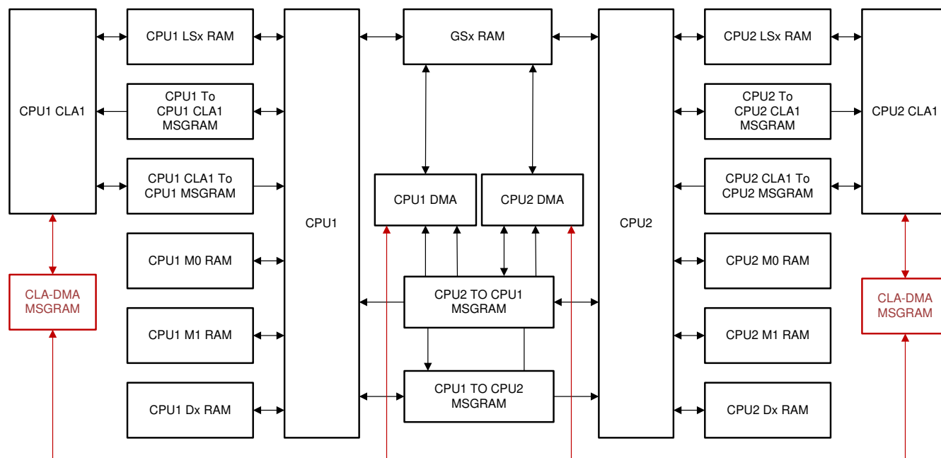
Figure 3-16. Memory Architecture
