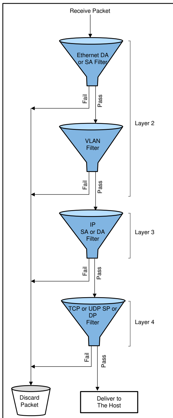
Figure 43-13. Packet Filtering
