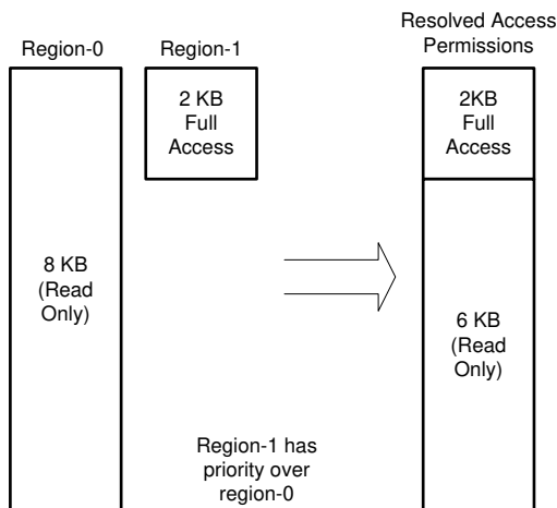
Figure 41-13. Overlapping Regions
