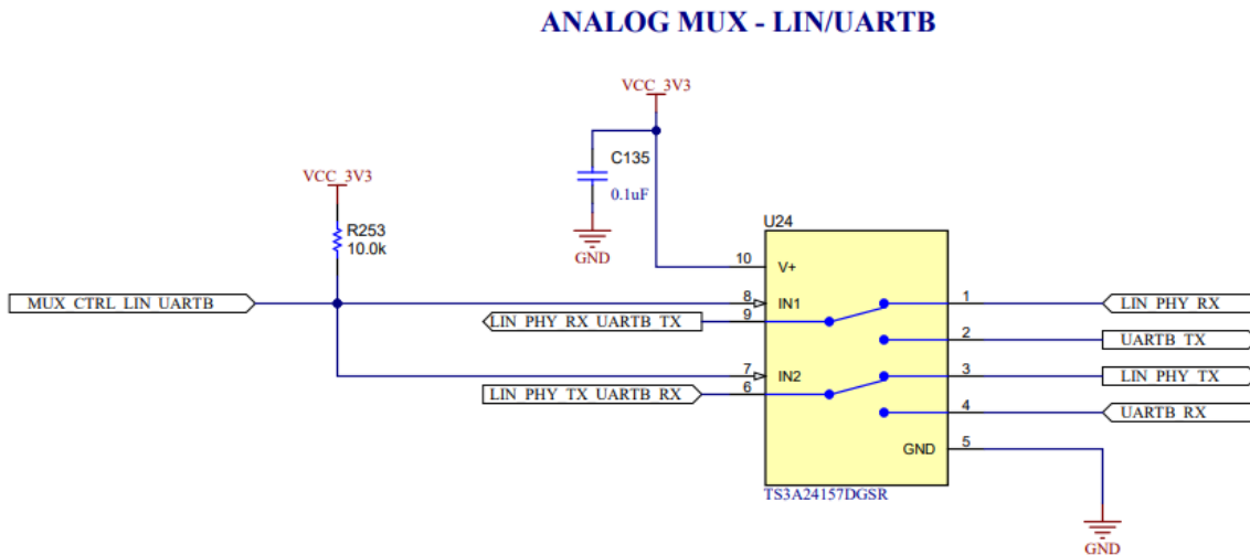
Figure 3-25. Analog Mux for the LIN PHY Switch
