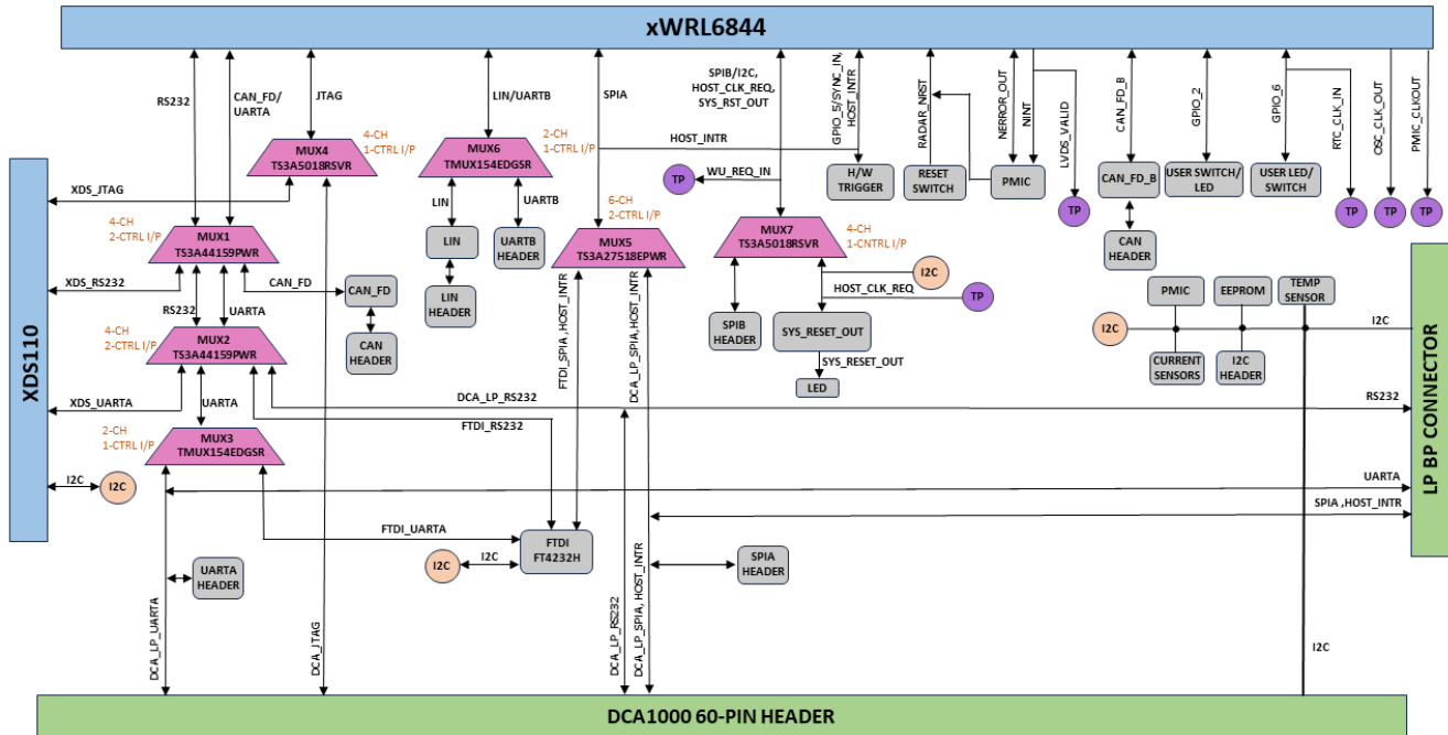
Figure 3-9. Functionality Muxing Options in the EVM
