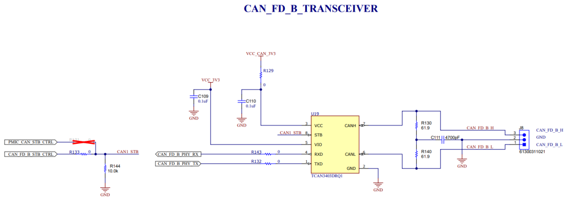
Figure 3-19. CAN-FD B Connector
