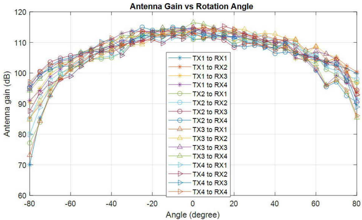
Figure 3-7. xWRL6844EVM Azimuth Antenna Radiation Pattern
