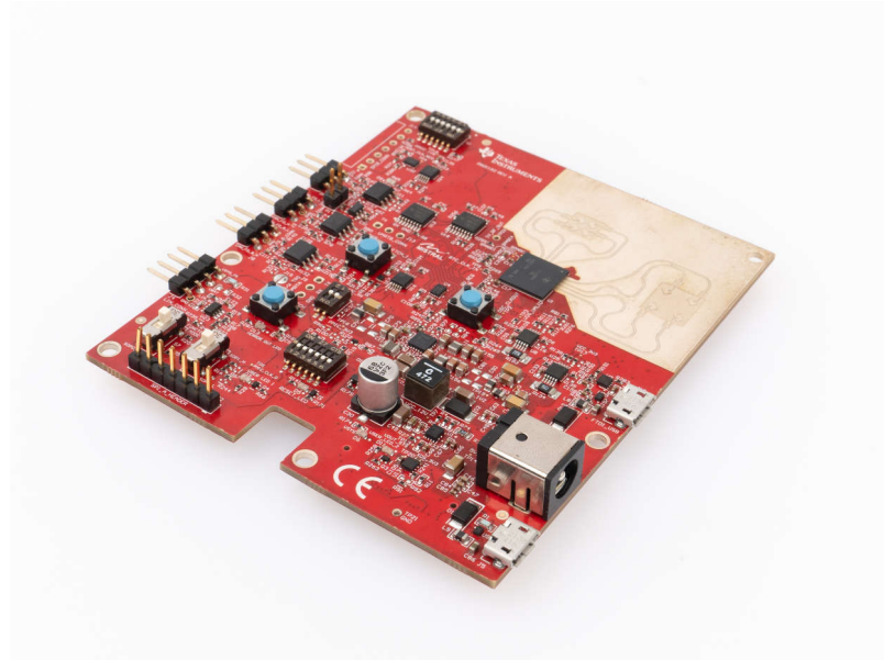
Figure 1-1. xWRL6844EVM
