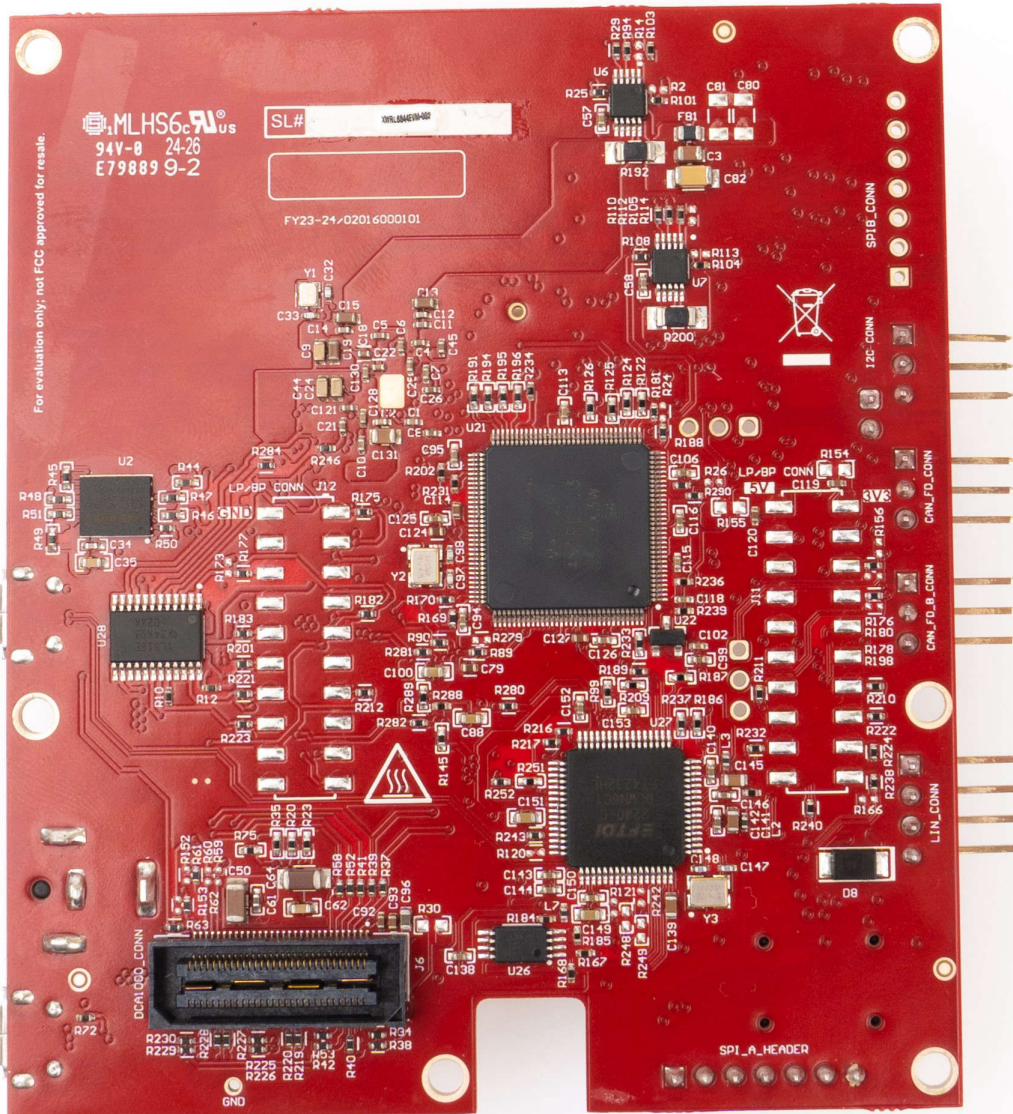
Figure 3-2. xWRL6844EVM (Bottom View)
