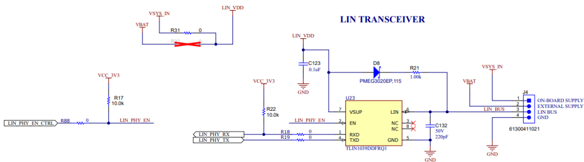
Figure 3-26. LIN PHY Interface
