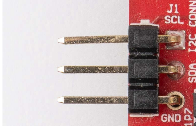
Figure 3-27. I2C Connector
