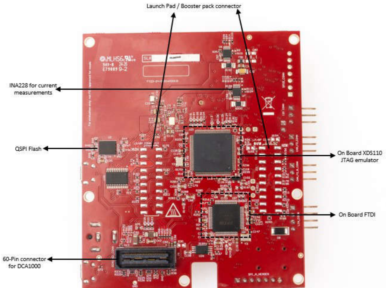
Figure 3-4. Salient Features of EVM (Bottom Side)
