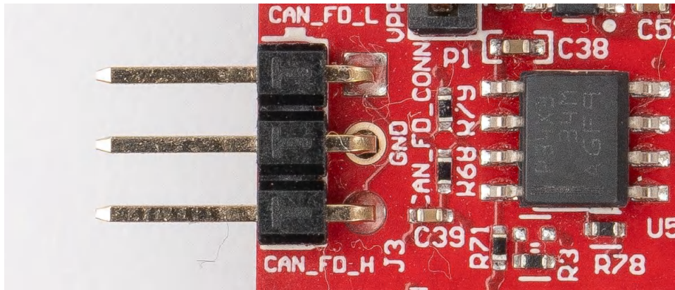
Figure 3-21. CAN-FD A Connector
