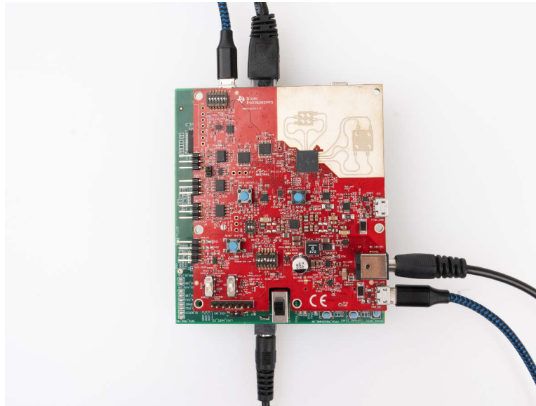
Figure 3-31. AWRL6844EVM for Raw Data Capture
