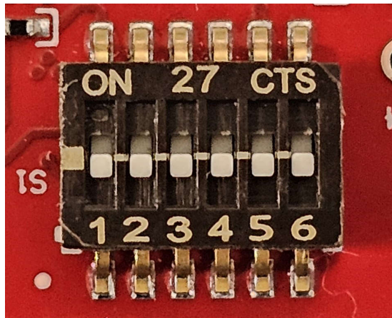
Figure 3-11. Slide Switch (S1)
