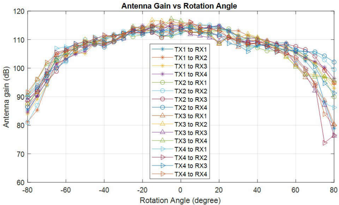
Figure 3-8. xWRL6844EVM Elevation Antenna Radiation Pattern
