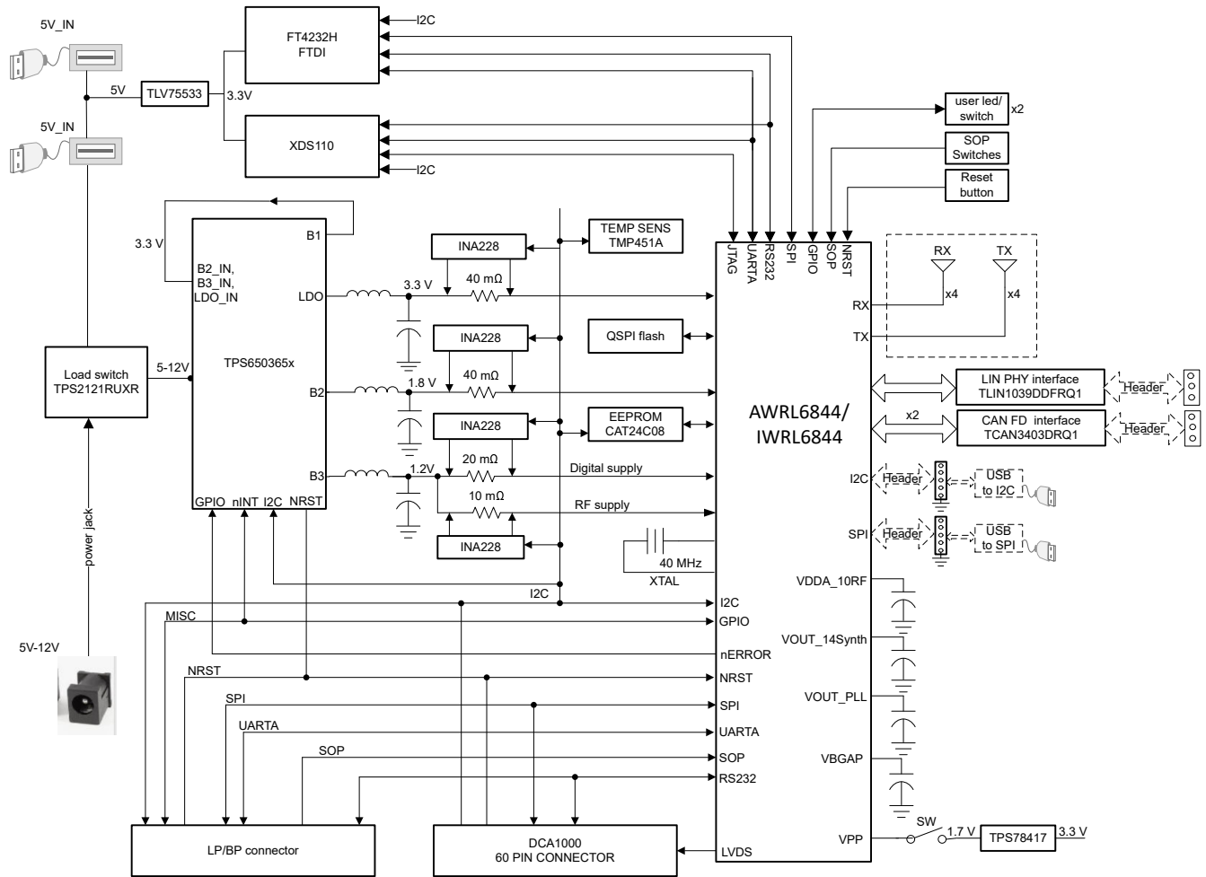
Figure 2-1. Functional Block Diagram
