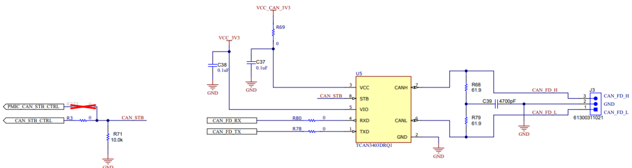
Figure 3-23. CAN-FD PHY Used in the EVM
