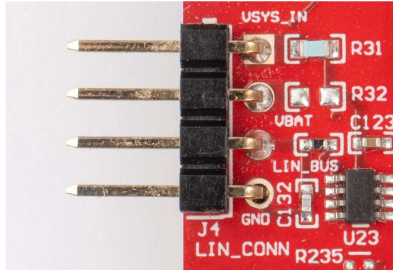
Figure 3-24. LIN Connector
