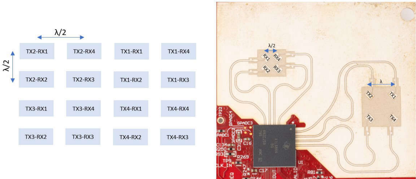
Figure 3-6. Antenna Virtual array with respect to TXs and RXs
