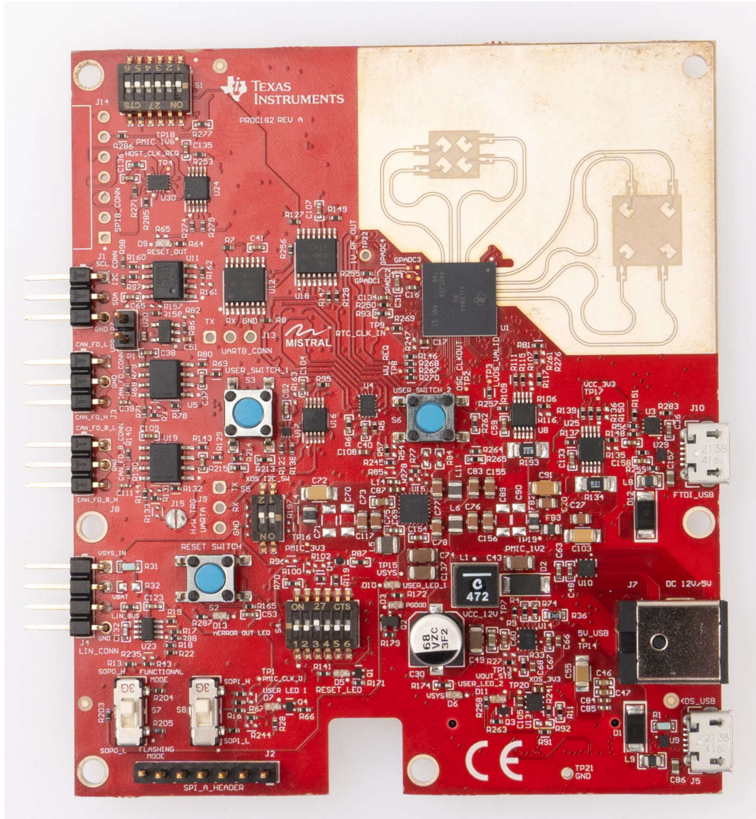
Figure 3-1. xWRL6844EVM (Top View)
