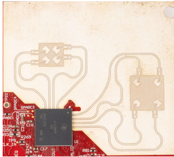
Figure 3-5. TX and Rx Antennas of the EVM
