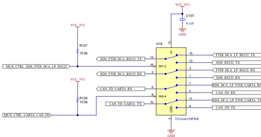
Figure 3-22. Analog Mux for the CAN PHY Switch
