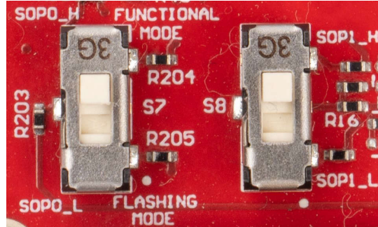
Figure 3-10. SOP switches (S7, S8)
