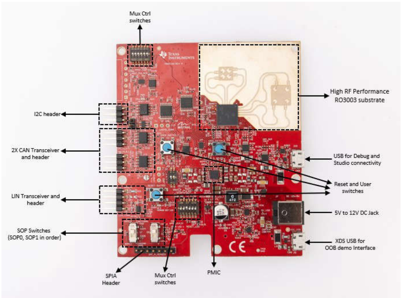
Figure 3-3. Salient Features of EVM (Top Side)
