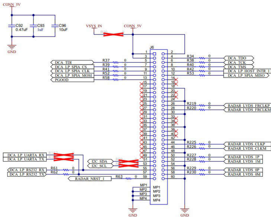
Figure 3-16. DCA1000 HD Connector Pins
