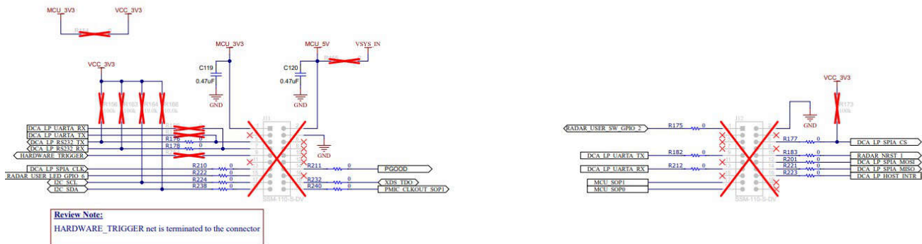
Figure 3-18. LP-BP connector Pins
