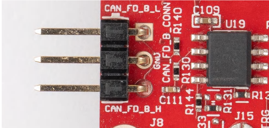
Figure 3-19. CAN-FD B Connector
