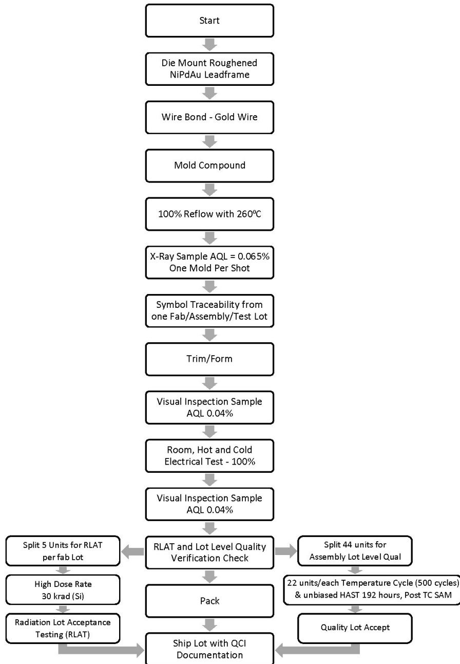
Figure 2-1. SN54SC4T02-SEP Space Enhanced Plastic Production Flow Chart
