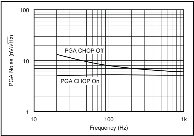
Figure 30. PGA Noise
