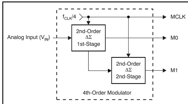
Figure 31. Fourth-Order Modulator
