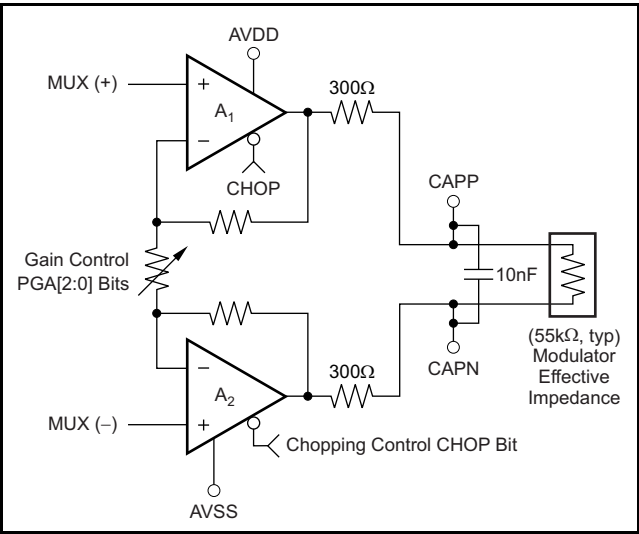
Figure 29. PGA Block Diagram
