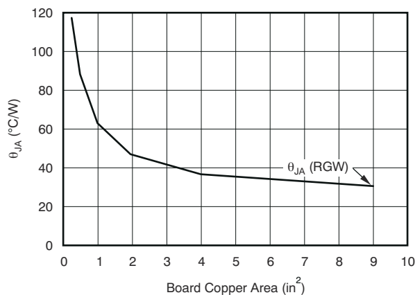
Figure 8-1. \theta_{JA} vs Board Size
