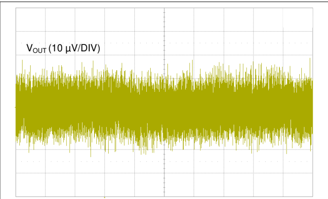
Figure 7-3. Output Noise Voltage, 10 Hz to 100 kHz (10 ms/DIV)
