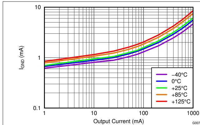
Figure 5-7. Ground Current vs Output Current
