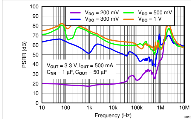
Figure 5-15. Power-Supply Rejection Ratio vs Dropout
