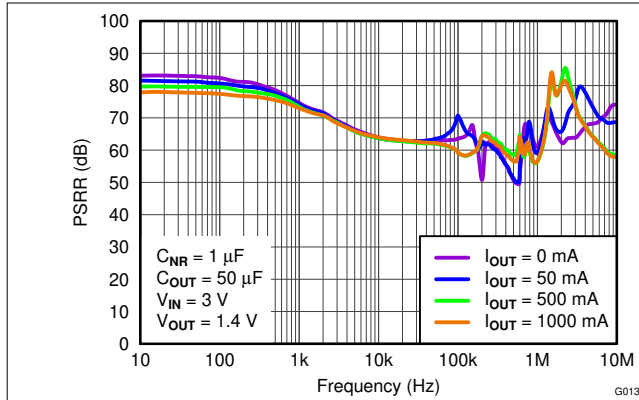
Figure 5-13. Power-Supply Rejection Ratio vs I_O
