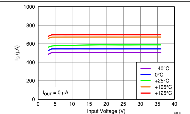
Figure 5-6. Quiescent Current vs Input Voltage
