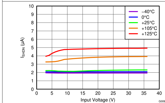
Figure 5-9. Shutdown Current vs Input Voltage
