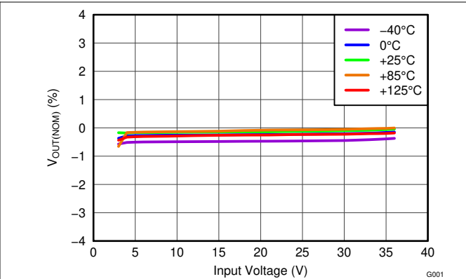
Figure 5-2. Line Regulation
