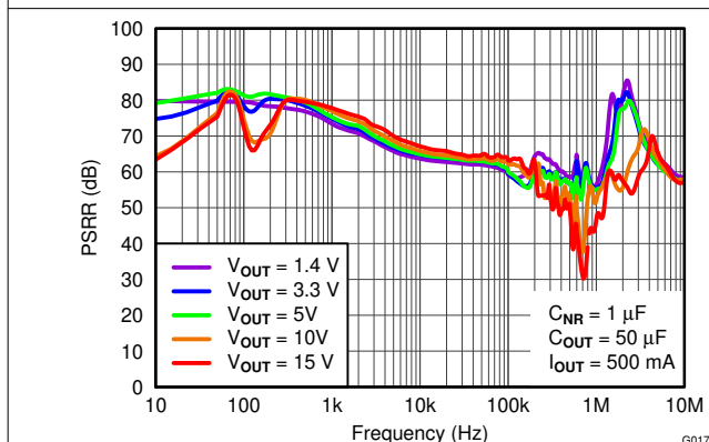
Figure 5-17. Power-Supply Rejection Ratio vs Output Voltage
