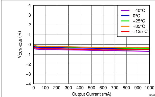
Figure 5-3. Load Regulation
