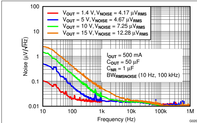
Figure 5-1. Noise vs Output Voltage
