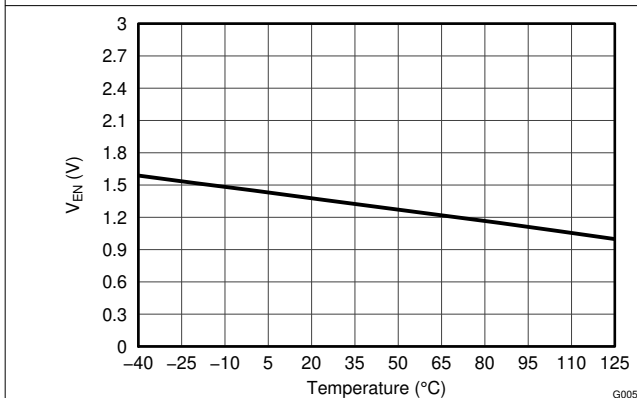
Figure 5-5. Enable Voltage Threshold vs Temperature
