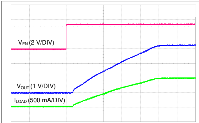
Figure 7-2. Startup with EN Pin rising (10 ms/DIV)
