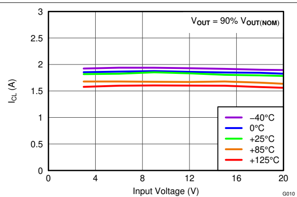
Figure 5-10. Current Limit vs Input Voltage
