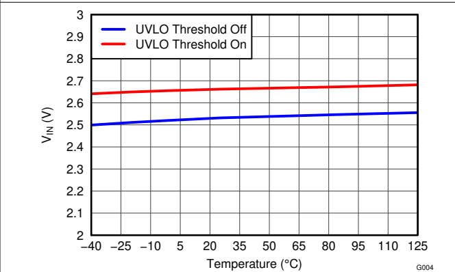
Figure 5-4. UVLO Threshold vs Temperature
