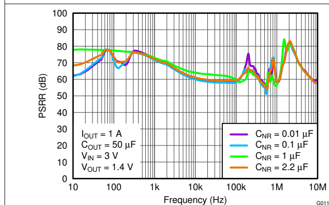
Figure 5-11. Power-Supply Rejection Ratio vs C_{\text{NR}}
