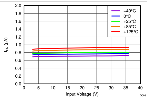
Figure 5-8. Enable Current vs Input Voltage
