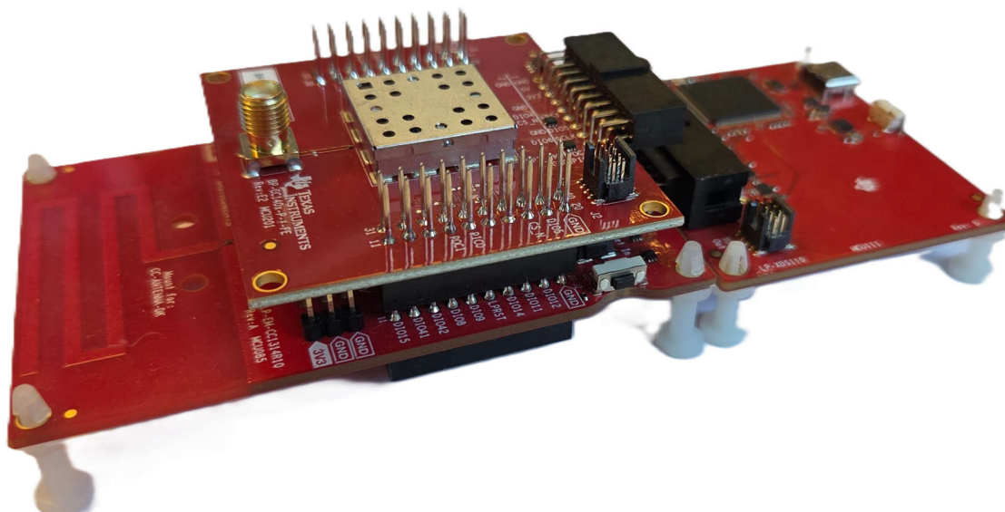
Figure 2-2. CC1402P BoosterPack Stacked on Top of the CC1314R10 LaunchPad (+ LP-XDS110)
