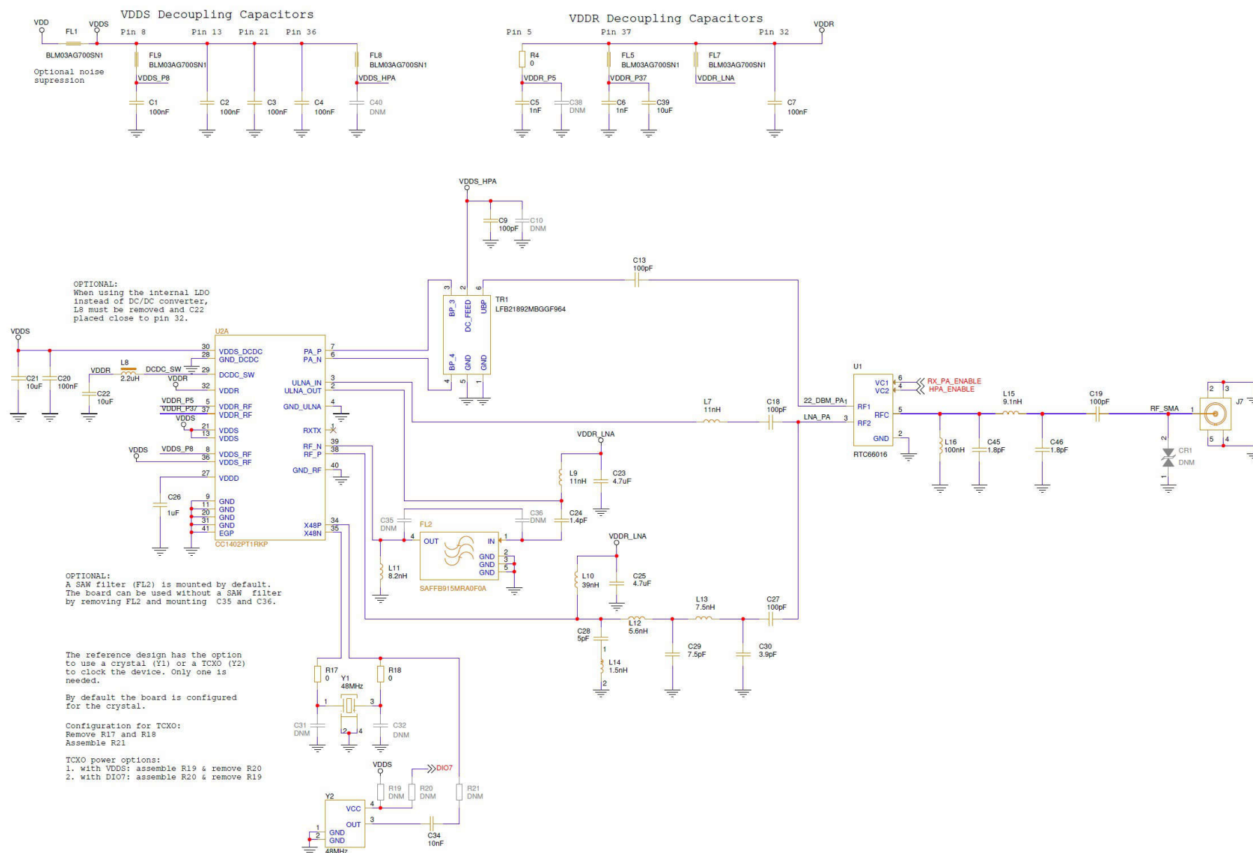
Figure 4-4. BP-CC1402P-9-FE Schematics Page 1
