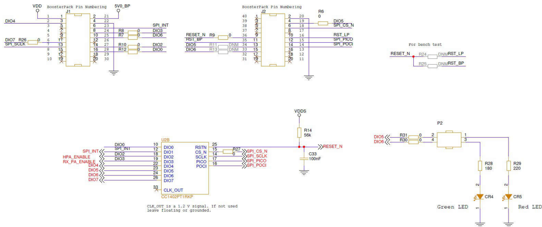
Figure 4-2. BP-CC1402P-8-FE Schematics Page 2
