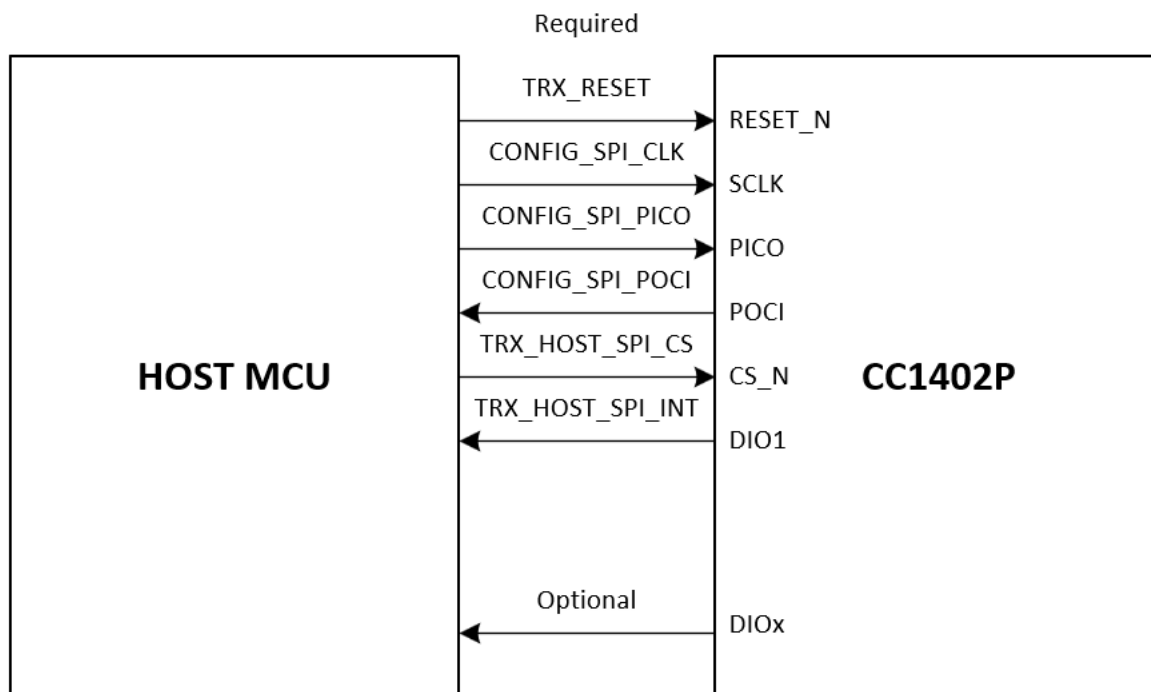
Figure 2-5. Connections between the CC1402P and the Host MCU
