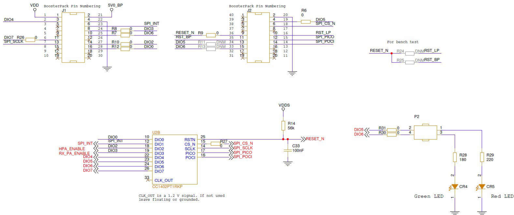
Figure 4-5. BP-CC1402P-9-FE Schematics Page 2
