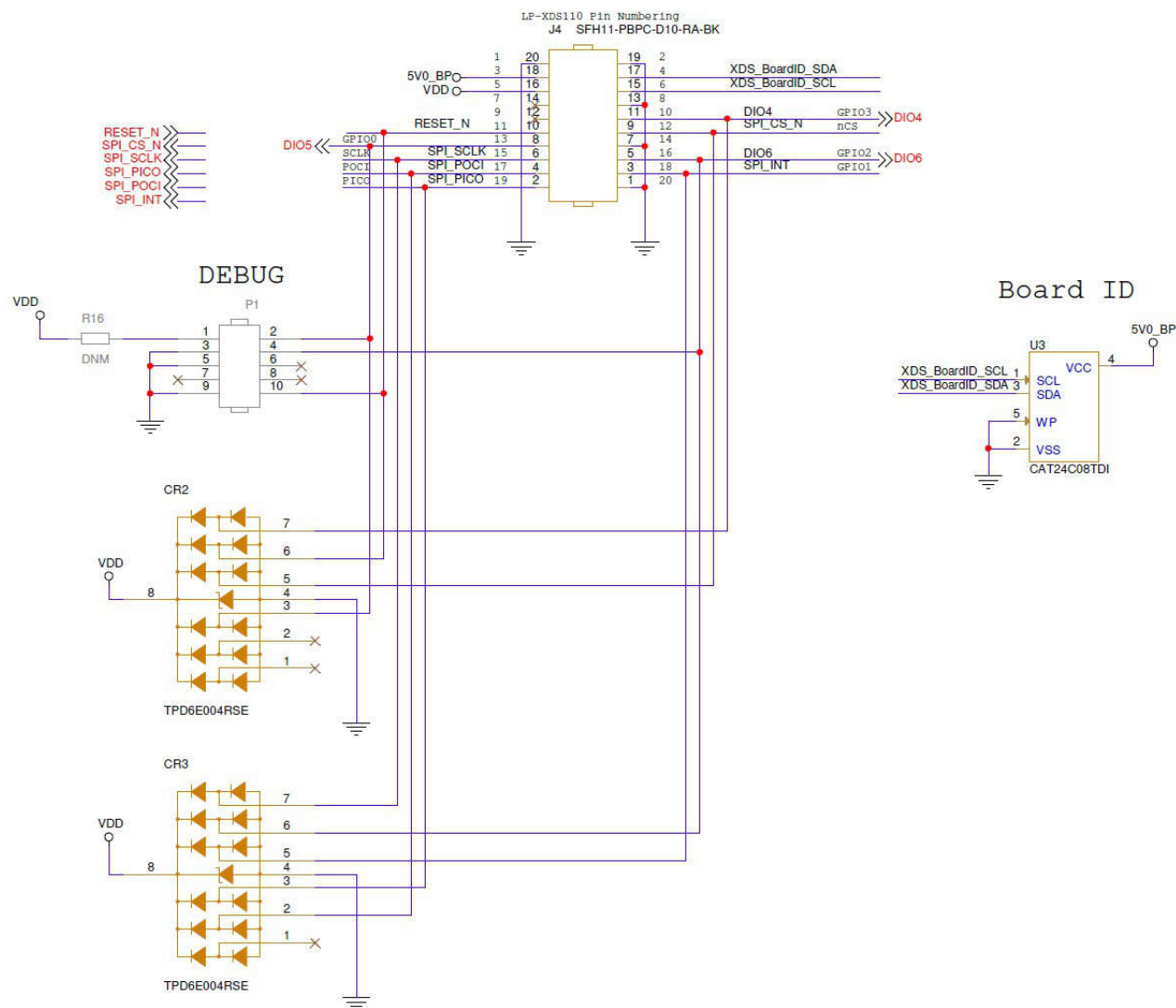
Figure 4-3. BP-CC1402P-8-FE Schematics Page 3
