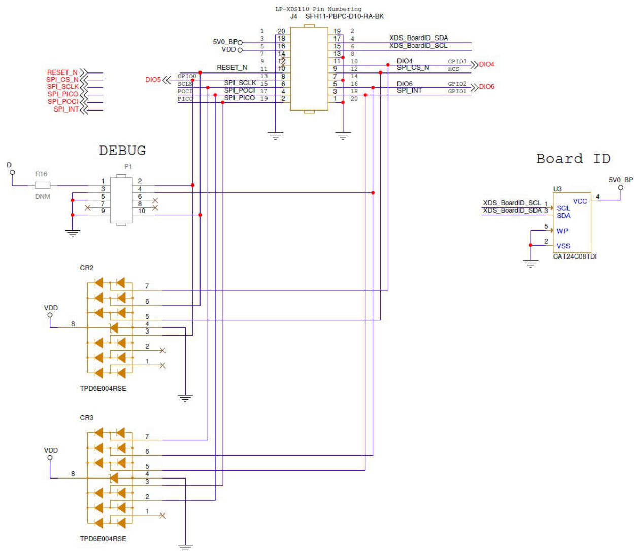
Figure 4-6. BP-CC1402P-9-FE Schematics Page 3
