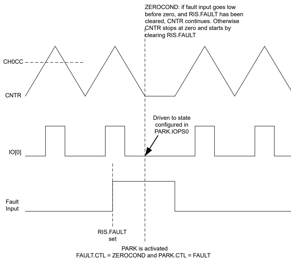
Figure 12-11. Fault and Park—Zero Condition
