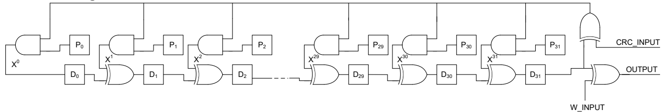
Figure 28-2. LFSR Logic
