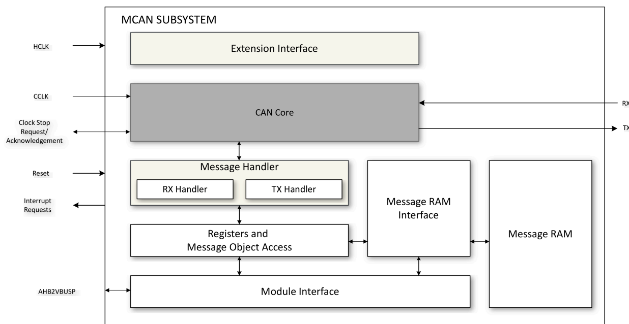
Figure 27-1. MCAN SUBSYSTEM
