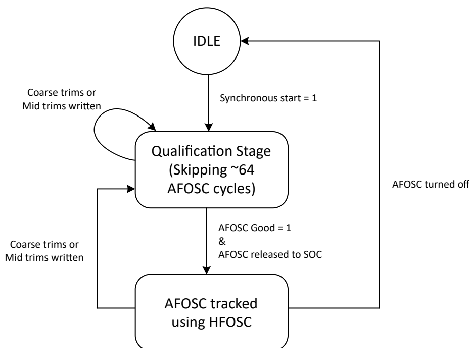
Figure 6-8. AFOSC Qualification
