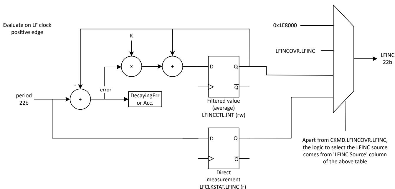
Figure 6-5. Block Diagram
