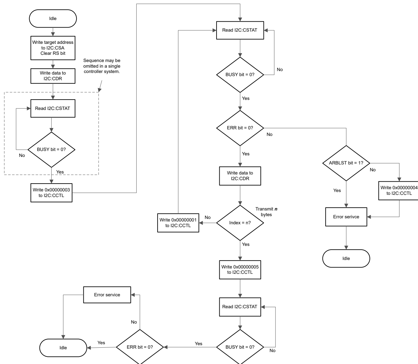
Figure 25-9. Controller Transmit with Repeated Start Condition
