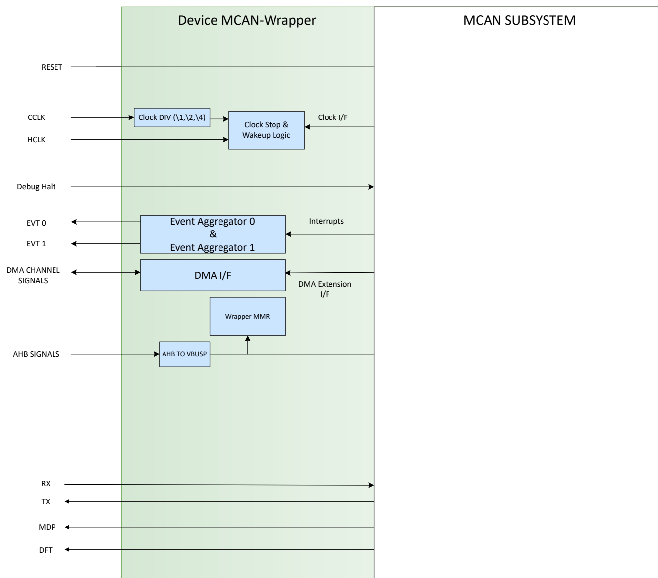
Figure 27-14. MCAN Wrapper
