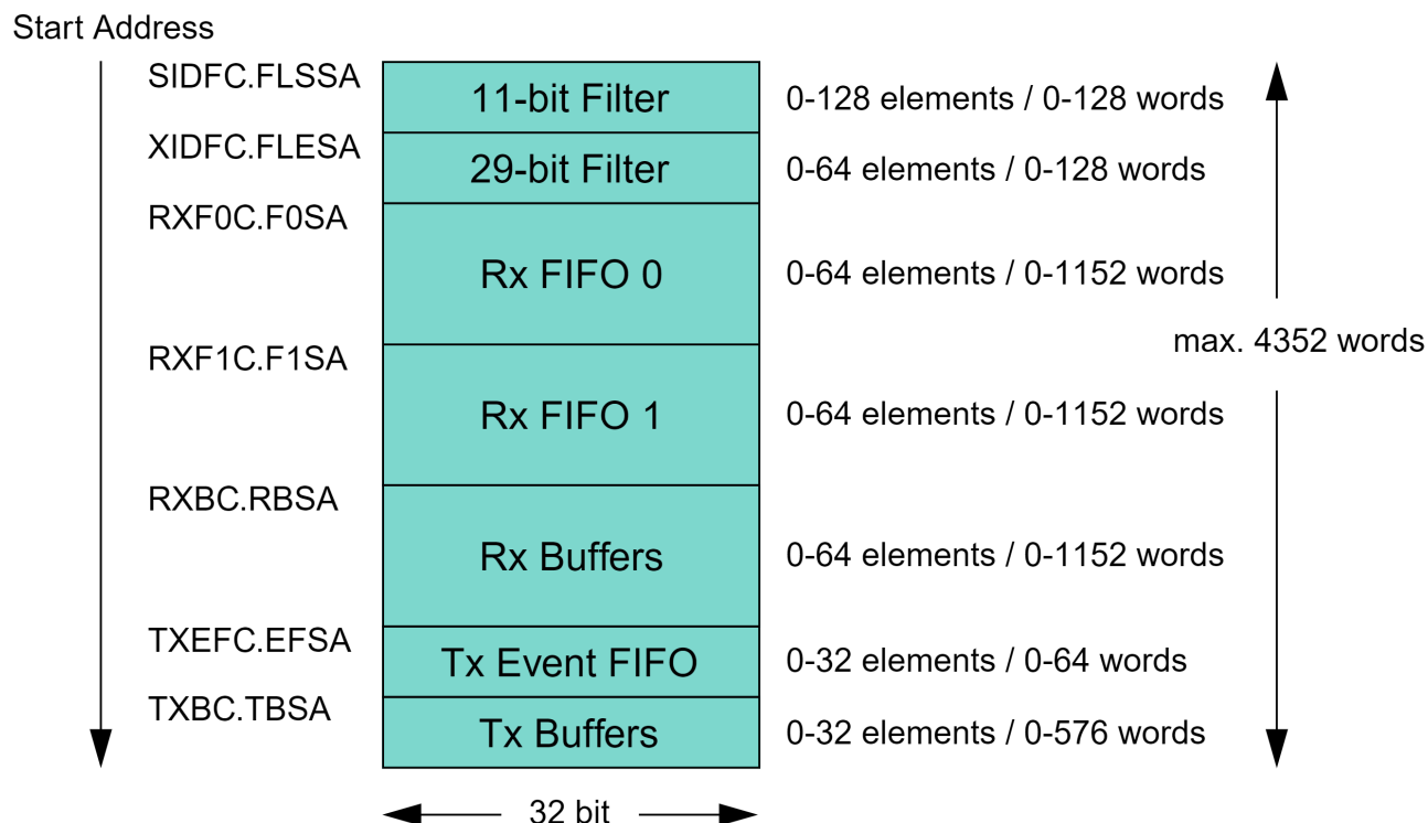
Figure 27-13. MCAN_Message_RAM_Configuration
