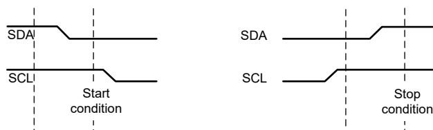
Figure 25-3. Start and Stop Conditions
