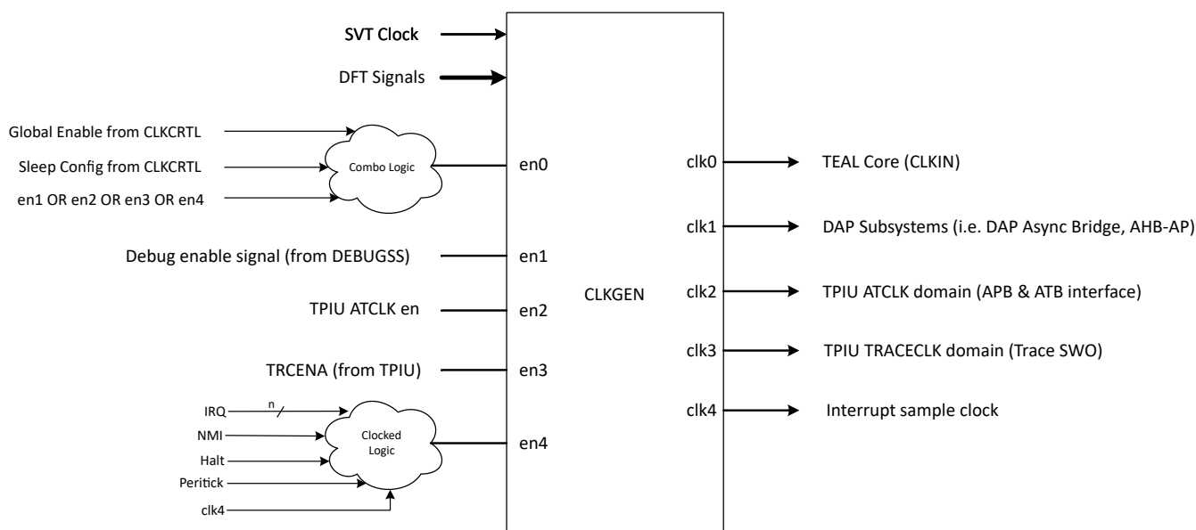
Figure 2-2. CPUSS Clock Control
