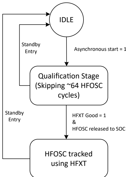
Figure 6-6. HFOSC Qualification
