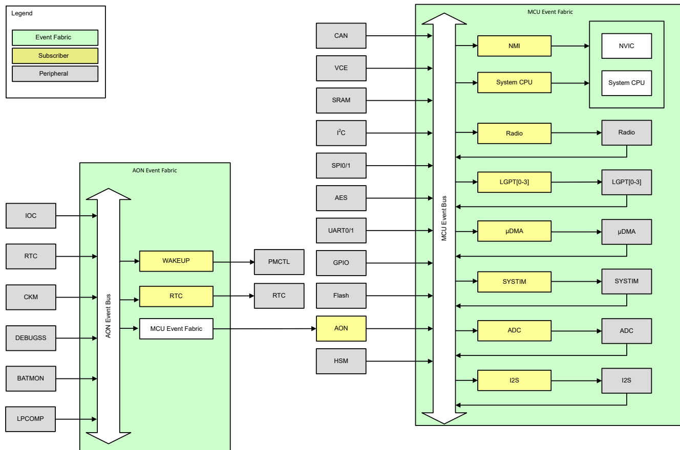
Figure 4-2. Event Fabric Overview (Simplified)
