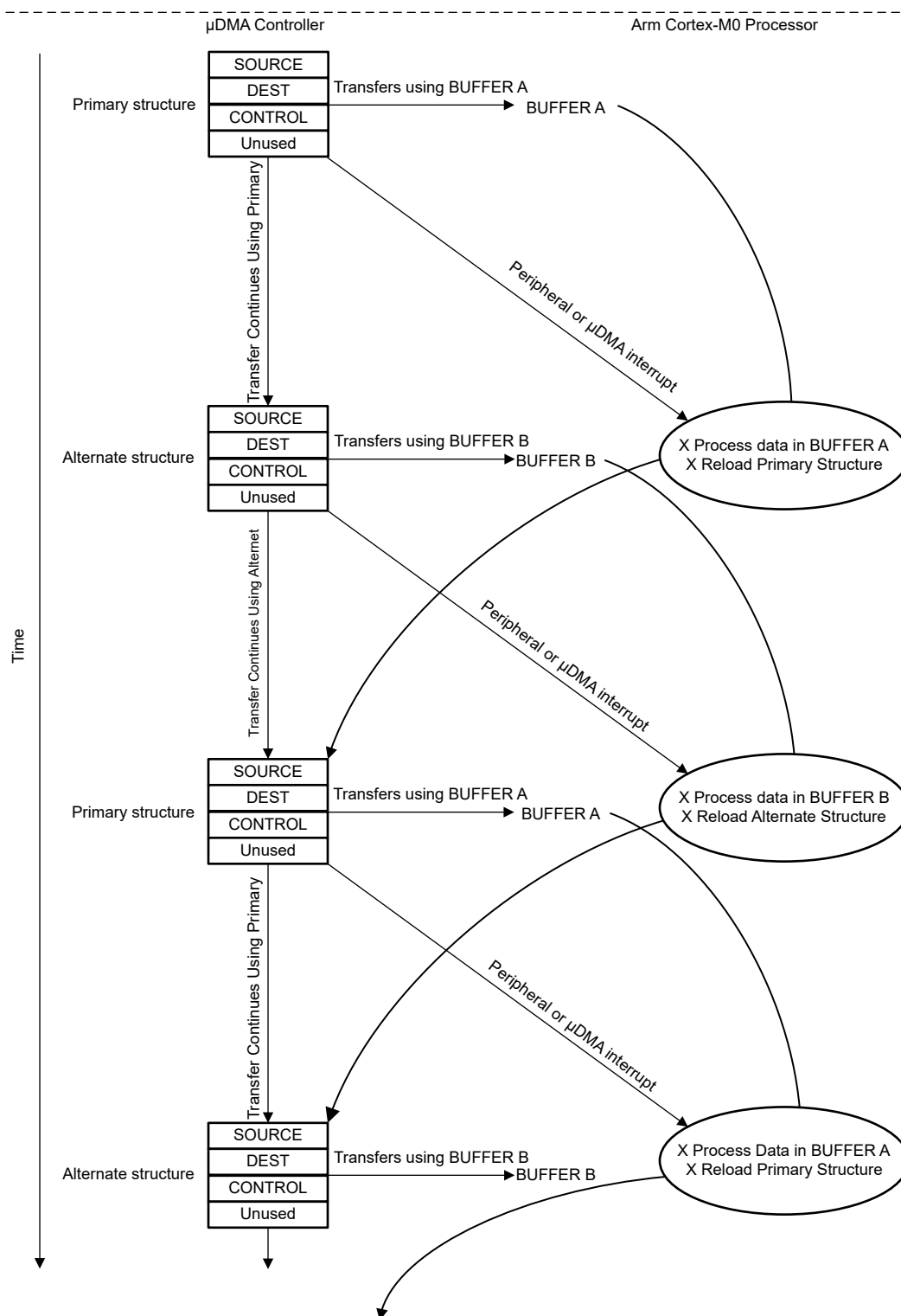
Figure 19-2. Example of Ping-Pong \mu DMA Transaction
