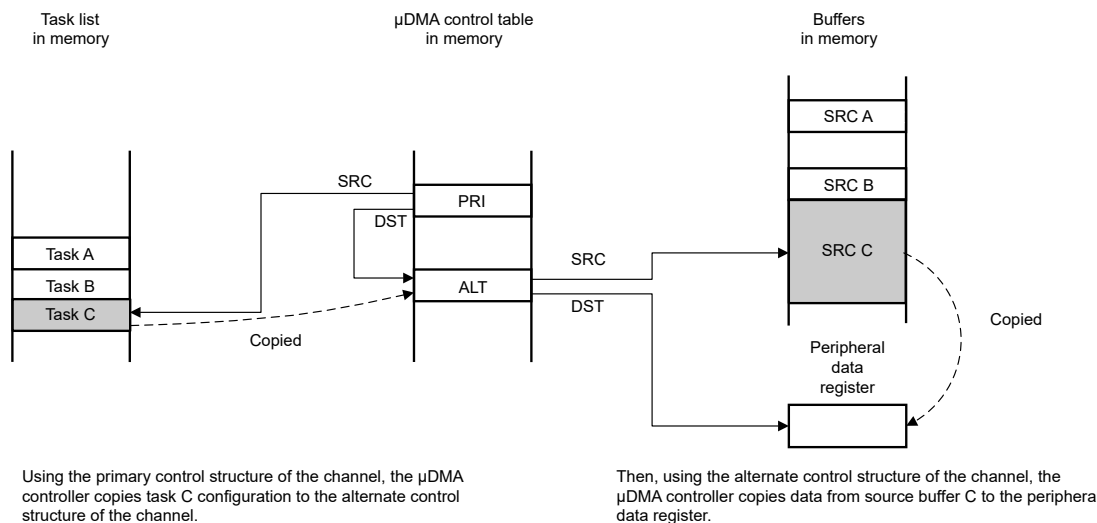
Figure 19-3. Memory Scatter-Gather, Setup, and Configuration
