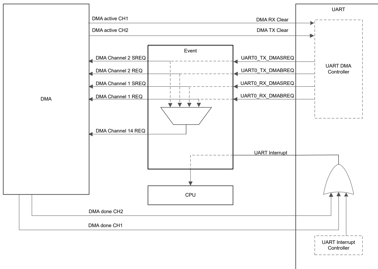
Figure 23-4. \mu DMA Example
