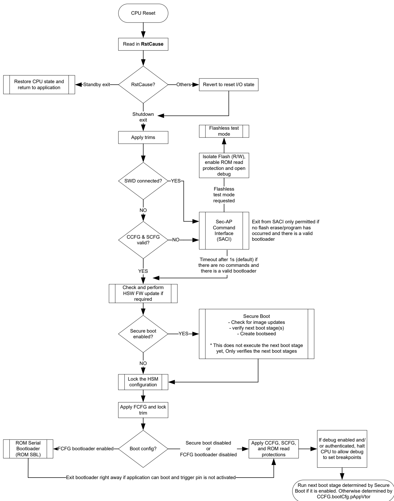
Figure 9-1. Boot Flow
