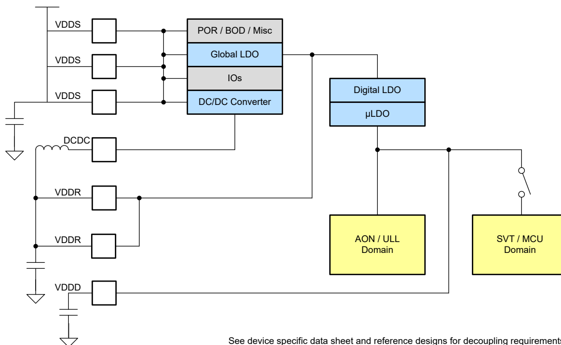
Figure 1-2. Supply System
