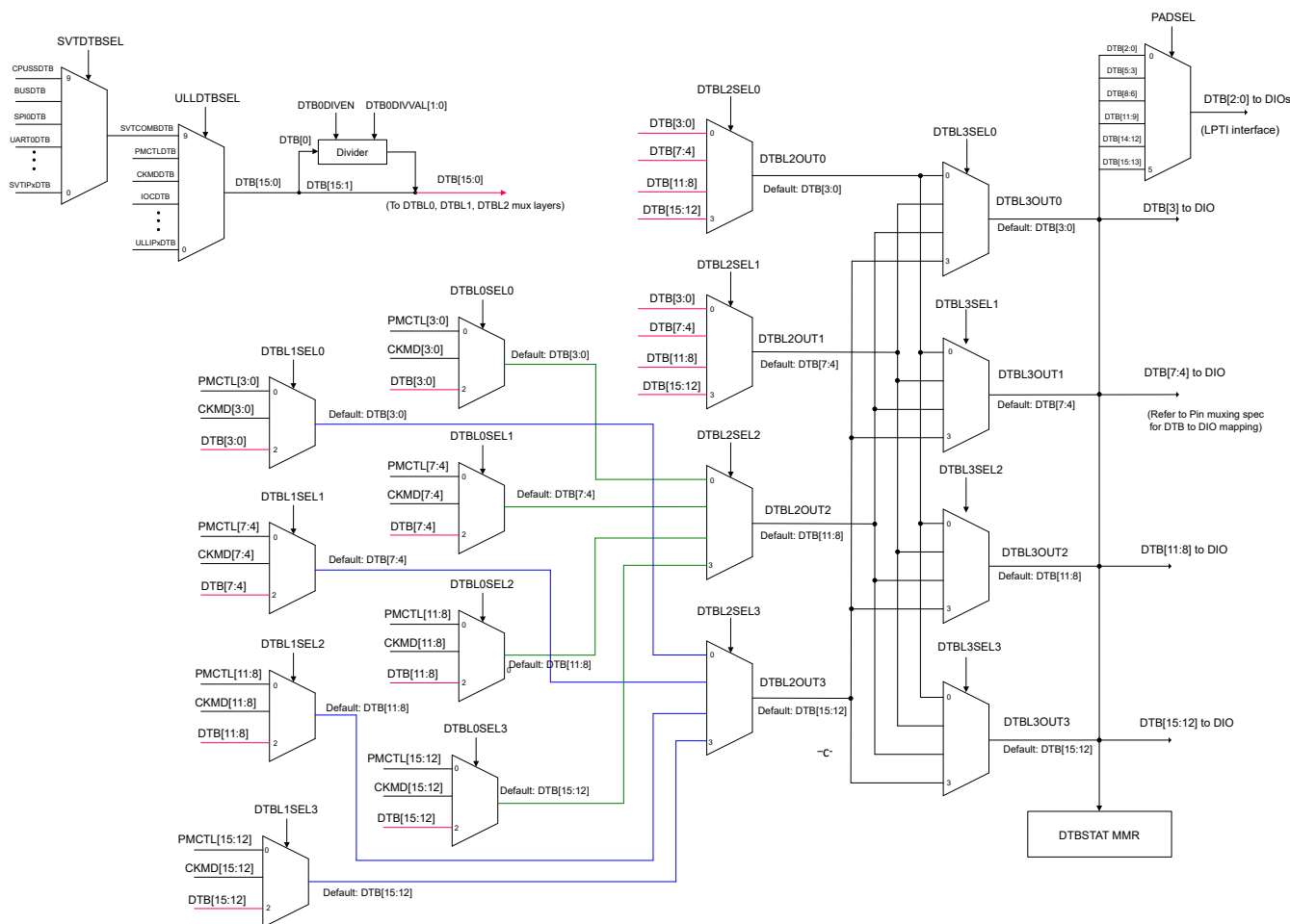
Figure 22-2. DTB Multiplexing
