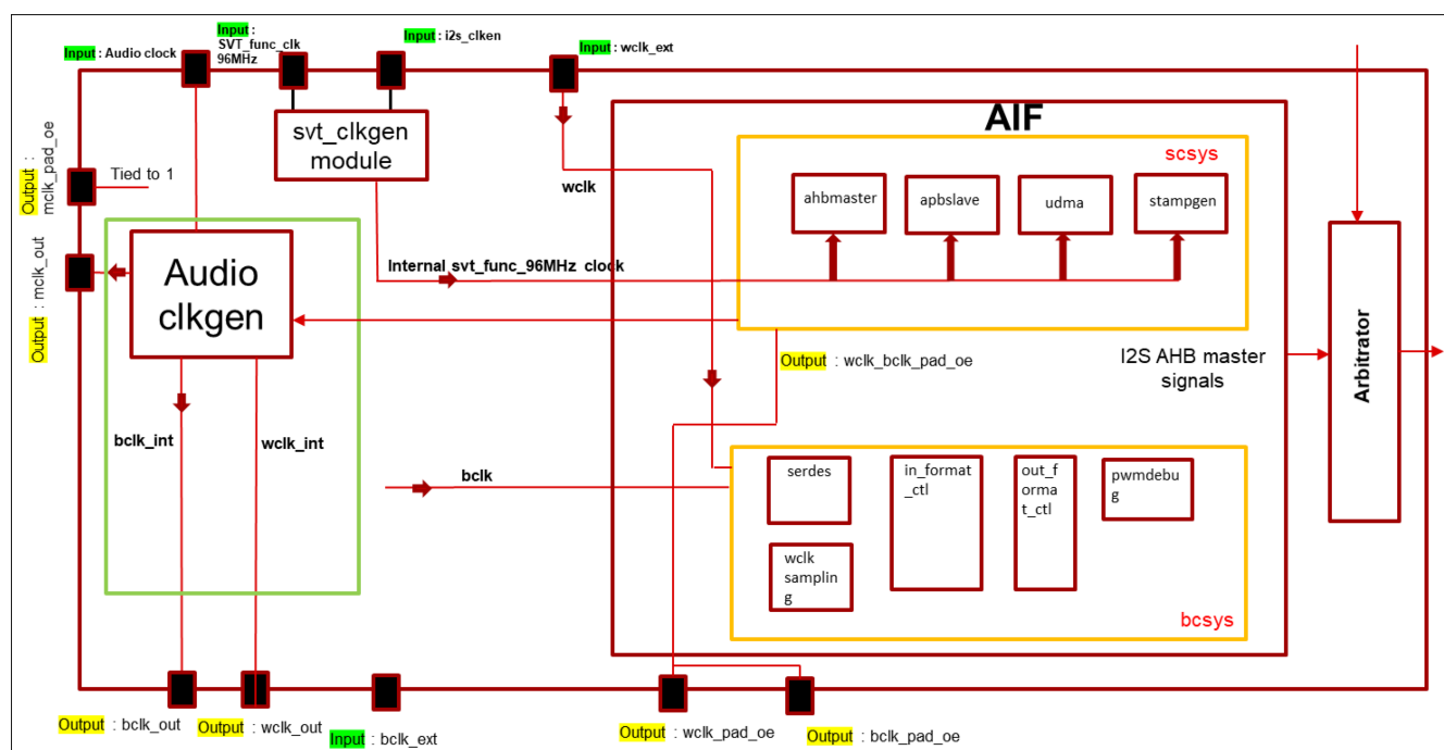
Figure 26-2. I 2 S Clock Architecture
