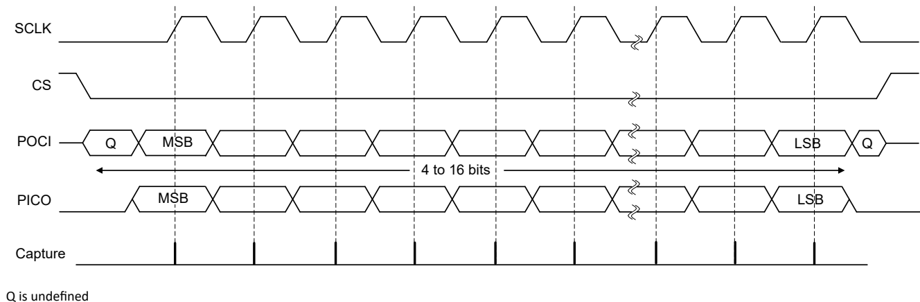
Figure 24-2. Motorola SPI Frame Format with SPO=0 and SPH=0
