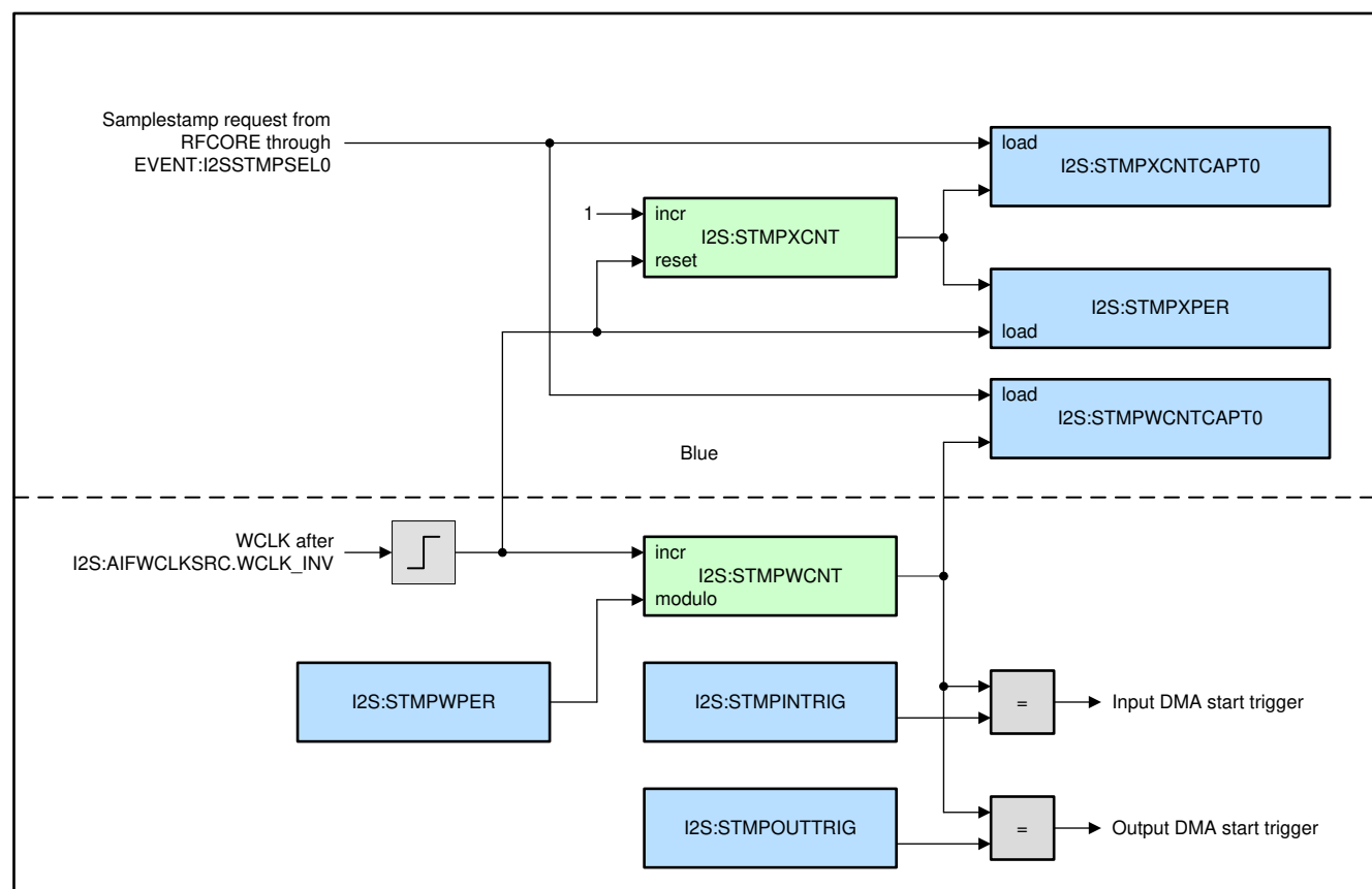
Figure 26-12. Samplestamp Generator
