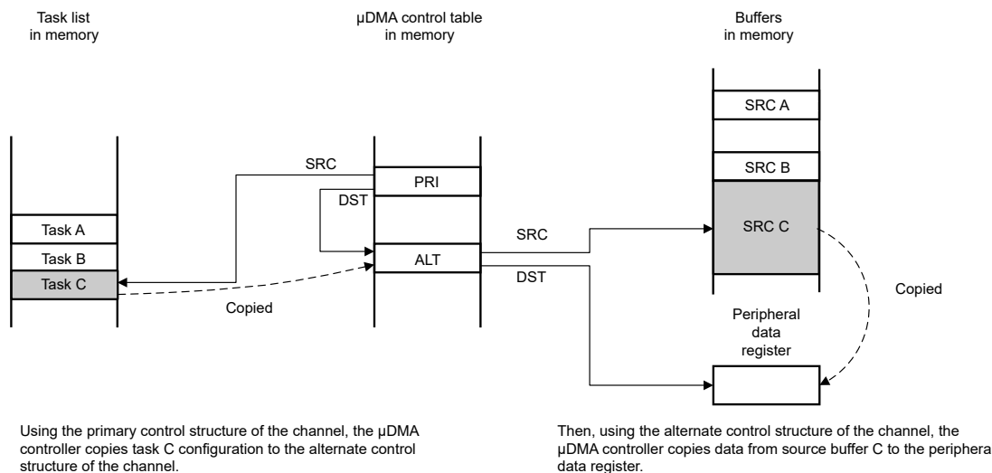
Figure 19-6. Peripheral Scatter-Gather, \mu DMA Copy Sequence
