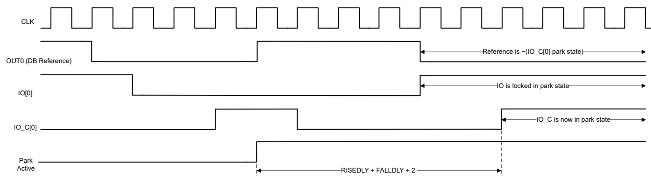
Figure 12-14. Deadband Switch to Equal Park States
