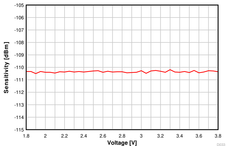
Figure 8-15. Sensitivity vs. Supply Voltage (VDD S ) (50 kbps, 868.3 MHz)
