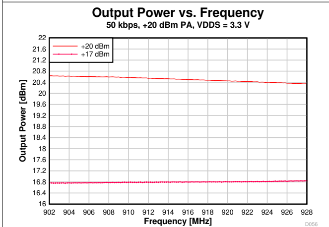
Figure 7-49. Output Power vs. Frequency (50 kbps, 915 MHz, VDDS = 3.3 V)
