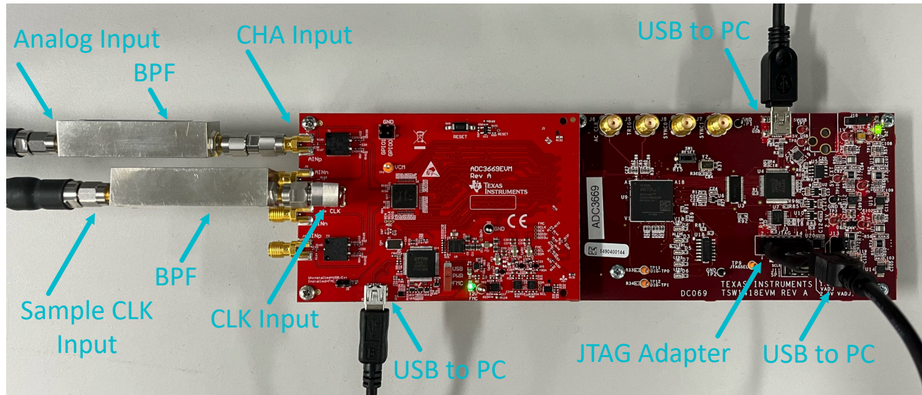
Figure 2-2. Assembled setup of the ADC3669EVM
