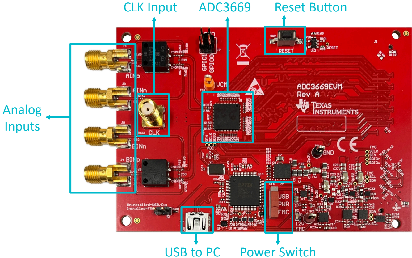
Figure 2-1. ADC3669EVM Features.
