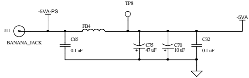
Analog Supply (+/-5volts) for Ext. Components
