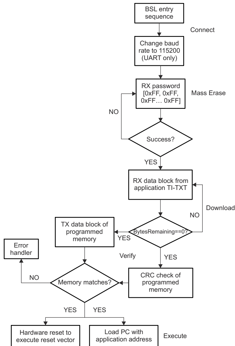
Figure 5-1. Flowchart
