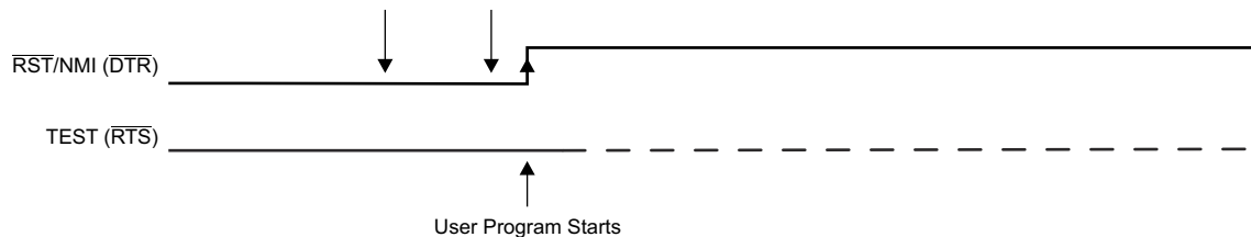
Figure 3-1. Standard RESET Sequence
