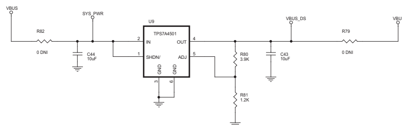
Figure 6. TUSB1064RNQ EVM Power
