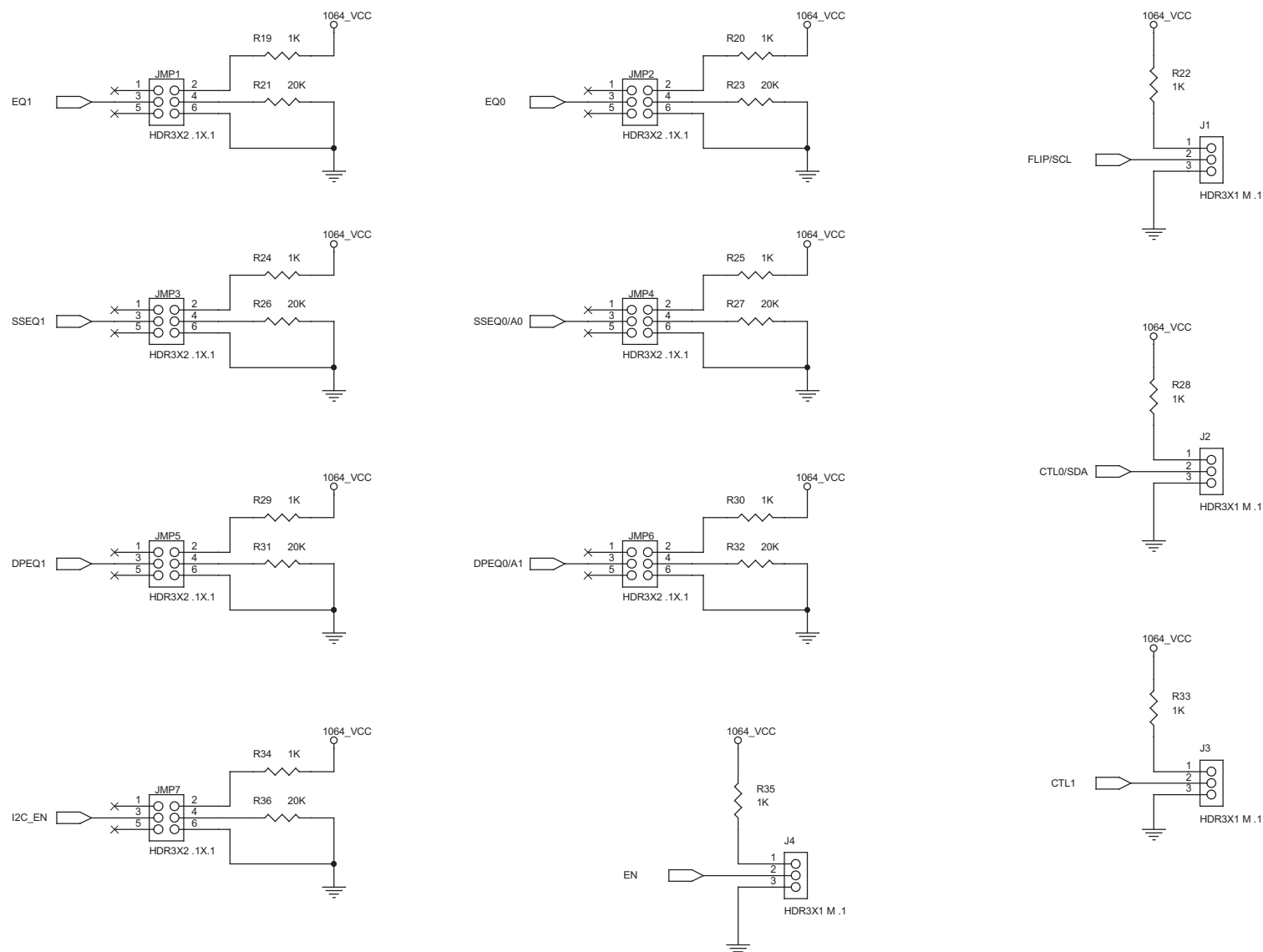
Figure 4. TUSB1064RNQ EVM Configuration Pins
