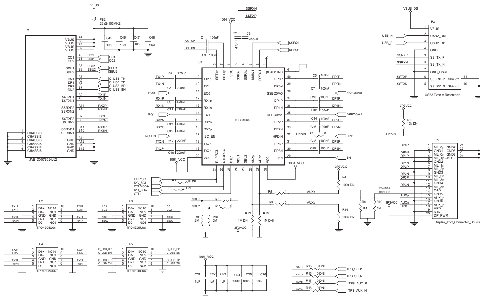
Figure 3. TUSB1064RNQ EVM Main Schematic
