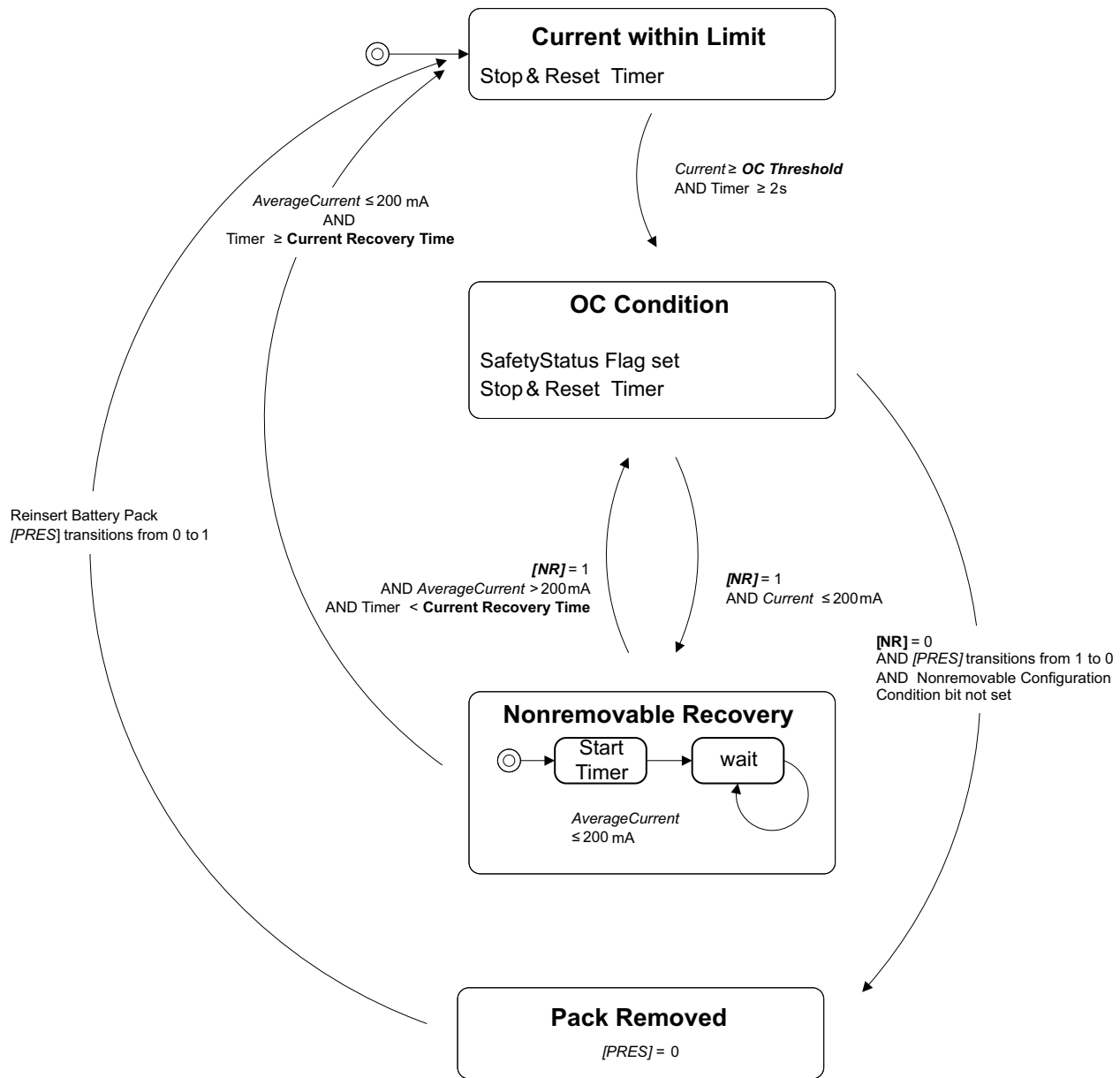
Figure 2-2. OC Protection
