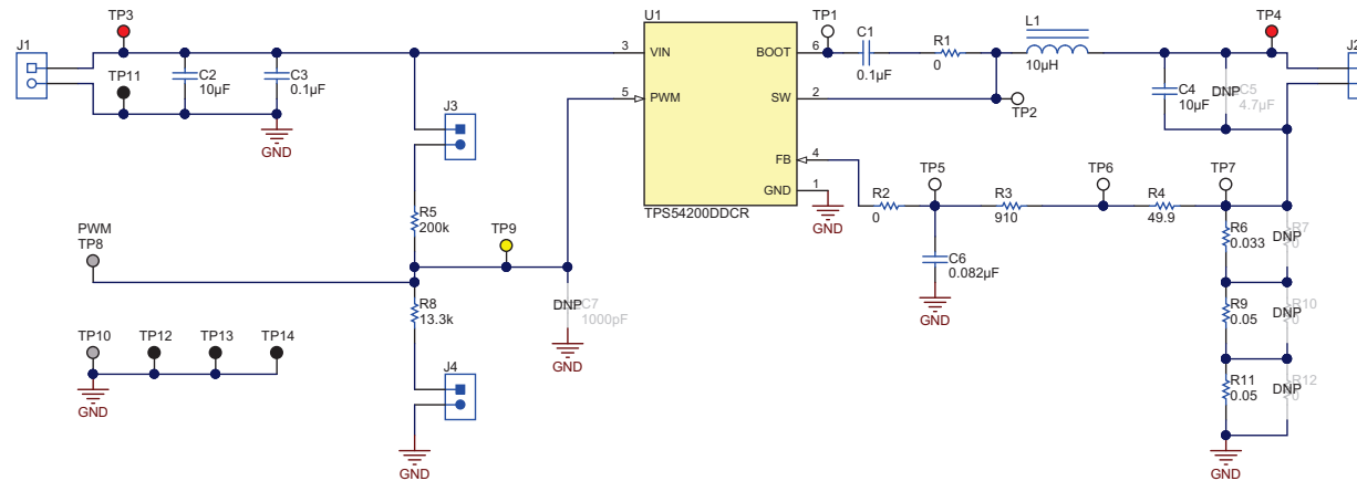
Figure 11. TPS54200EVM-818 Schematic
