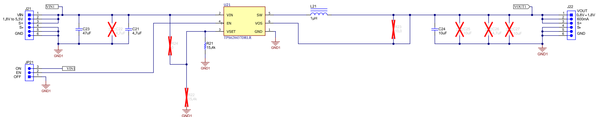
Figure 4-2. TPS628437 Schematic
