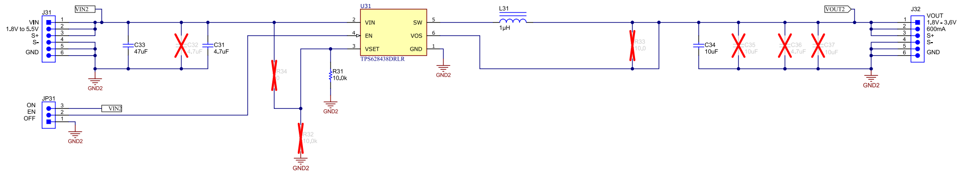
Figure 4-3. TPS628438 Schematic
