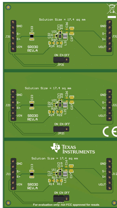
TP62843678EVM-030 Hardware Image (Top View)
