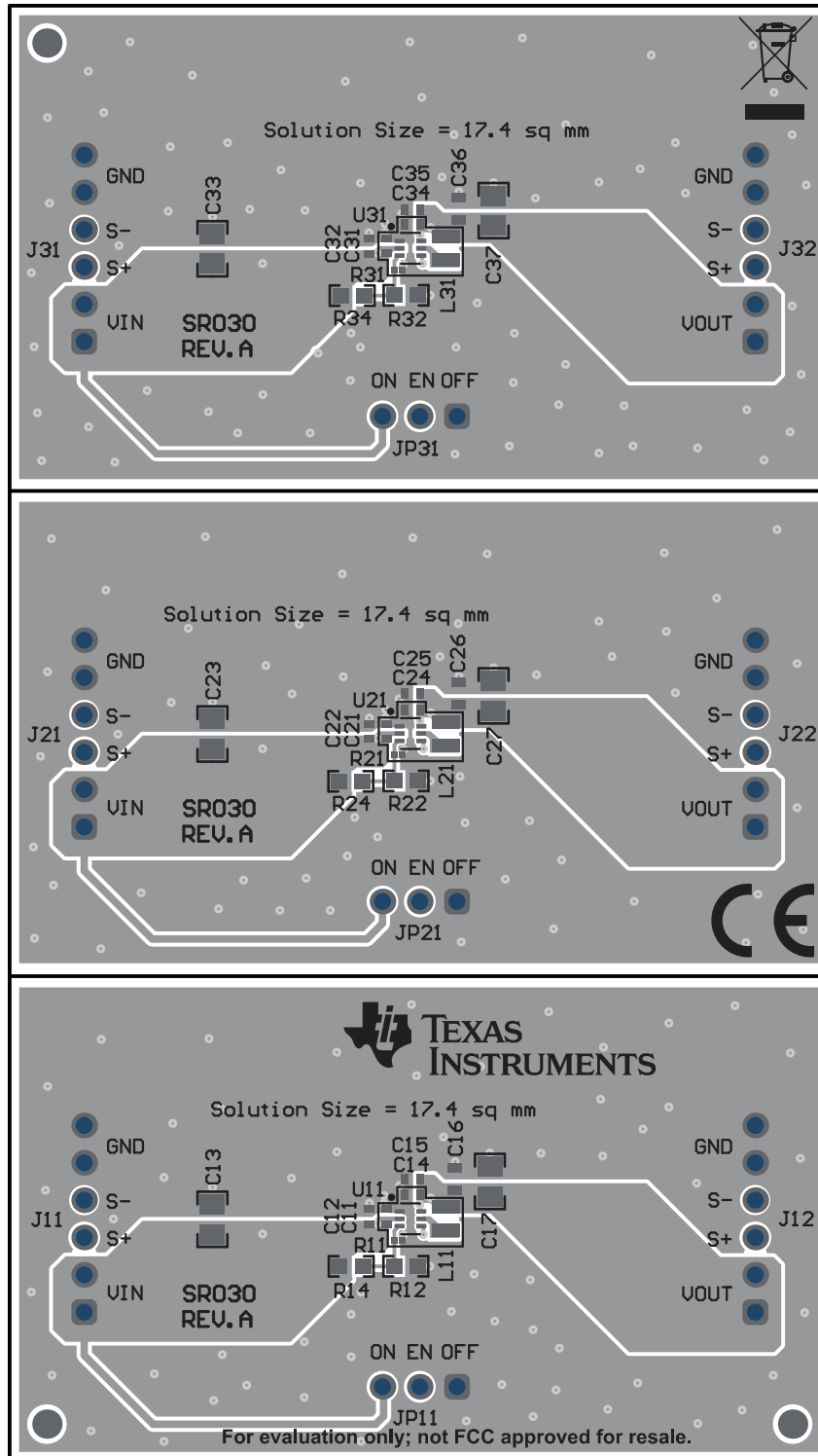
Figure 4-4. Top Assembly
