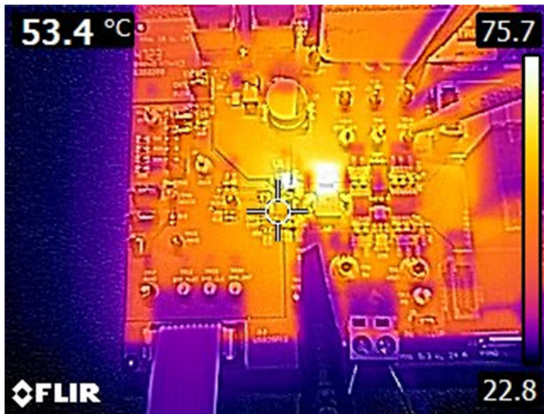
Figure 4-23. Thermal Characteristics, 800kHz FCCM, Internal LDO, 20A Load, No Airflow, Soak 10 Minutes
