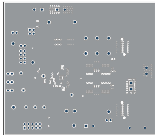
Figure 5-5. TPS544B27EVM Layer 2
