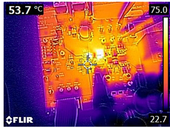
Figure 4-28. Thermal Characteristics, 1.2MHz, FCCM, External 5V Bias, 20A Load, No Airflow, Soak 10 Minutes
