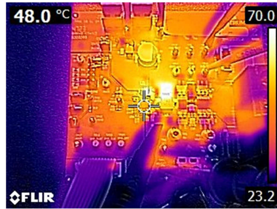
Figure 4-22. Thermal Characteristics, 600kHz FCCM, External 5V Bias, 20A Load, No Airflow, Soak 10 Minutes
