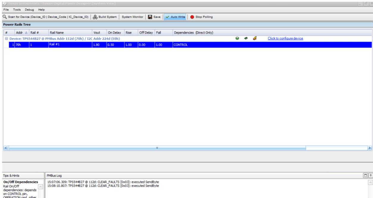
Figure 3-1. PMBus GUI System View
