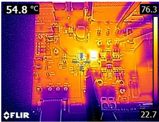
Figure 4-25. Thermal Characteristics, 1MHz FCCM, Internal LDO, 20A Load, No Airflow, Soak 10 Minutes
