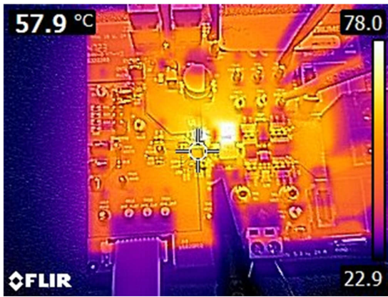
Figure 4-27. Thermal Characteristics, 1.2MHz, FCCM, Internal LDO, 20A Load, No Airflow, Soak 10 Minutes
