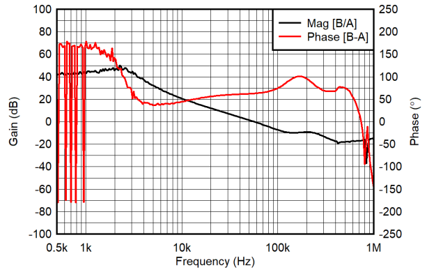
Figure 4-20. Bode Plot, FCCM, 800kHz, 20A Load
