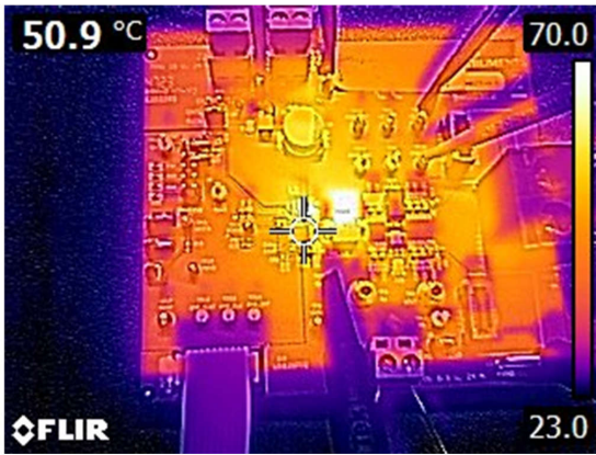
Figure 4-21. Thermal Characteristics, 600kHz FCCM, Internal LDO, 20A Load, No Airflow, Soak 10 Minutes
