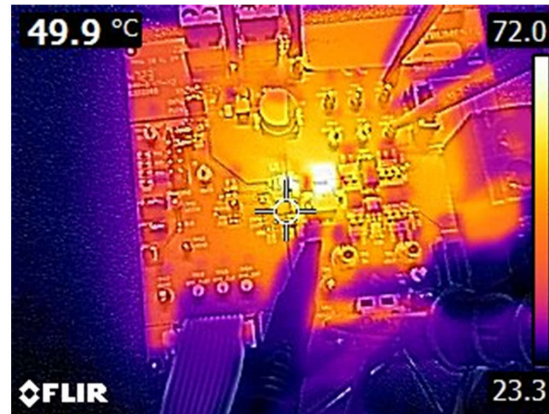
Figure 4-24. Thermal Characteristics, 800kHz FCCM, External 5V Bias, 20A Load, No Airflow, Soak 10 Minutes
