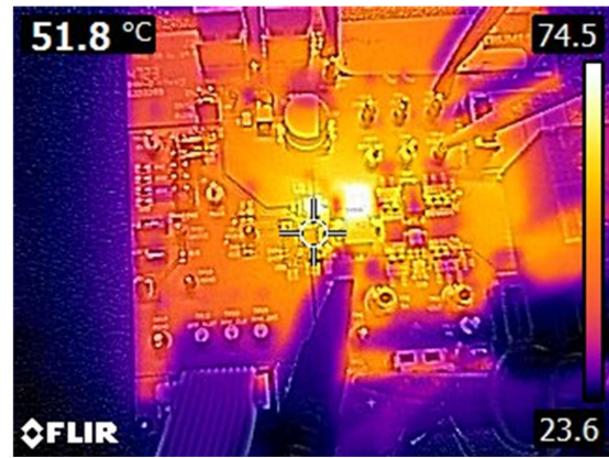
Figure 4-26. Thermal Characteristics, 1MHz FCCM, External 5V Bias, 20A Load, No Airflow, Soak 10 Minutes
