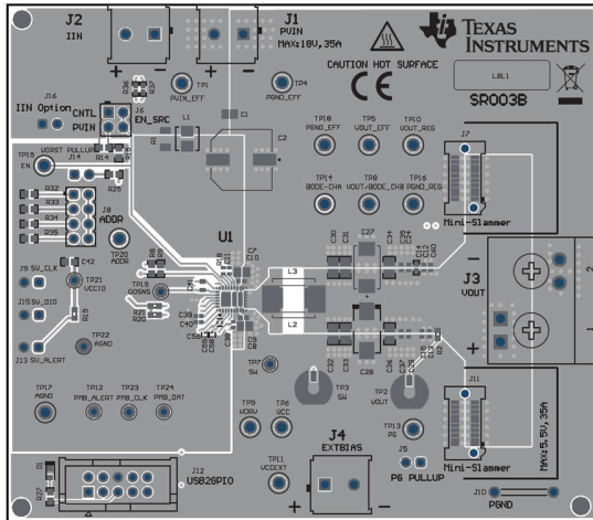
Figure 5-2. TPS544B27EVM Top Composite View
