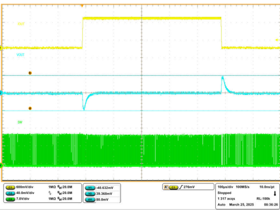
Figure 4-19. Load Transient, FCCM, 0A to 10A Load Step, 5A/us
