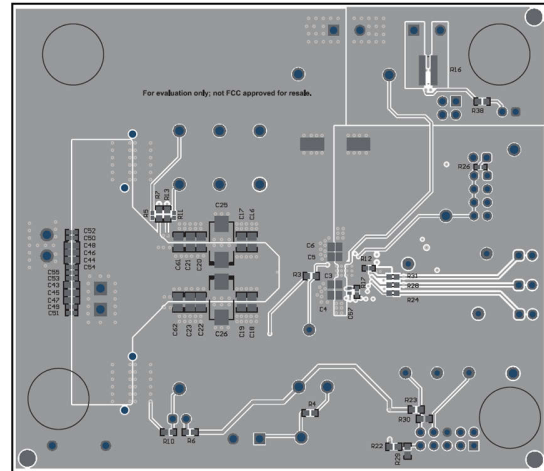
Figure 5-3. TPS544B27EVM Bottom Composite View
