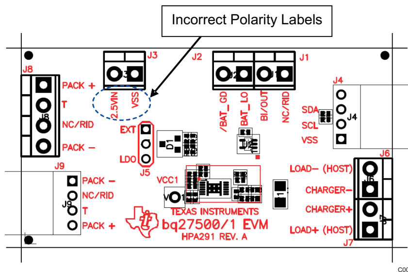
Figure 1. HPA291 Rev. A with incorrect silkscreen labels
